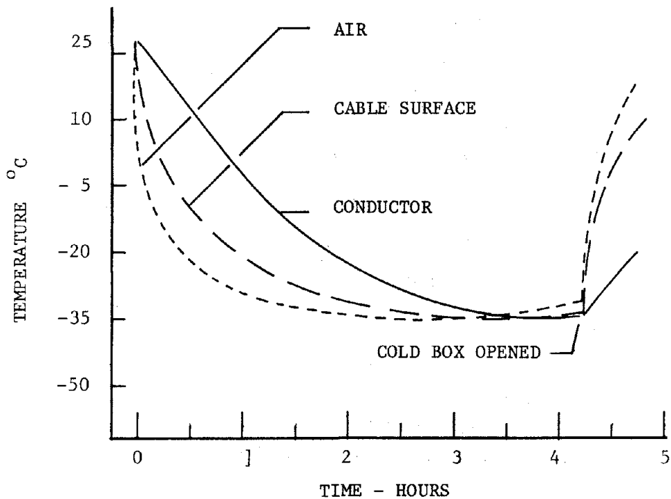
Figure 8. Cable Cooling Curves Leveling near -35^{\circ}\text{C} .
