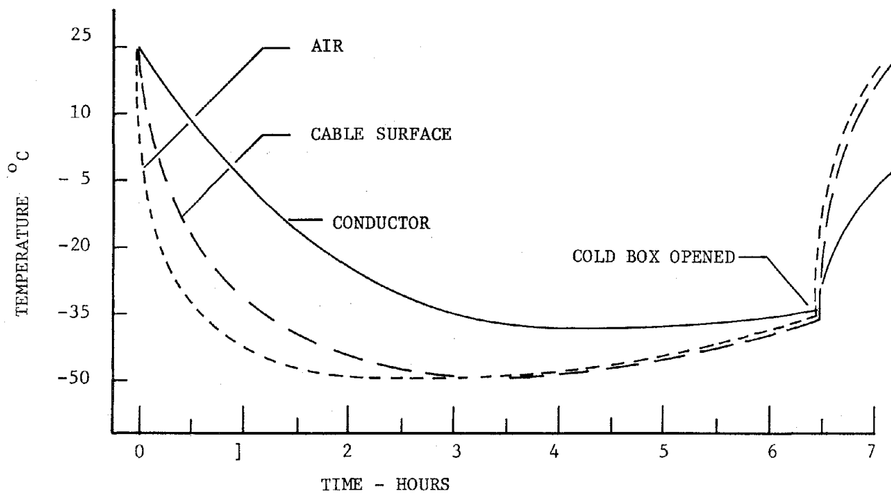
Figure 9. Cable Cooling Curves Showing Temperature Overshoot to -50^{\circ}\text{C} .
