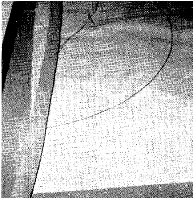
Figure 11. Cable Jacket that Withstood the Cold Bend Test.
