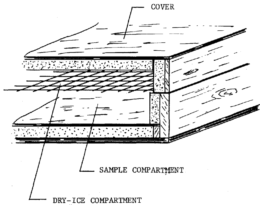
Figure 7. Cold Box Construction
