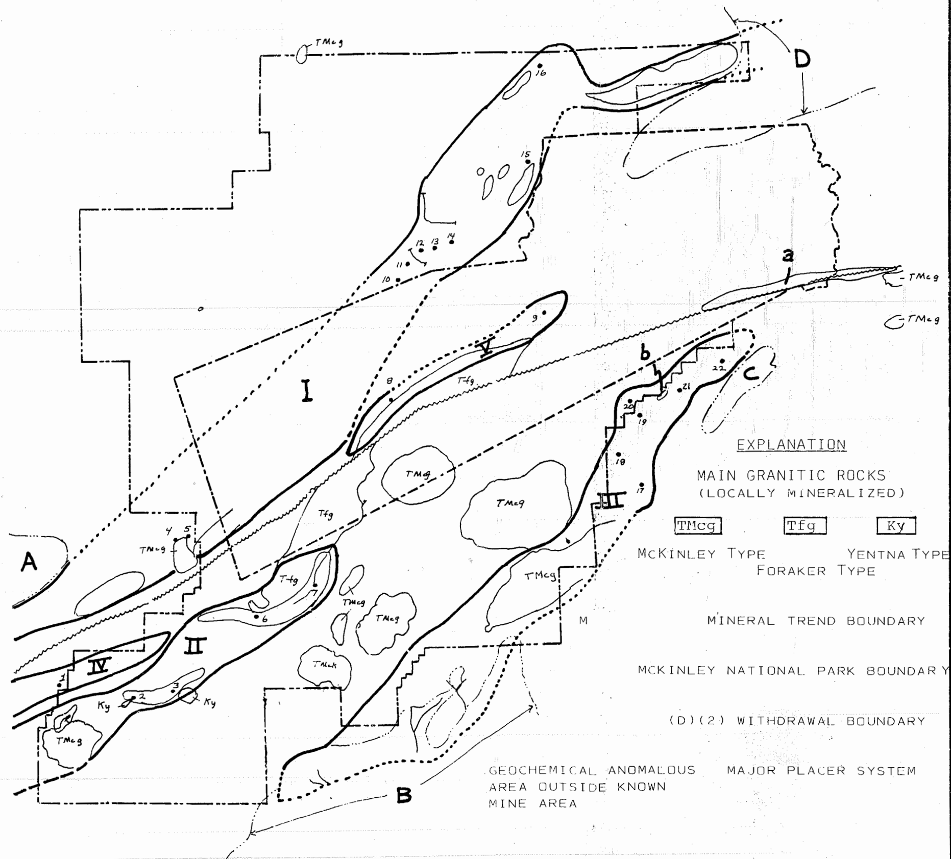
FIGURE 6.1 SUMMARY OF ECONOMIC GEOLOGY OF THE MT. MCKINLEY REGION
