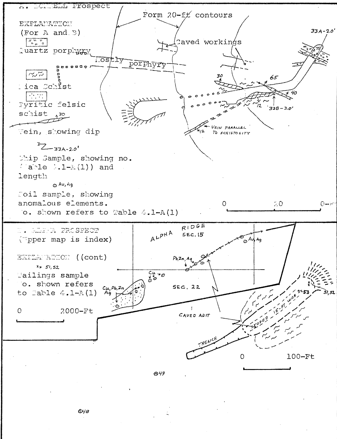
FIGURE 4.1-A(1)- 2--SKETCH MAPS OF THE BONNELL (A) and ALPHA (B) PROSPECTS
