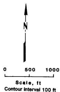
Figure 9 - Geologic and sample location map of the northwestern Bokan Mountain area.
