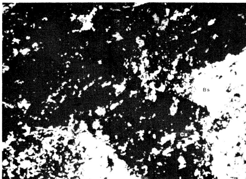
Figure 23 - Radioactive dikes at Bokan Mountain generally contain fine to medium grain Cb-REE-Zr minerals suspended in a matrix of quartz and Na-feldspar.
