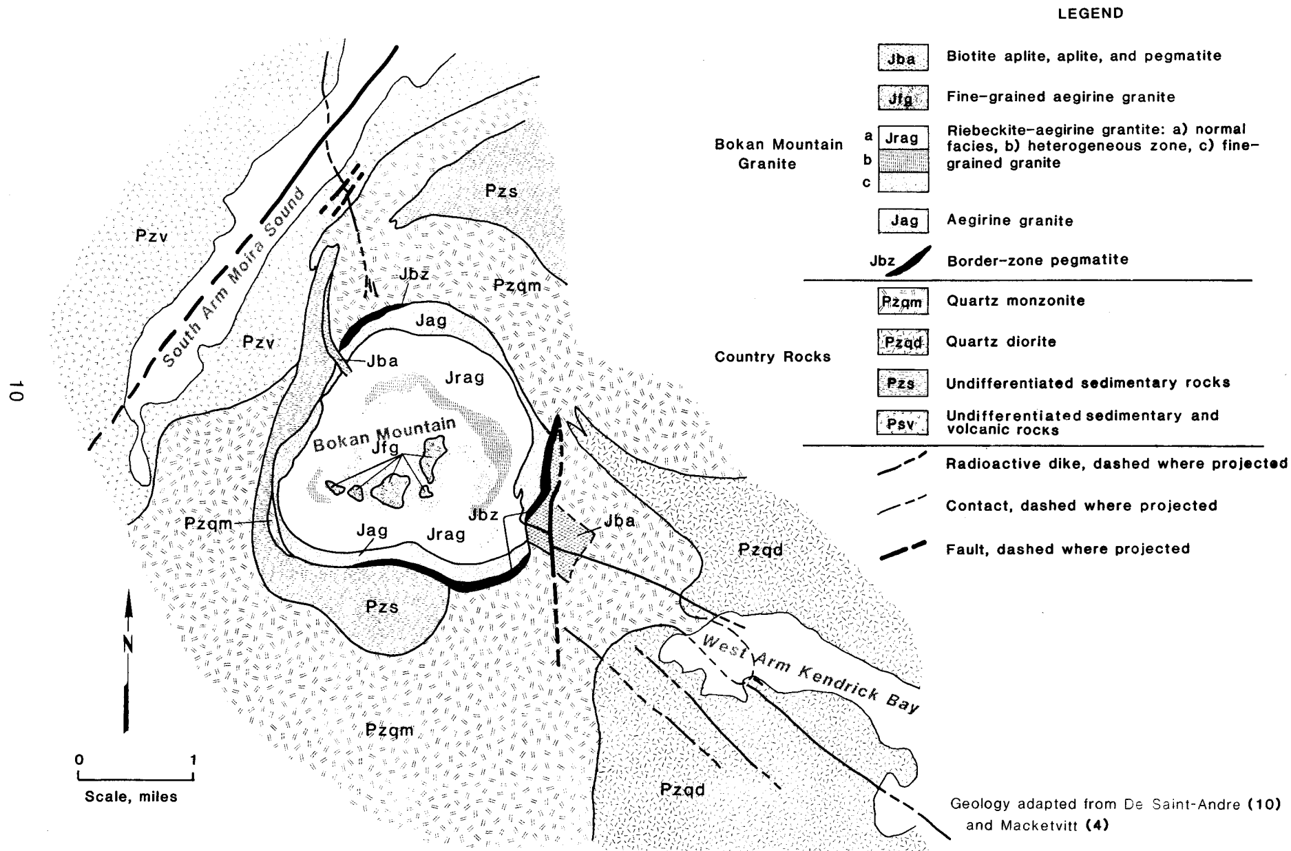
Figure 3 - Geology of the Bokan Mountain granite.
