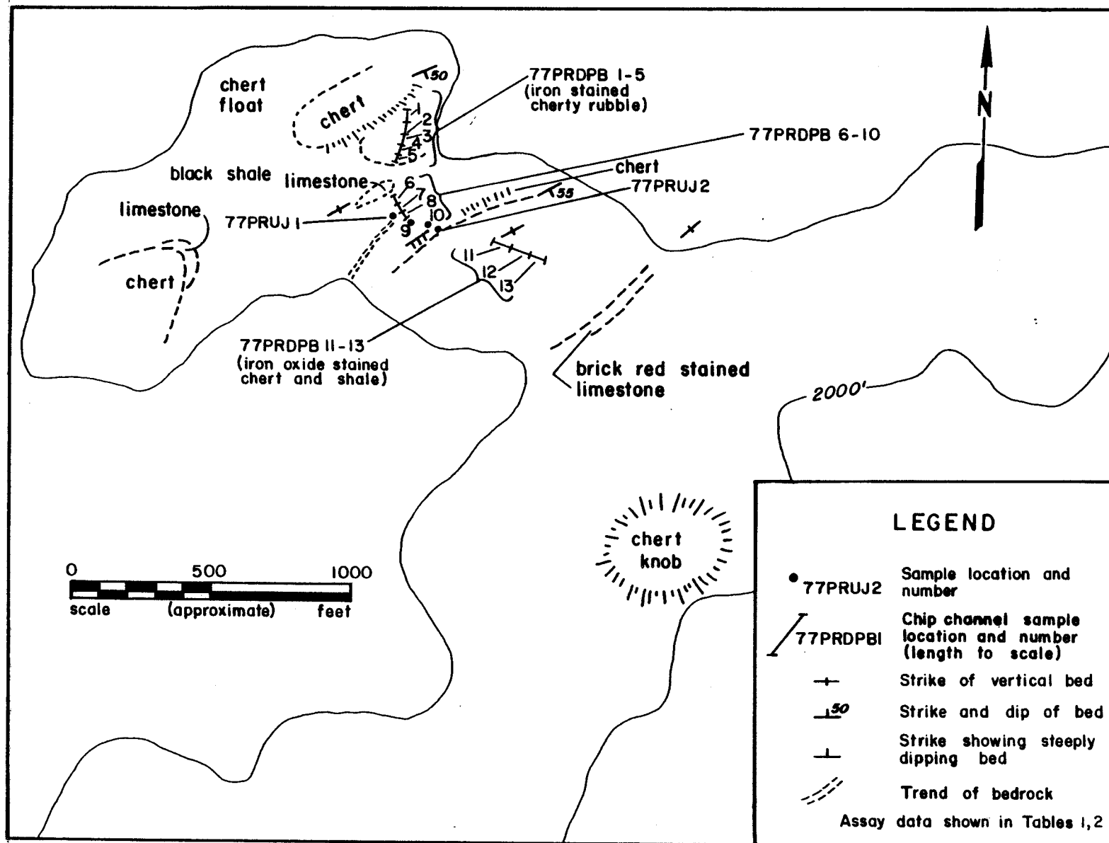
FIGURE 5.- Bedrock sample locations west of Kagvik Creek, Misheguk Mountain quadrangle, Alaska
