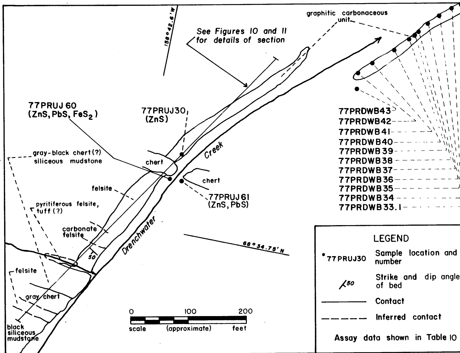
FIGURE 9.- Generalized geology, mineral occurrences and sample locations--Drenchwater Creek, Howard Pass quadrangle, Alaska
