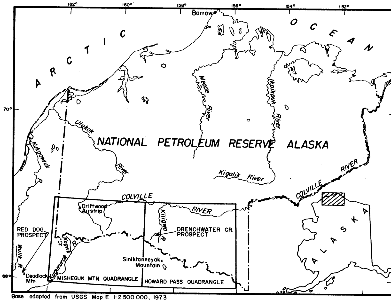
FIGURE 1.- Index map of Northern Alaska showing location of 1977 field studies related to the National Petroleum Reserve-Alaska
