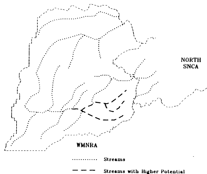
Figure 4b. Location of Streams Tested for Gold Placer Potential
