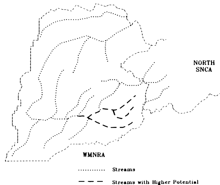
Figure ES-2b. Location of Streams Tested for Gold Placer Potential
