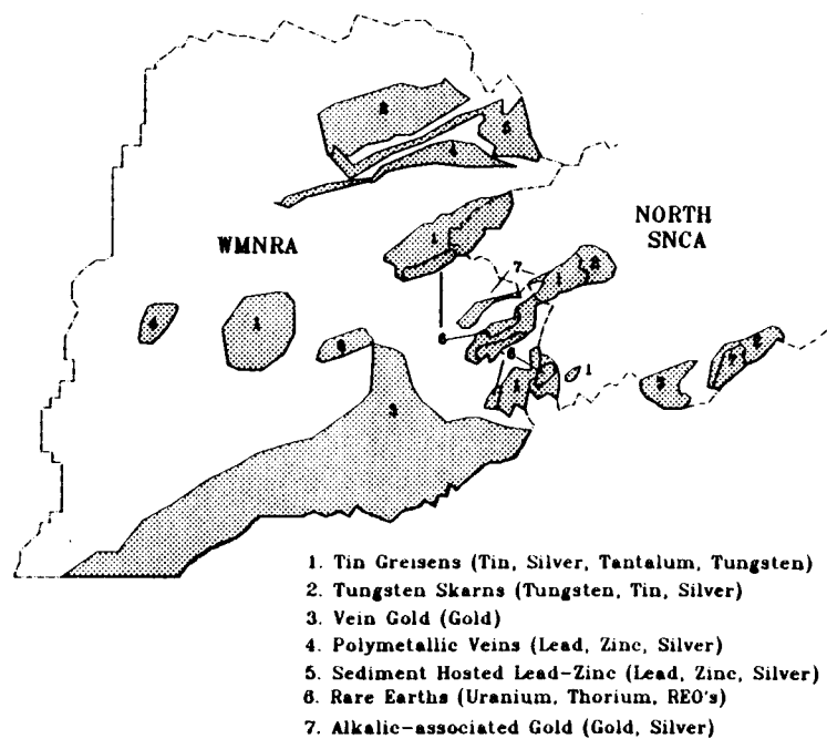
Figure 4a. Location of Lands Favorable for Various Types of Non-Placer Mineral Deposits
