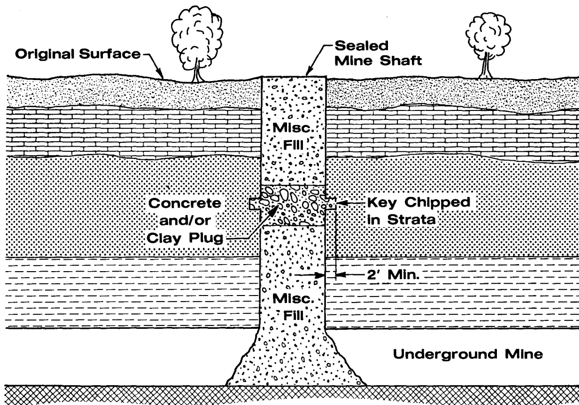
FIGURE 23. - Hydraulic shaft seal with keyed plug.
