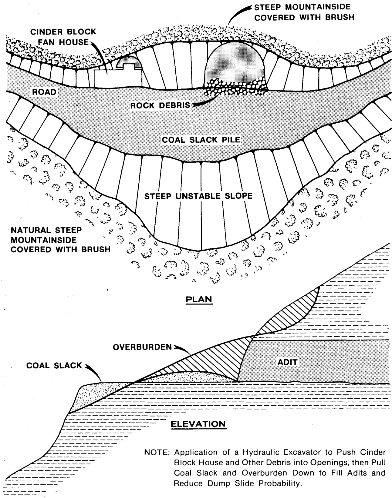
FIGURE 3. - Suggested earth backfill for steep slope adit.
