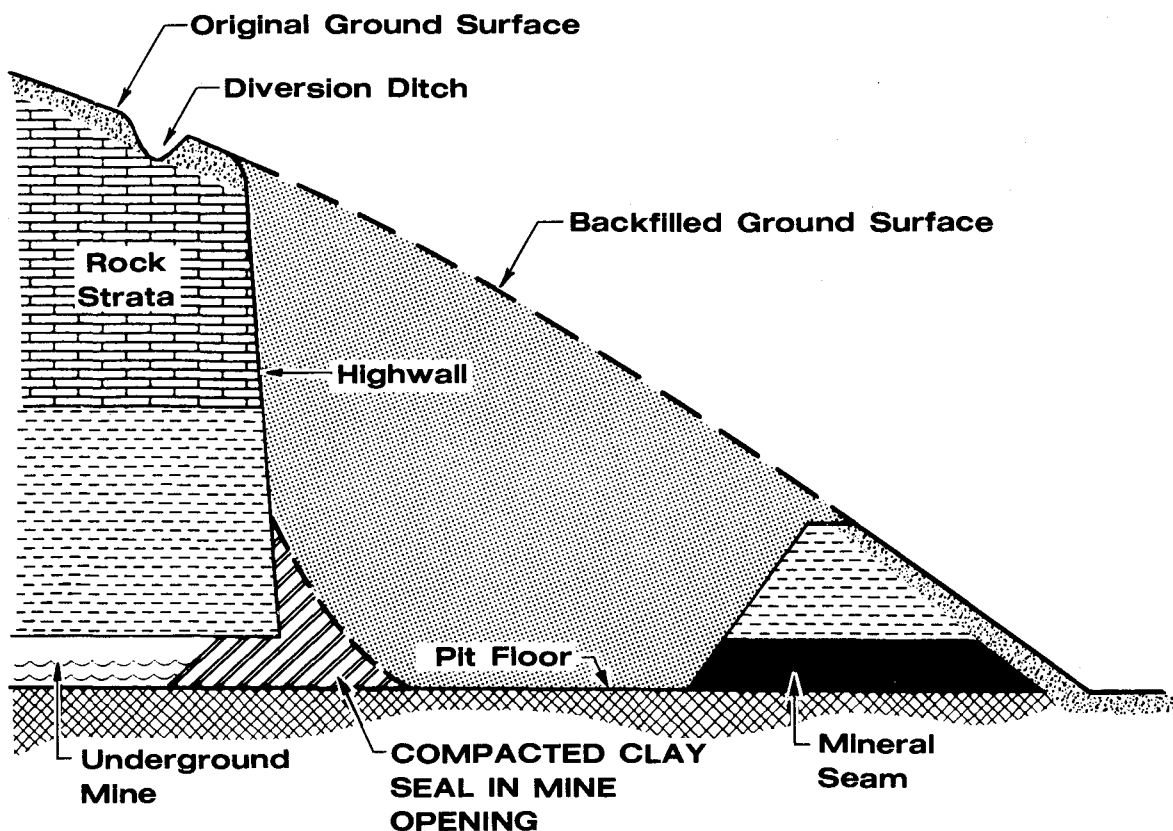
FIGURE 20. - Cross section of typical clay seal.
