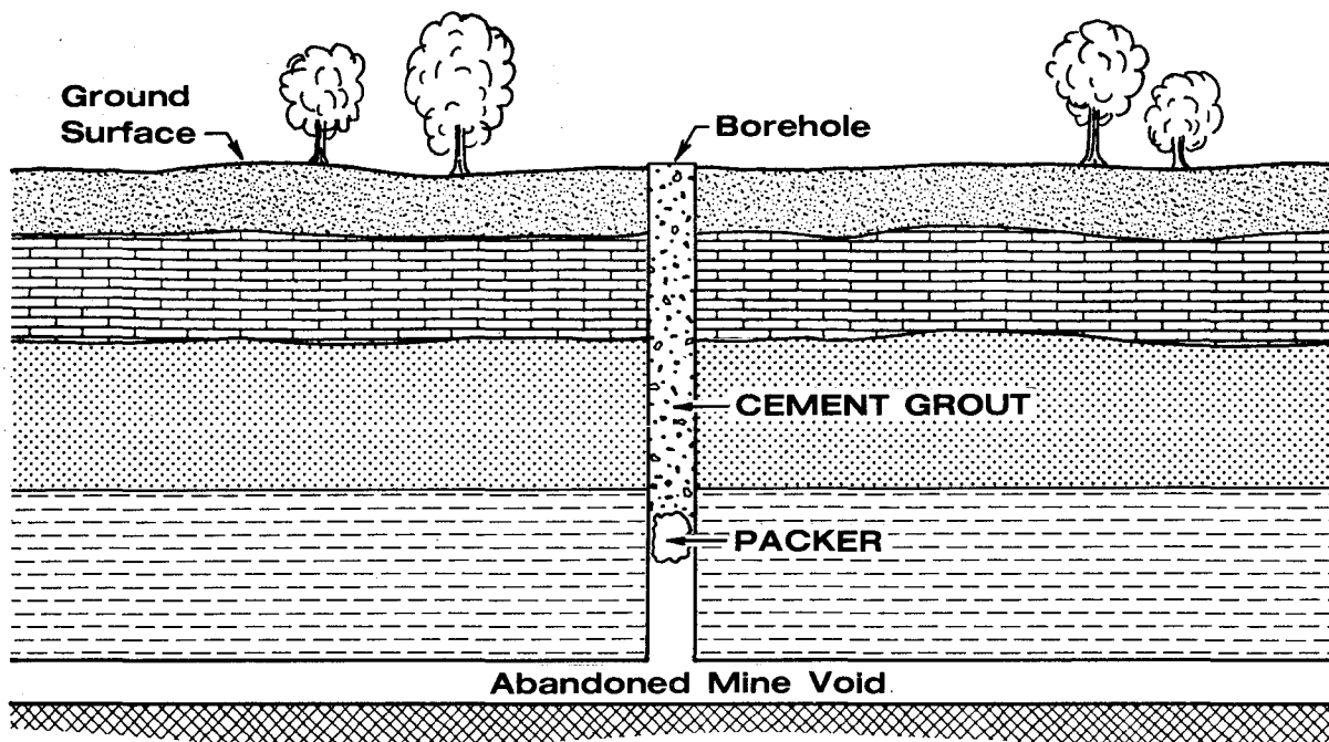
FIGURE 25. - Typical method of borehole sealing with cement grout.
