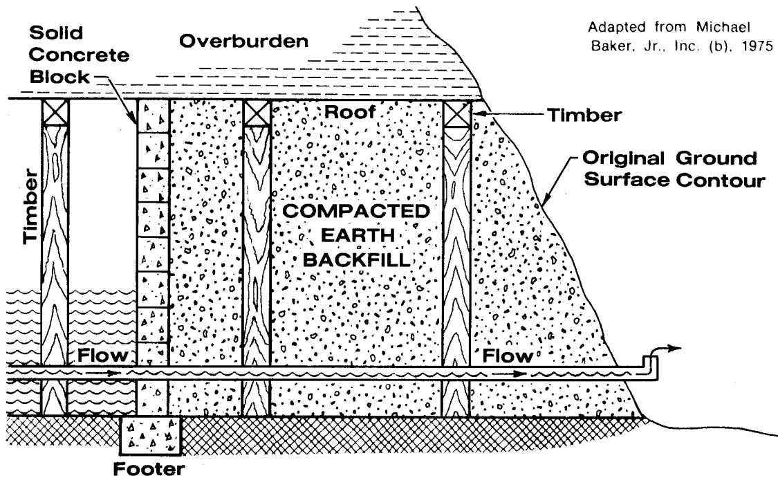
FIGURE 9. - Earth backfill air seal.
