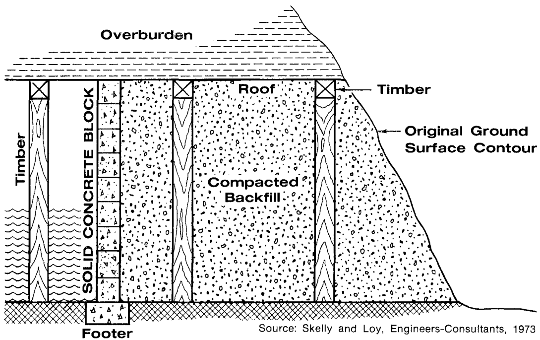
FIGURE 15. - Backfilled masonry block seal.
