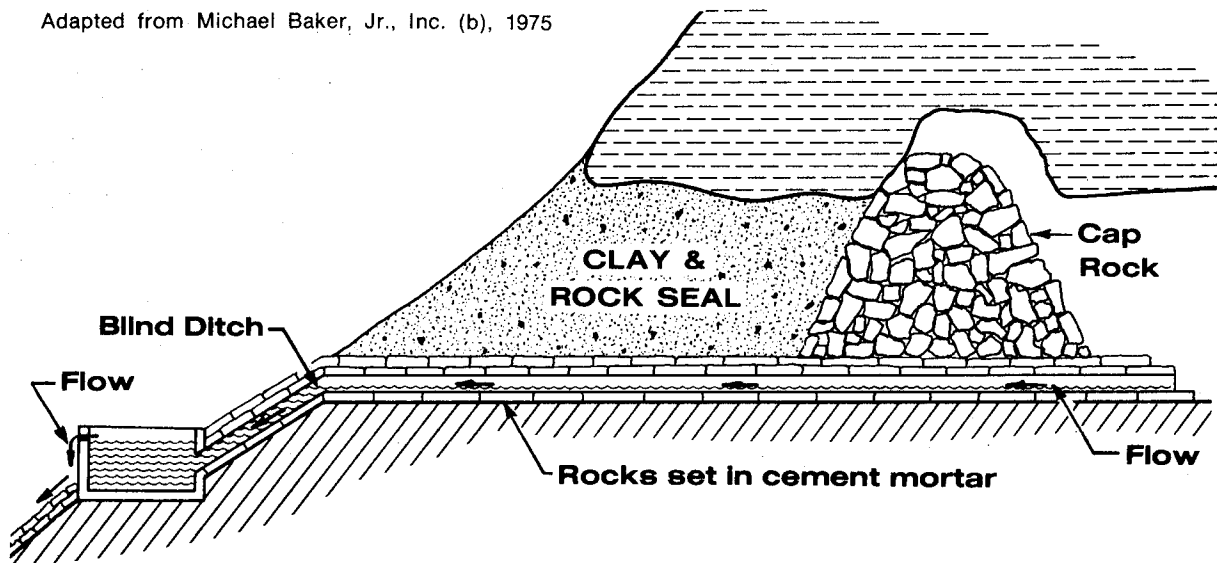
FIGURE 10. - Clay and rock water-trap air seal for caved pit mouth.
