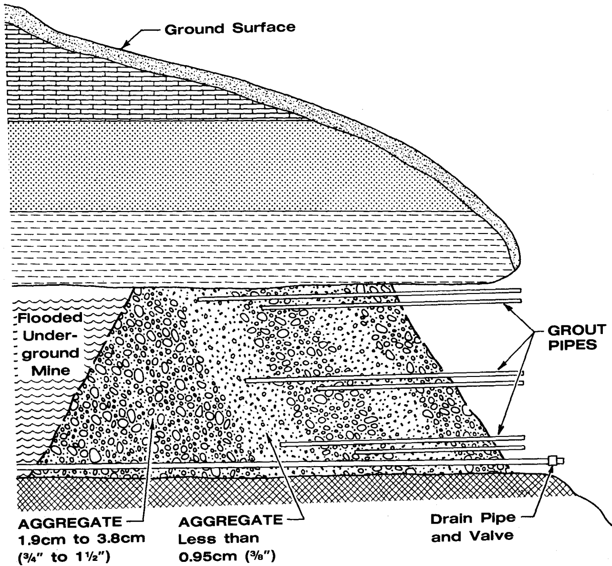
FIGURE 16. - Grouted aggregate seal for accessible opening.
