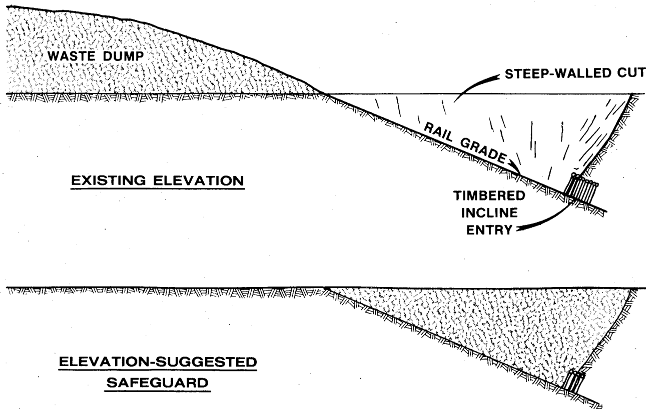
FIGURE 2. - Earth backfill for unstable incline.
