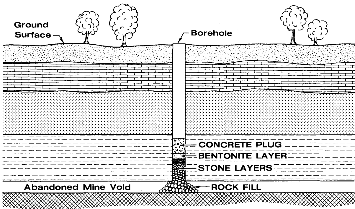
FIGURE 24. - Hydraulic borehole seal with bentonite and concrete.
