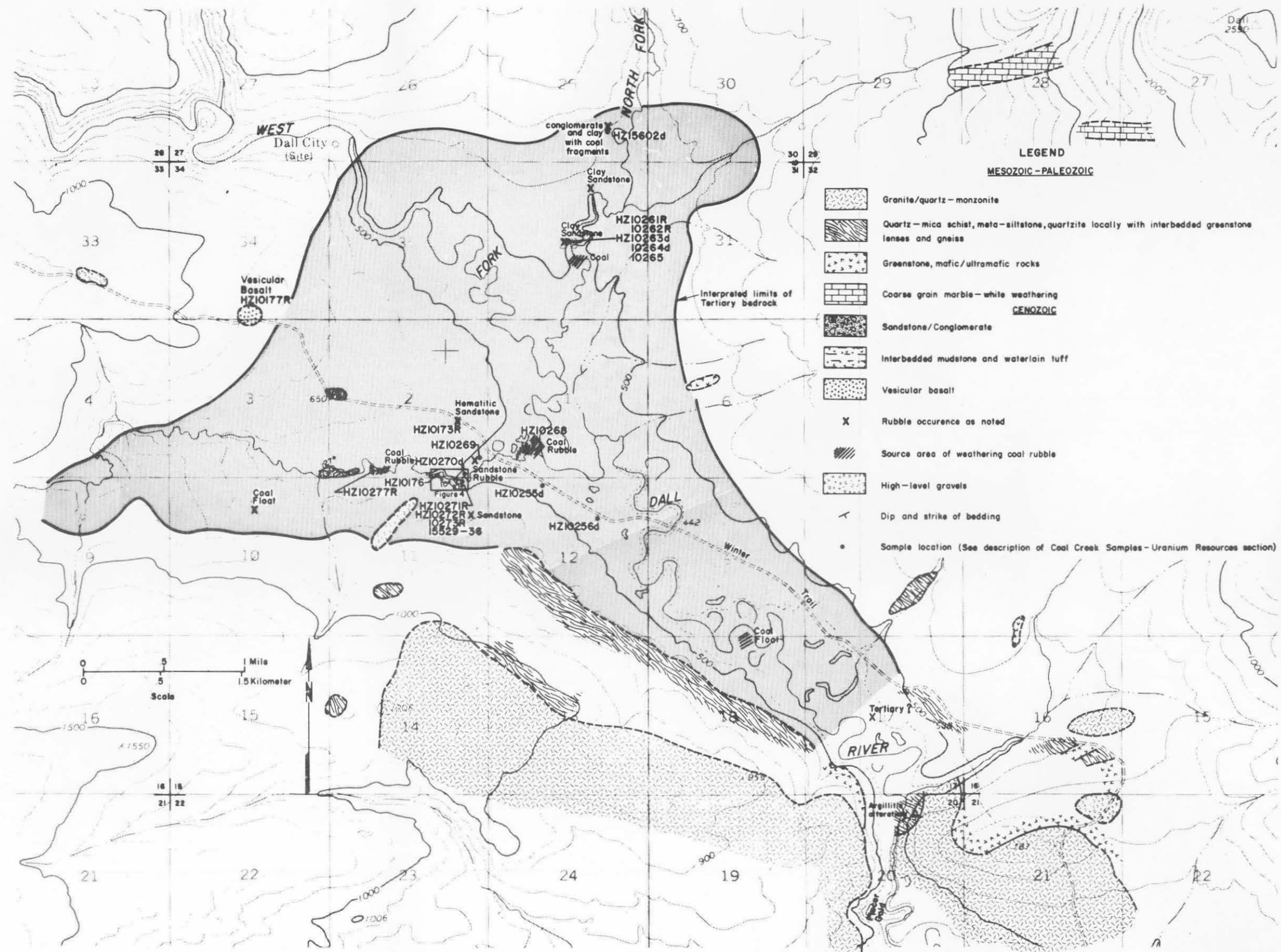
FIGURE 5 - UPPER DALL RIVER REGION
