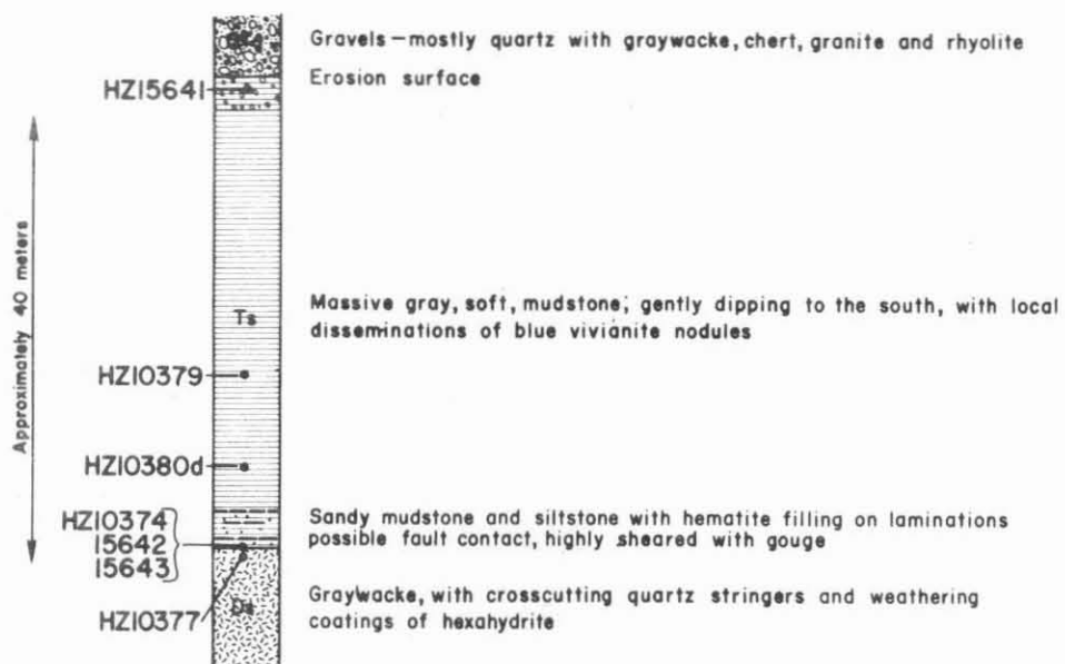
Figure 9 : Composite Section and Sample Locations of Hodzana Locality 2
