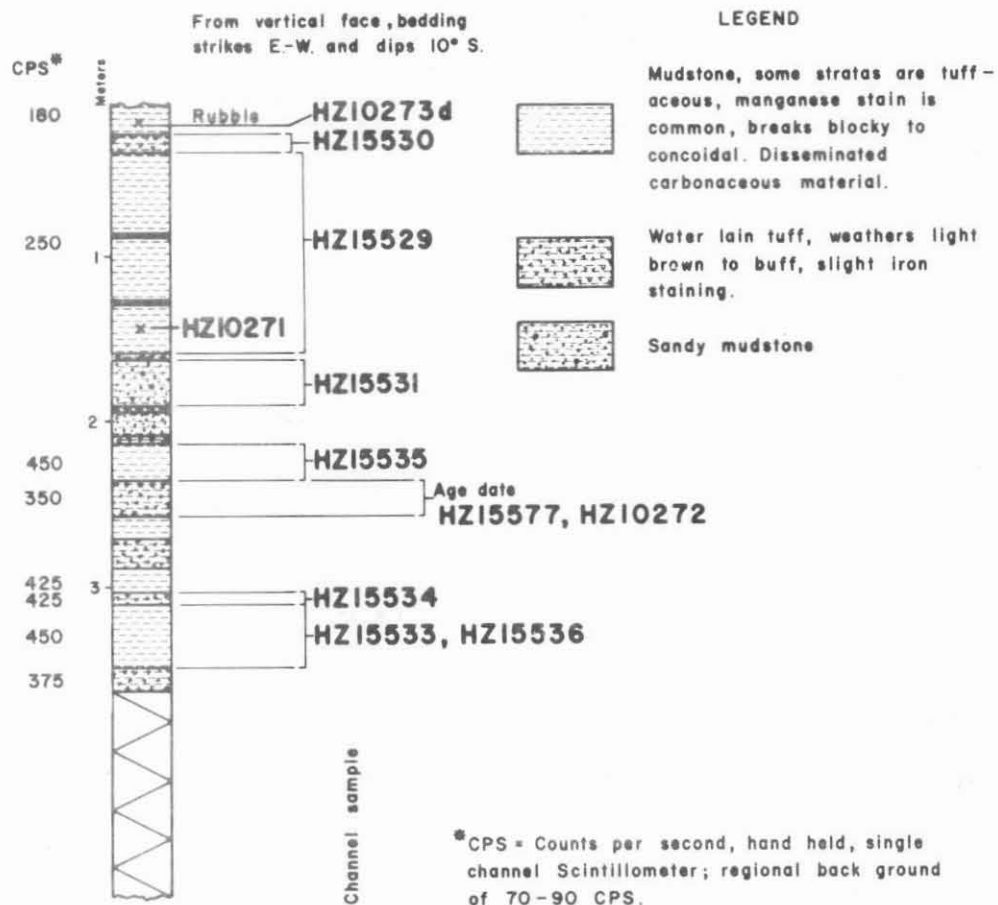
Figure 7.- Profile of water lain tuffs - Coal Creek
