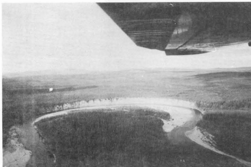
Figure 4. Mudbank: Tertiary bedrock at "Mudband" on the Hodzana River
