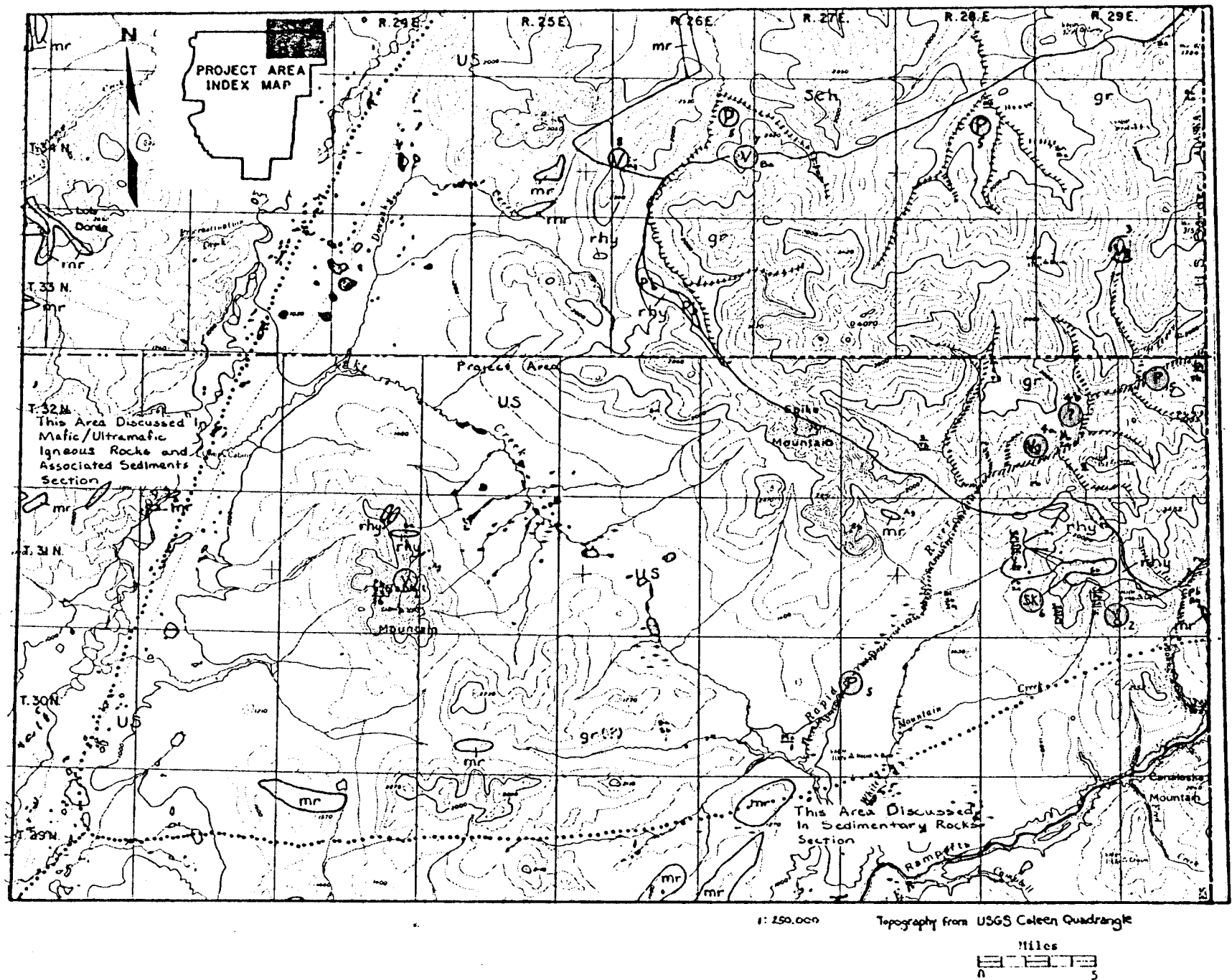
FIGURE 8.- Mineral occurrences and anomalies--granitic terrane
