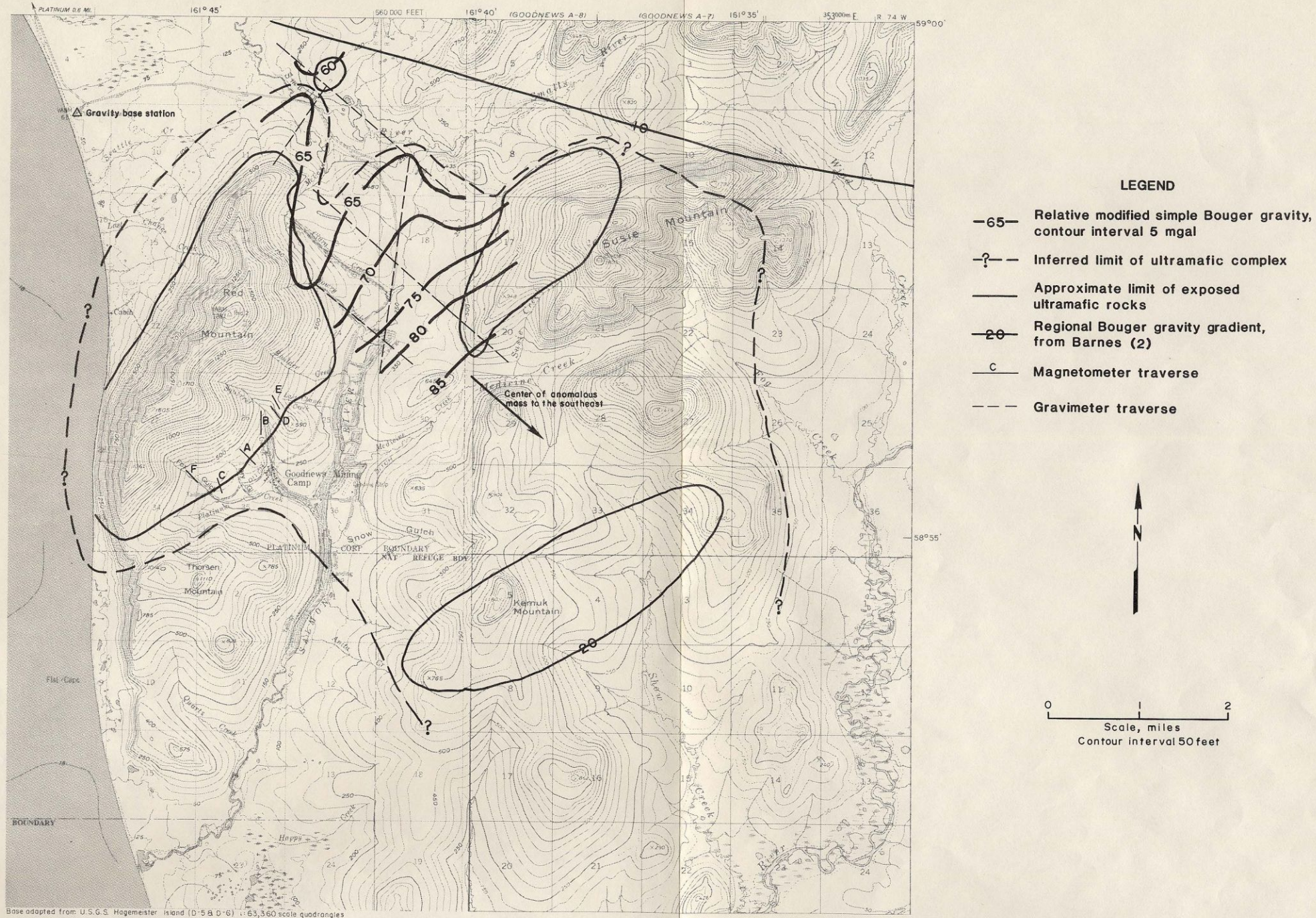
FIGURE 20. -- Location of geophysical traverses and gravity contour map of the Goodnews Bay Complex
