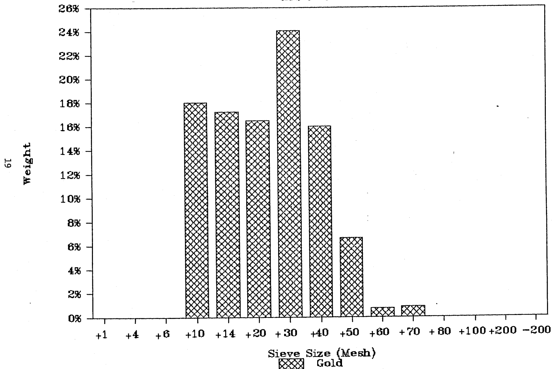
Figure 10. Histogram of Sample B-6 Eldorado Creek.
