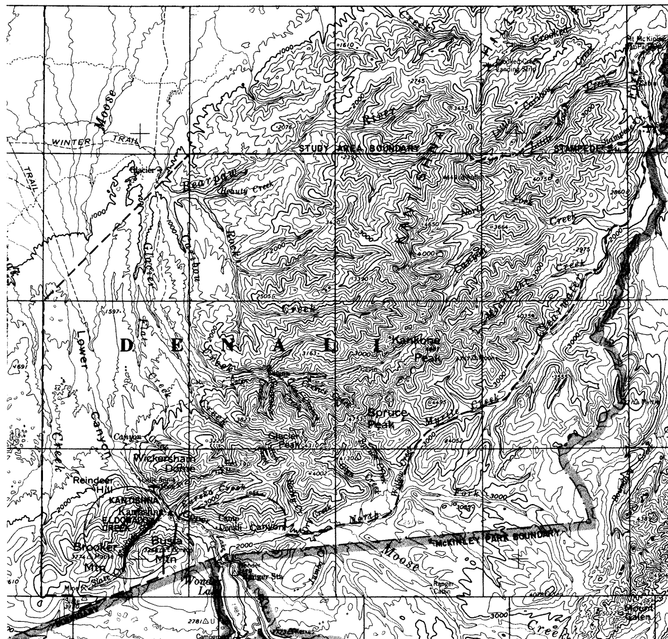
Figure K-15 Eldorado Creek location, Kantishna Hills study area
