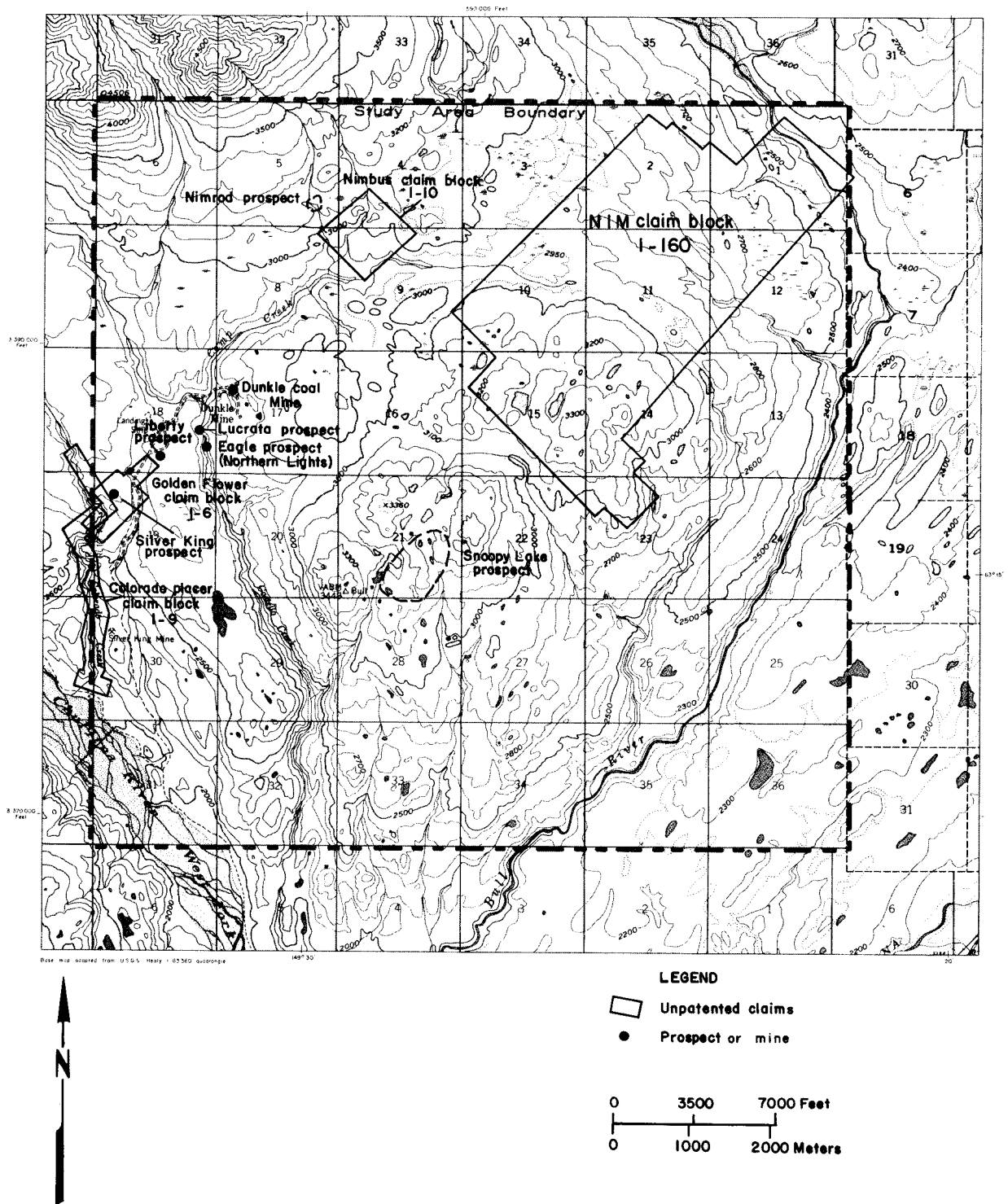
Figure D-9 Claims, Mines, and Prospects - Dunkle Mine Study Area
