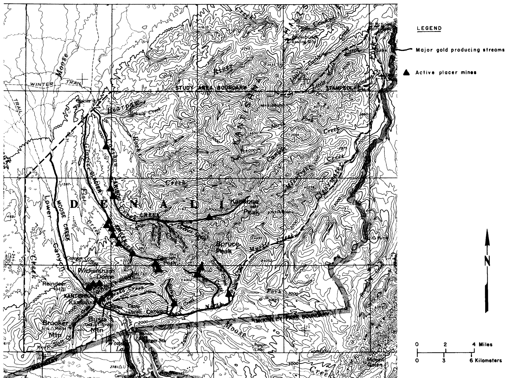
Figure K-9 Major placer gold producing streams and active 1983 placer mining operations in the Kantishna Hills study area
