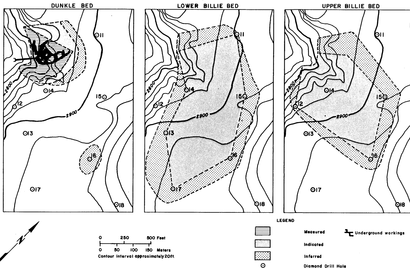
Figure No.D-8 Coal Reserves, W.E. Dunkle Mine- Dunkle Mine Study Area (from Rutledge, 1948)
