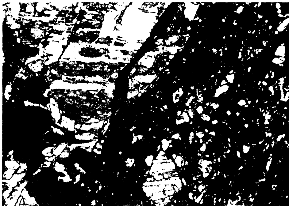
FIGURE 9. - Cataclastic texture in wehrliite. Field of view = 1.1 x 1.7 mm. Sample KW19877.
