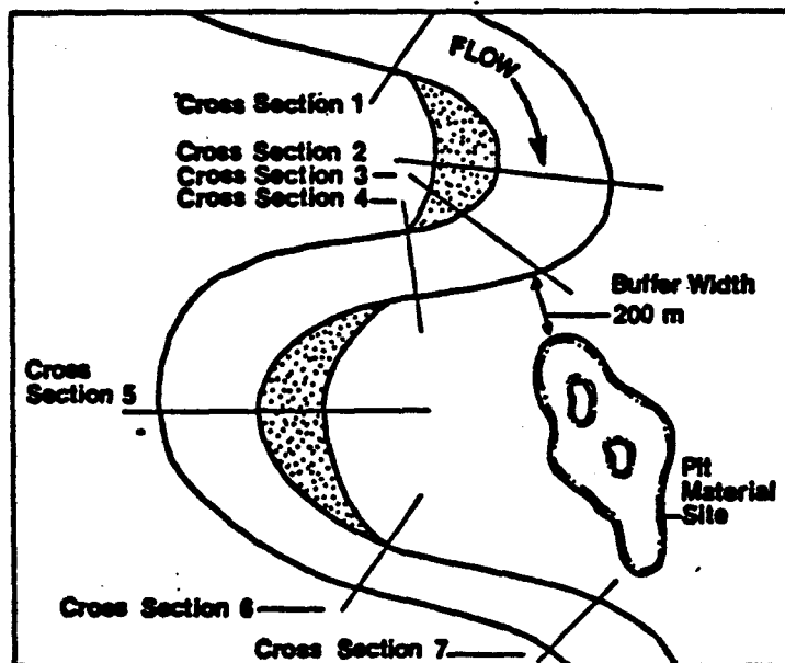
Figure 16. Schematic of an example of buffer height design (Woodward Clyde Consultant, 1980)
