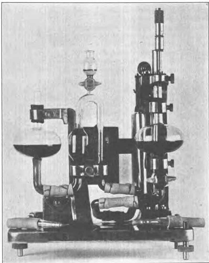
FIGURE 2.—Wahlen gauge or Illinois differential micromanometer
