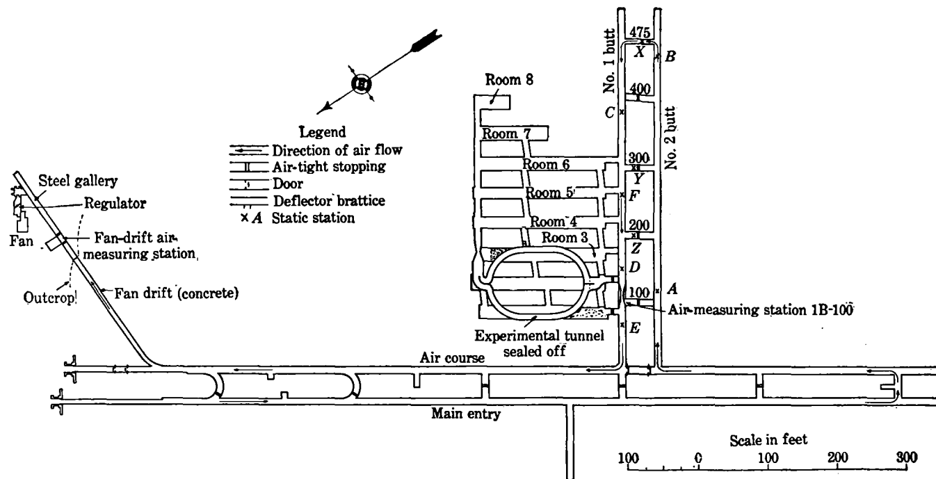
FIGURE 1.—Plan of experimental mine, showing location of test section and air-measuring and static stations
