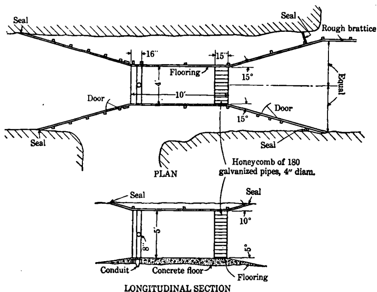
FIGURE 4.—Air-measuring station at 1B-100
