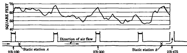
FIGURE 21.—Test section A-B with corresponding area graph
