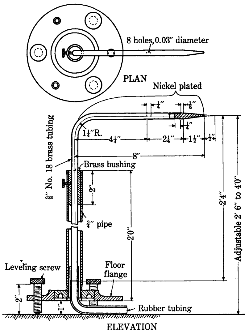
FIGURE 17.—Static-pressure tube and holder
