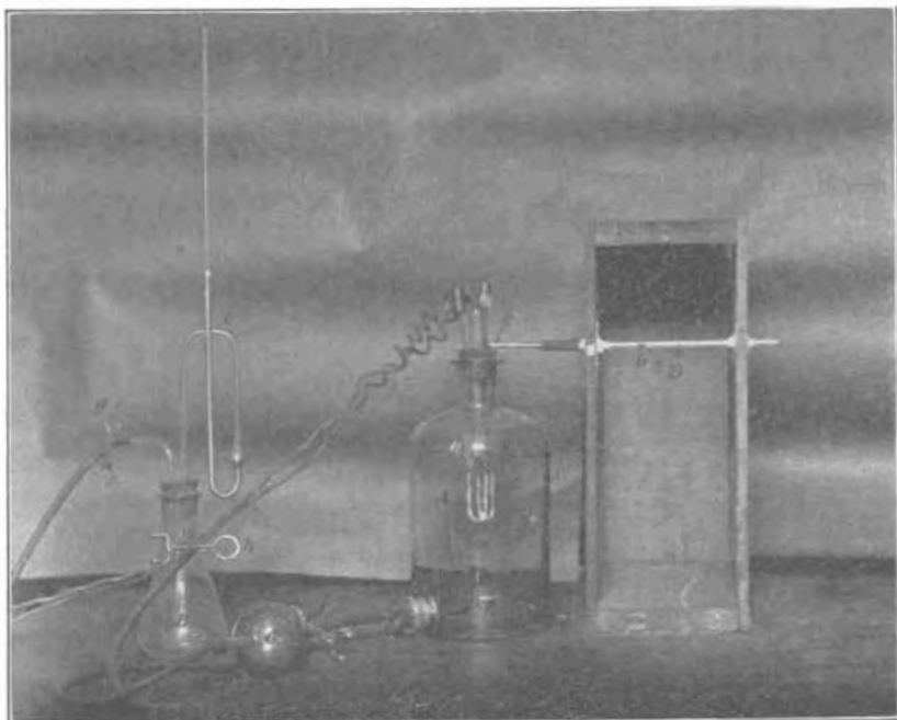
A. COAL-DUST IGNITION APPARATUS USED AT PITTSBURG.
