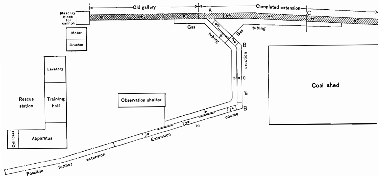
FIGURE 19.—Plan of Frameries gallery, showing proposed extension.
