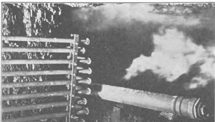
4. RADIATOR AND STEAM PIPE IN USE, MONONGAH NO. 8 MINE.
