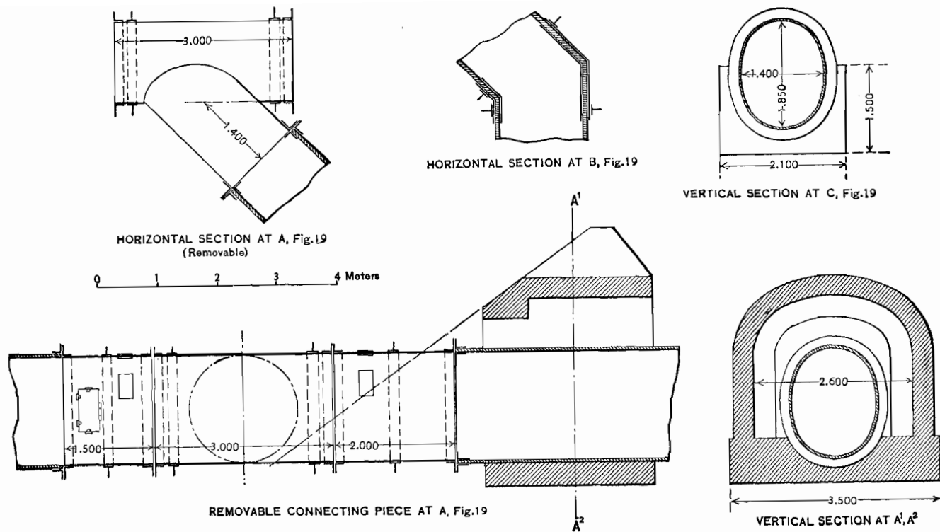
FIGURE 20.—Constructional details of extension to Frameries gallery.
