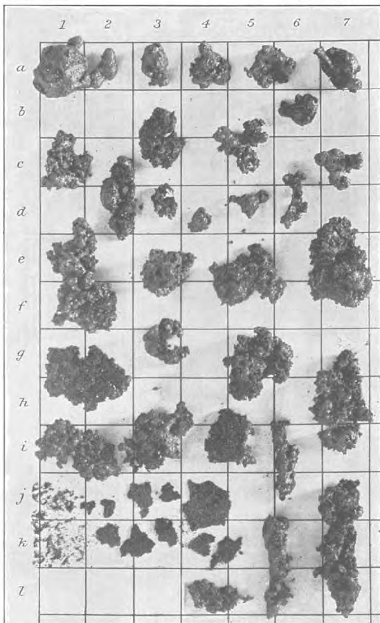
COKE DUST FROM PITTSBURG GALLERY DENSITY TEST WITH 200-MESH DUST.
