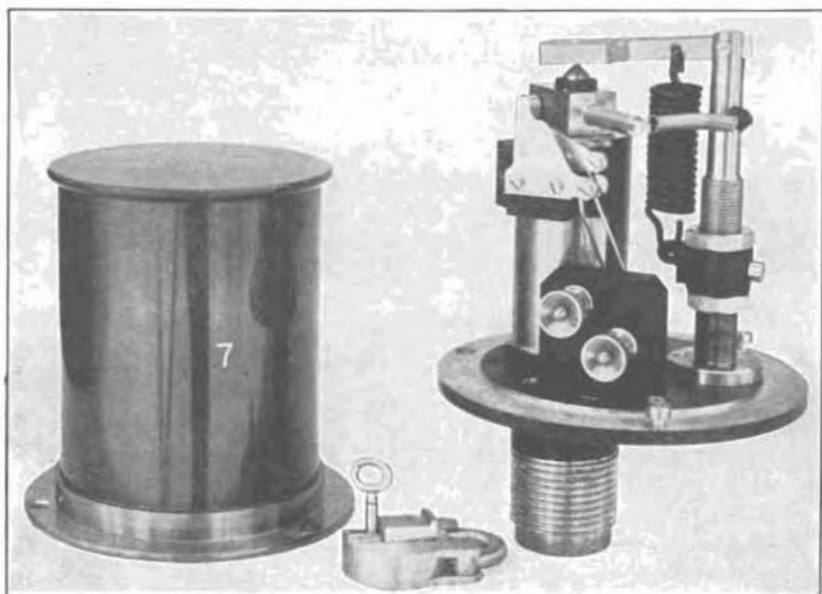
B. CONTACT BREAKER, ALTOFTS EXPERIMENTAL GALLERY; AFTER FIRING.
