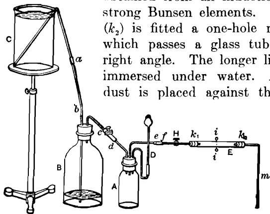
FIGURE 9.—Coal-dust ignition apparatus of Holtzwart and Meyer.
