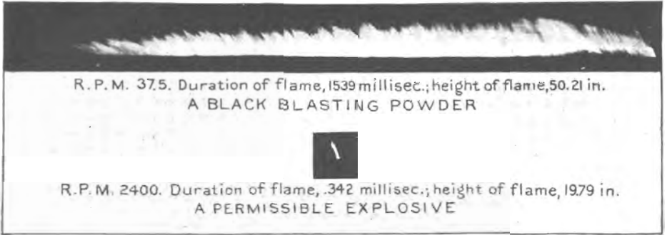
A. FLAMES FROM EXPLOSION OF EQUAL WEIGHTS OF BLACK BLASTING POWDER AND OF A PERMISSIBLE EXPLOSIVE.
