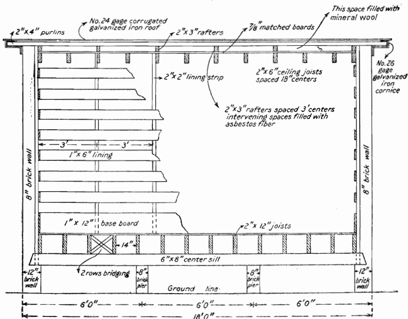
FIGURE 12.—Sections of magazine: A, section at line CD in fig. 11, B; B, section at line A in fig. 12, A.
