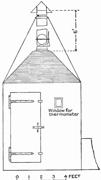
FIGURE 1.—Thaw house for frozen explosives: elevation.
