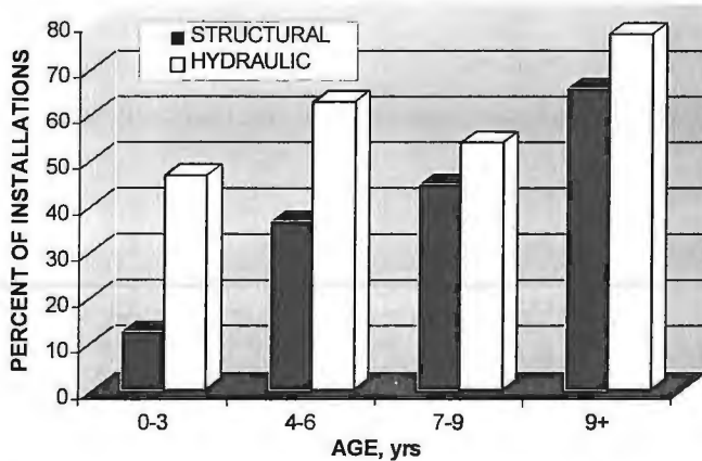
Figure 6.—Distribution of structural and hydraulic failures on shields as a function of age.
