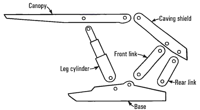
Figure 1.—Diagram of shield components .
