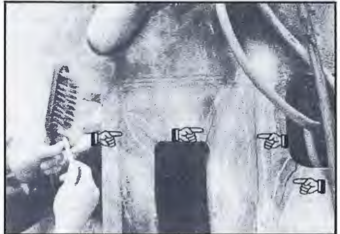
Figure 16.—Failure due to stress concentrations in cutout sections of caving shield.
