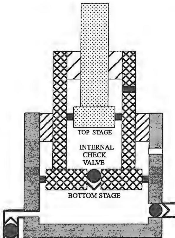
Figure 22.—Two-stage leg cylinder design used in shield supports.
