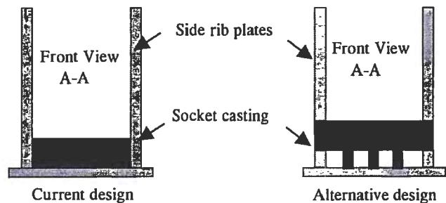
Figure 20.—Conventional and alternative leg cylinder casting design.
