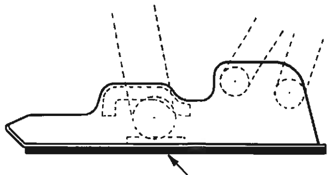
Figure 12.—Modification made to strengthen base in order to prevent leg socket casting failures.
