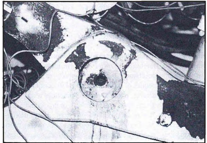
Figure 10.—Reduction in lemniscate pin contact area for worn joint.
