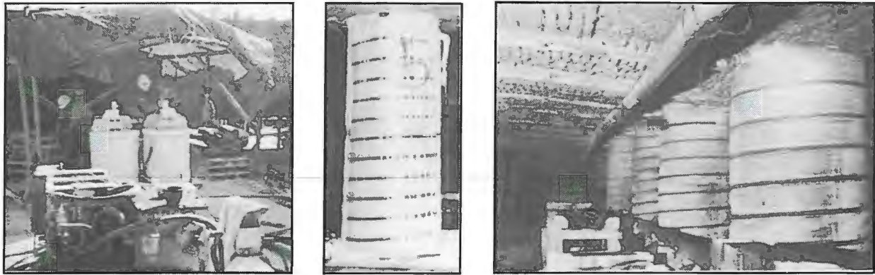
Figure 12.—A, Surface pumping station for Pumpable Crib; B, Pumpable Crib; and C, underground installation of Pumpable Crib in longwall tailgate.
