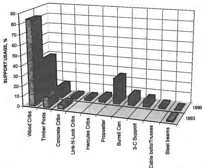
Figure 3.—Comparison of support technologies used in 1993 and 1996.
