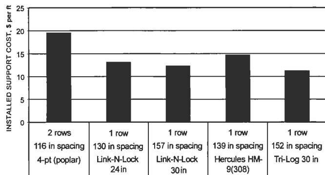
Figure 11.—Evaluation of engineered timber support systems as a replacement for conventional wood cribbing.
