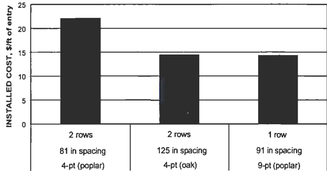
Figure 9.—Comparison of installation costs of various wood crib designs (timbers are 5×6×30 in and placed with 5-in side down).
