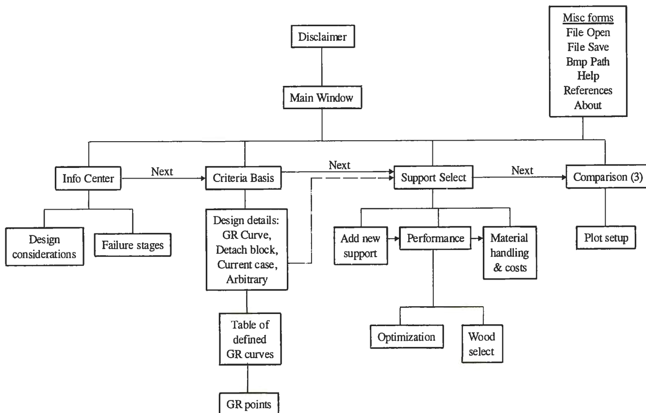
Figure 7.—Flow diagram showing program control.
