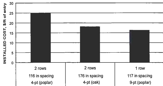
Figure 10.—Same analysis as shown in figure 9 except wide (6-in) side of timber placed down.
