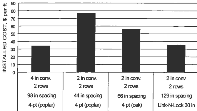
Figure 12.—Analysis of support system options when convergence requirement is reduced from 4 to 2 in.
