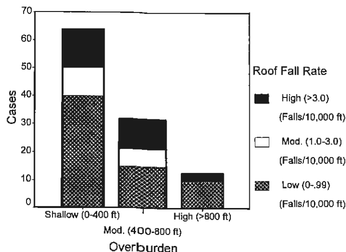
Figure 16.—Relationship between roof fall rate and overburden.
