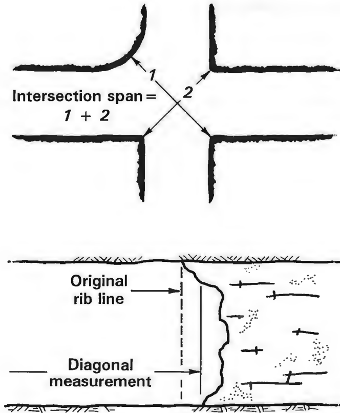
Figure 12.—Method of measuring intersection diagonals.
