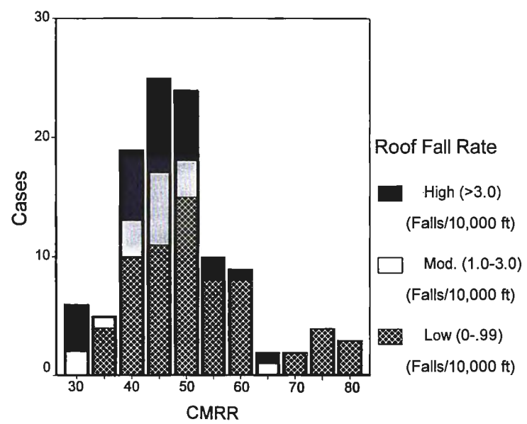
Figure 11.—Relationship between roof fall rate and CMRR.
