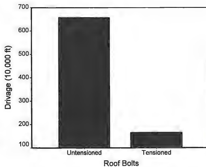
Figure 6.—Distribution of tensioned and untensioned bolts in the study.
