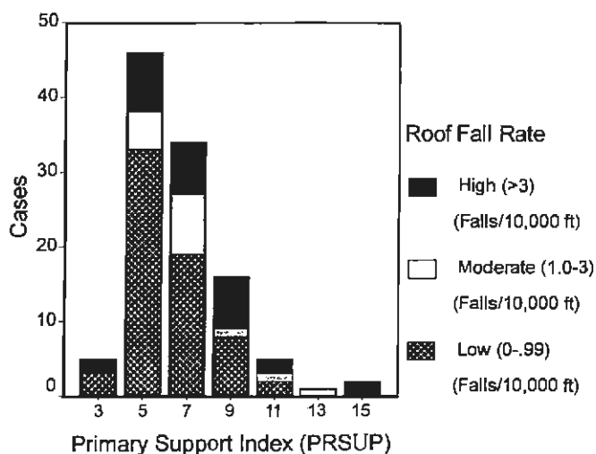
Figure 9.—Relationship between PRSUP and roof fall rate.
