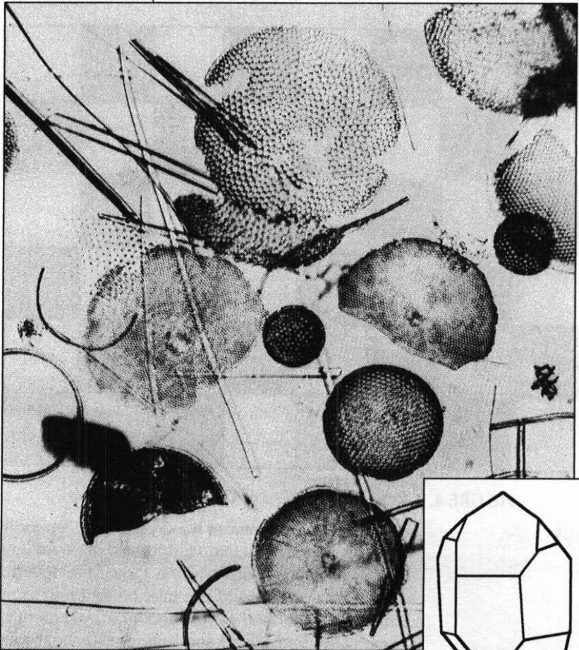
Photomicrograph of species of diatoms common in freshwater deposits. Average diameter of the fossils is about .05 mm.
