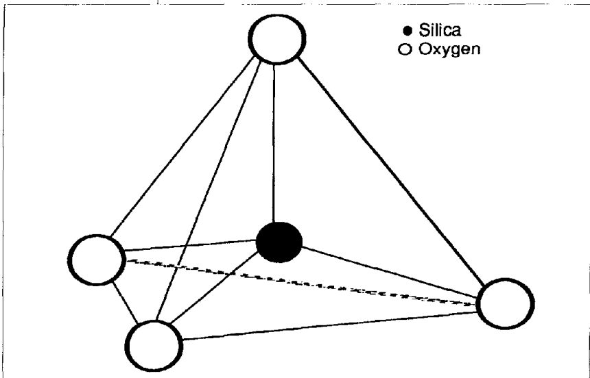
FIGURE 2. Silicon-Oxygen Tetrahedron
