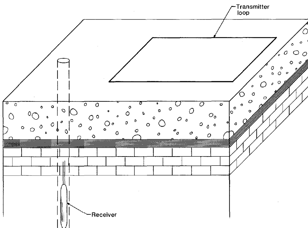
Figure 17.—Offset loop configuration.
