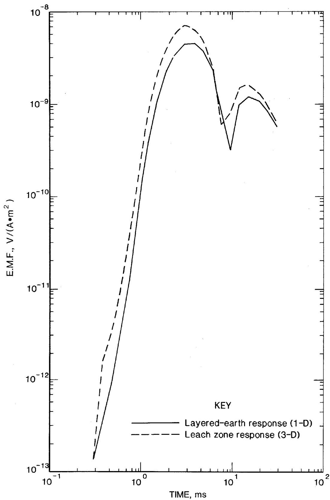
Figure 22.—TEM response in borehole 2 at depth of 690 m. Left peak corresponds to negative and right peak to positive E.M.F.
