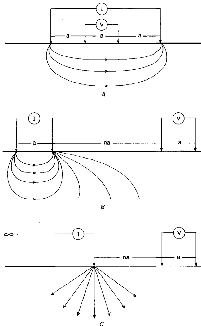
Figure 3.—Three common resistivity arrays. A, Wenner; B, dipole-dipole; C, pole-dipole. (I and V = current and voltage electrodes, respectively; a = electrode spacing; n = spacing multiplier, usually with values between 1 and 10.)
