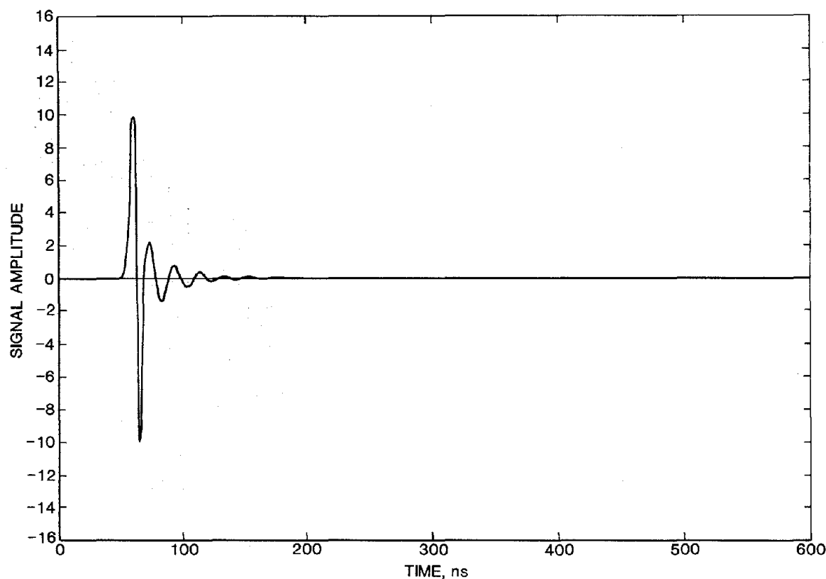
Figure 5.—Transmitted wavelet from GPR antenna.
