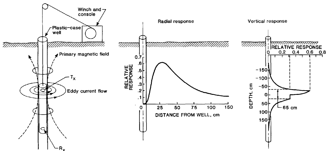
Figure 11.—Principle of operation of commercial borehole induction logger. ( T_x and R_x = transmitter and receiver coils, respectively.)
