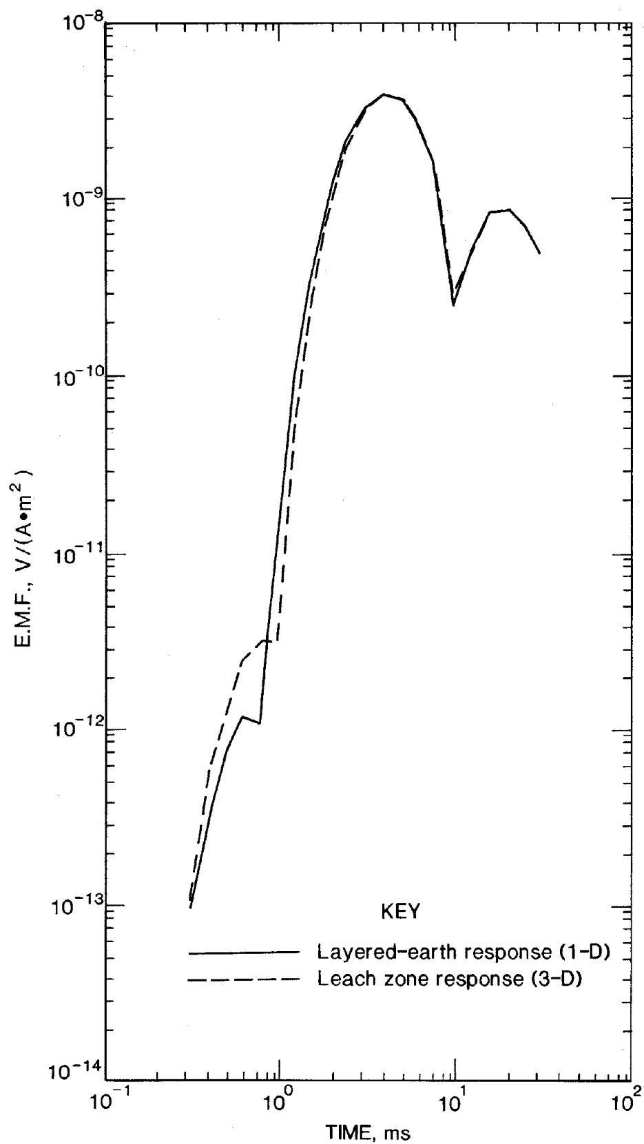
Figure 26.—TEM response in borehole 3 at depth of 720 m. Left peak corresponds to negative and right peak to positive E.M.F.
