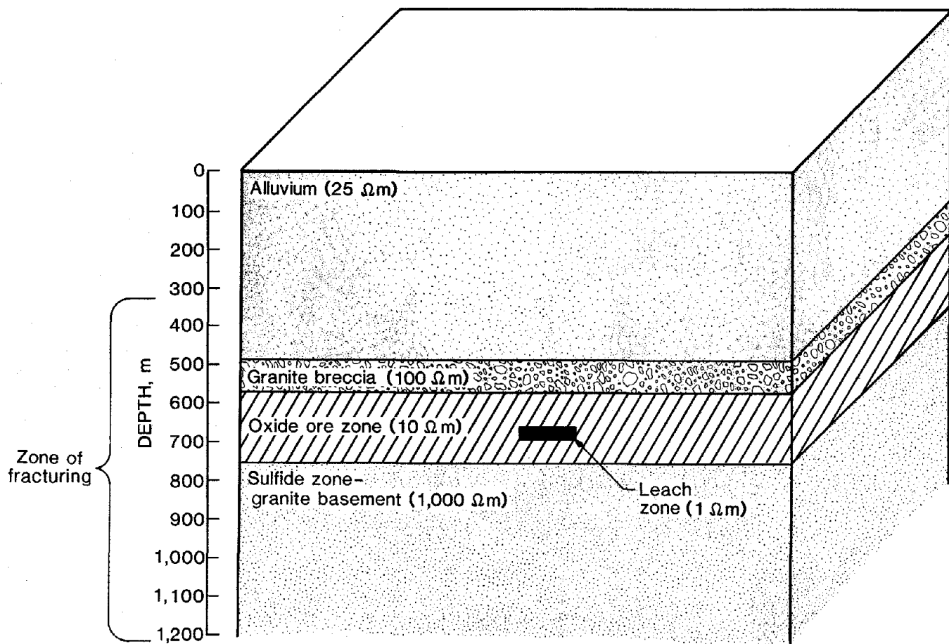
Figure 1.—Geoelectric section and leach zone of Santa Cruz site.
