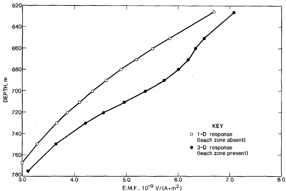
Figure 27.—Depth versus peak TEM response along section of borehole 1.
