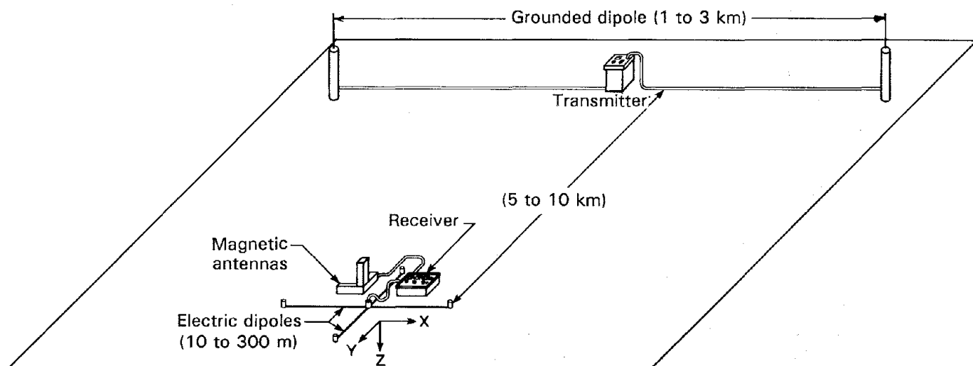
Figure 2.—Equipment configuration for CSAMT surveying.
