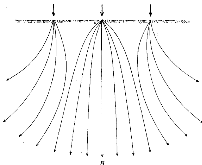
Figure 4.—Comparison of conventional (A) and focused (B) current injection as used in resistivity surveying.
