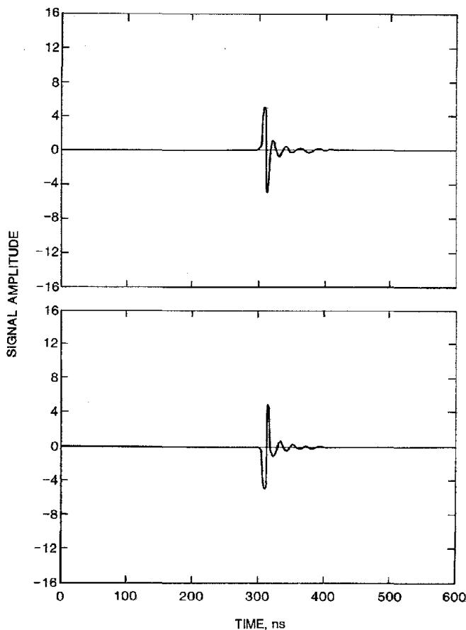
Figure 6.—Comparison of reflected pulses from nonconductor (top) and conductor (bottom).
