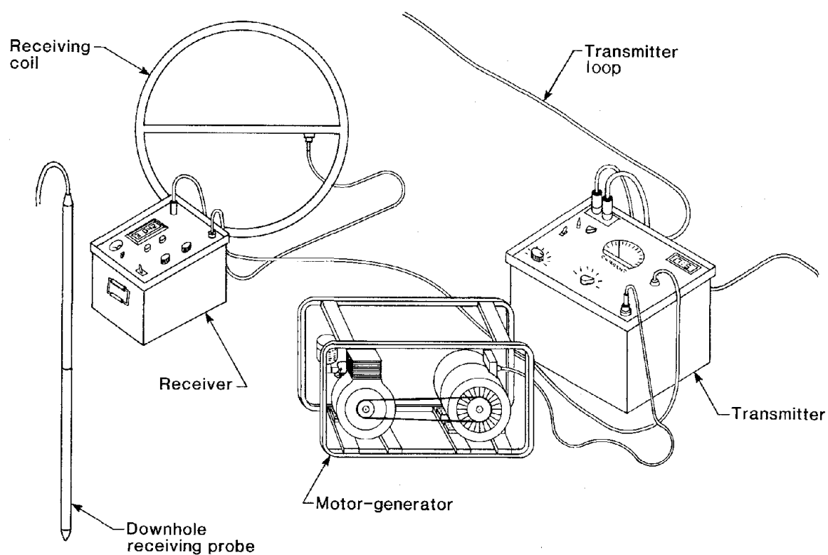
Figure 12.—Equipment used in TEM.
