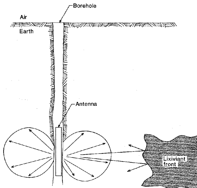
Figure 7.—Borehole GPR used to monitor lixiviant zone.
