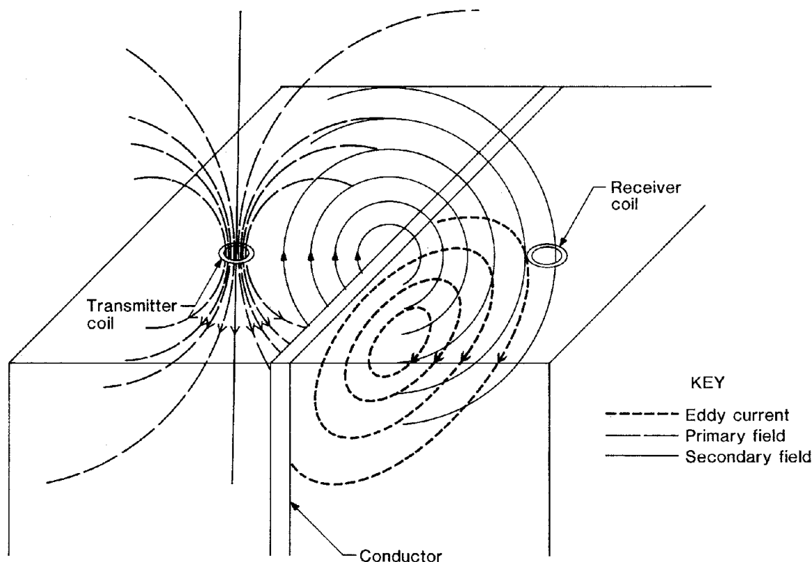
Figure 9.—EM field behavior near subsurface conductor.
