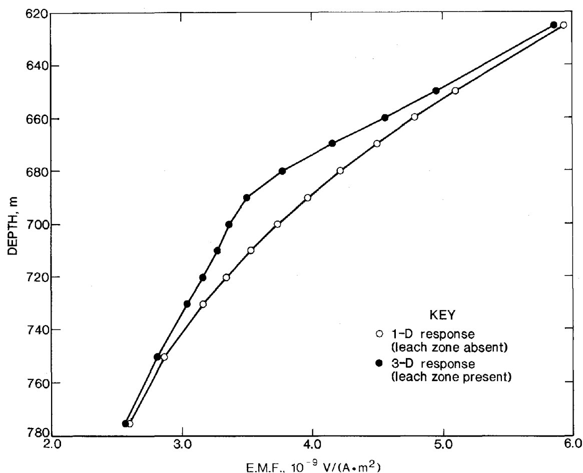
Figure 29.—Depth versus peak TEM response along section of borehole 3.
