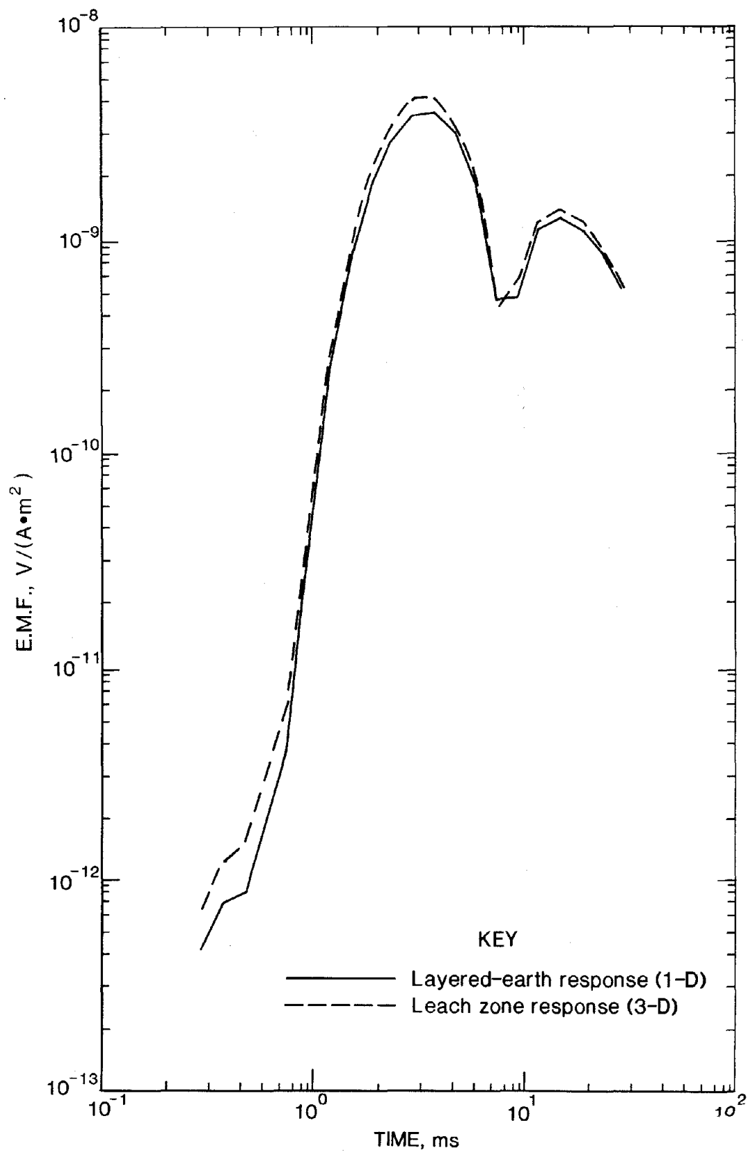
Figure 20.—TEM response in borehole 1 at depth of 720 m. Left peak corresponds to negative and right peak to positive E.M.F.
