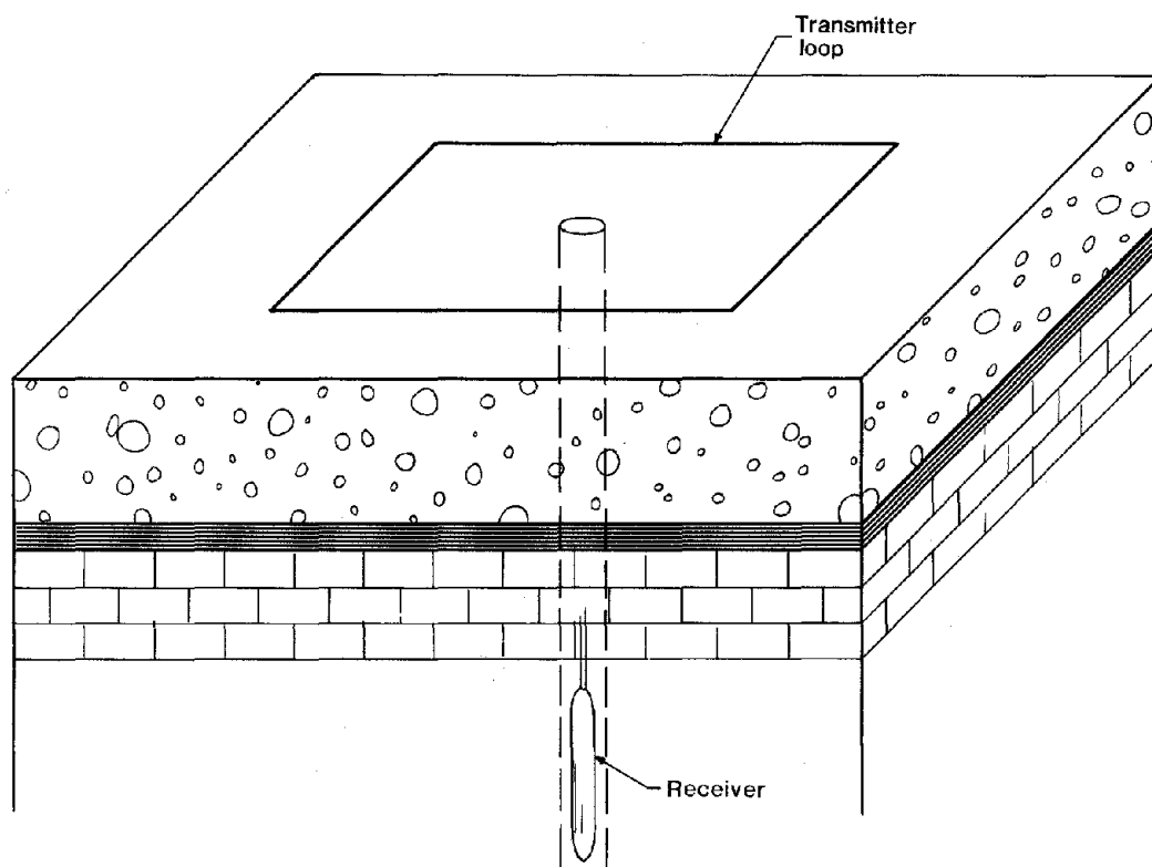
Figure 16.—Central induction configuration.
