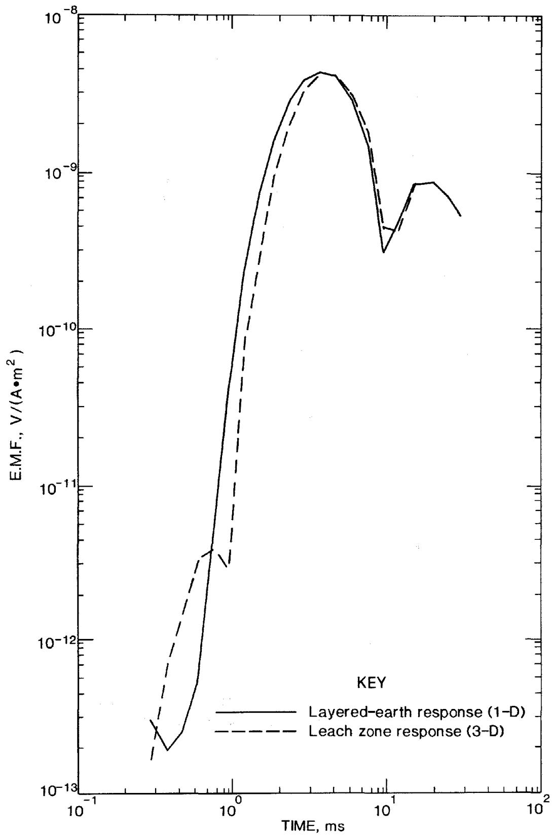
Figure 25.—TEM response in borehole 3 at depth of 690 m. Left peak corresponds to negative and right peak to positive E.M.F.
