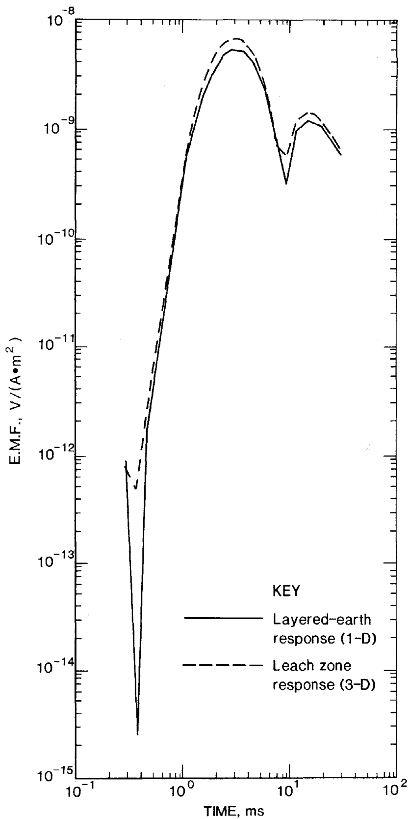
Figure 21.—TEM response in borehole 2 at depth of 660 m. Left peak corresponds to negative and right peak to positive E.M.F.
