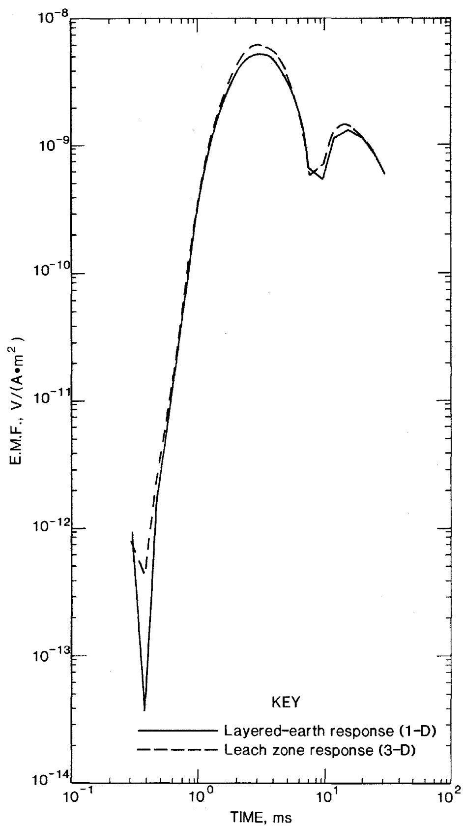
Figure 18.—TEM response in borehole 1 at depth of 660 m. Left peak corresponds to negative and right peak to positive E.M.F.
