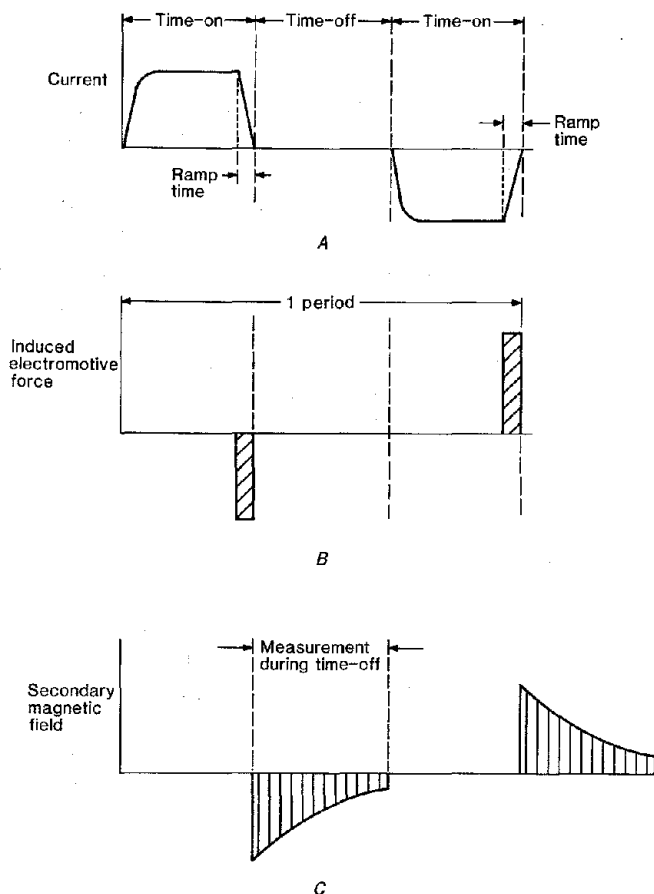
Figure 10.—Current waveforms and resultant secondary field observed in TEM. A, Current in transmitter loop; B, induced electromotive force caused by current; C, secondary magnetic field caused by eddy currents.
