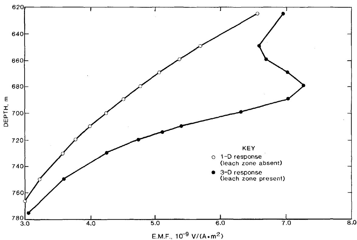
Figure 28.—Depth versus peak TEM response along section of borehole 2.
