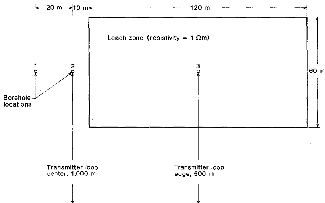
Figure 15.—Plan view of leach zone and borehole locations.
