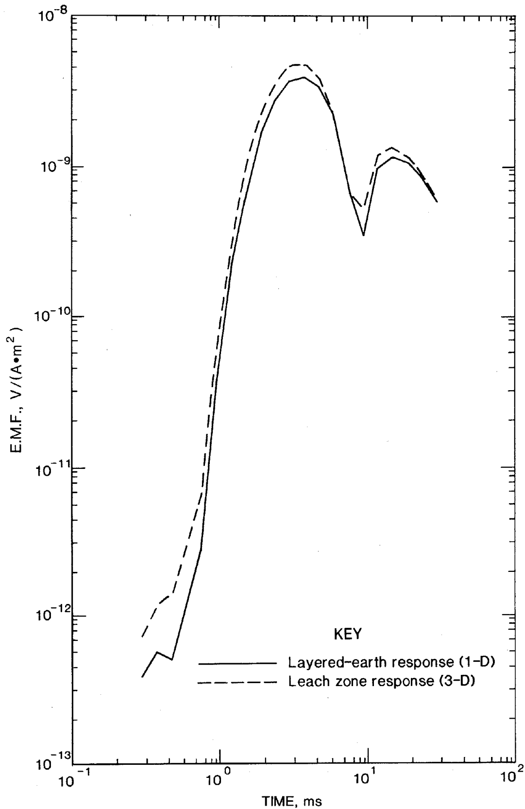
Figure 23.—TEM response in borehole 2 at depth of 720 m. Left peak corresponds to negative and right peak to positive E.M.F.
