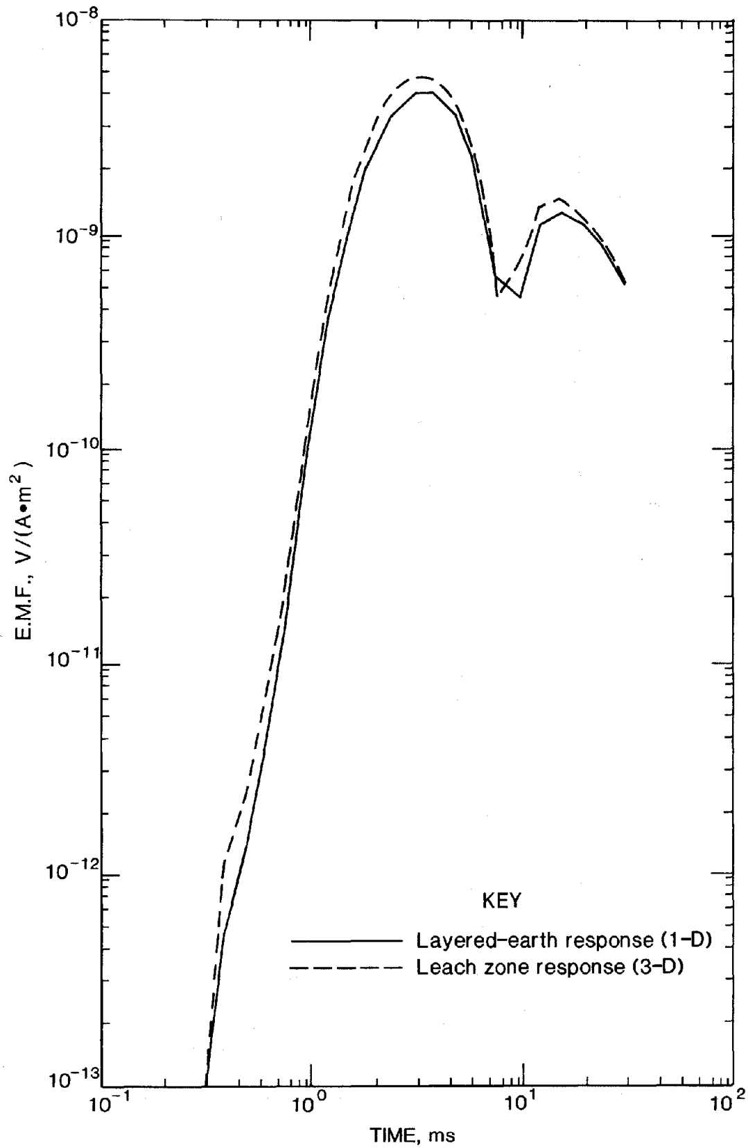
Figure 19.—TEM response in borehole 1 at depth of 690 m. Left peak corresponds to negative and right peak to positive E.M.F.
