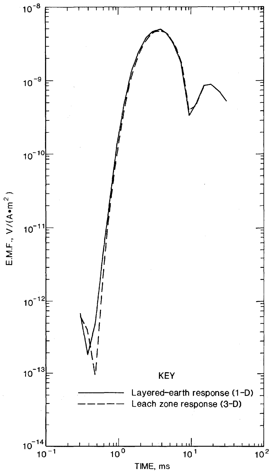
Figure 24.—TEM response in borehole 3 at depth of 660 m. Left peak corresponds to negative and right peak to positive E.M.F.
