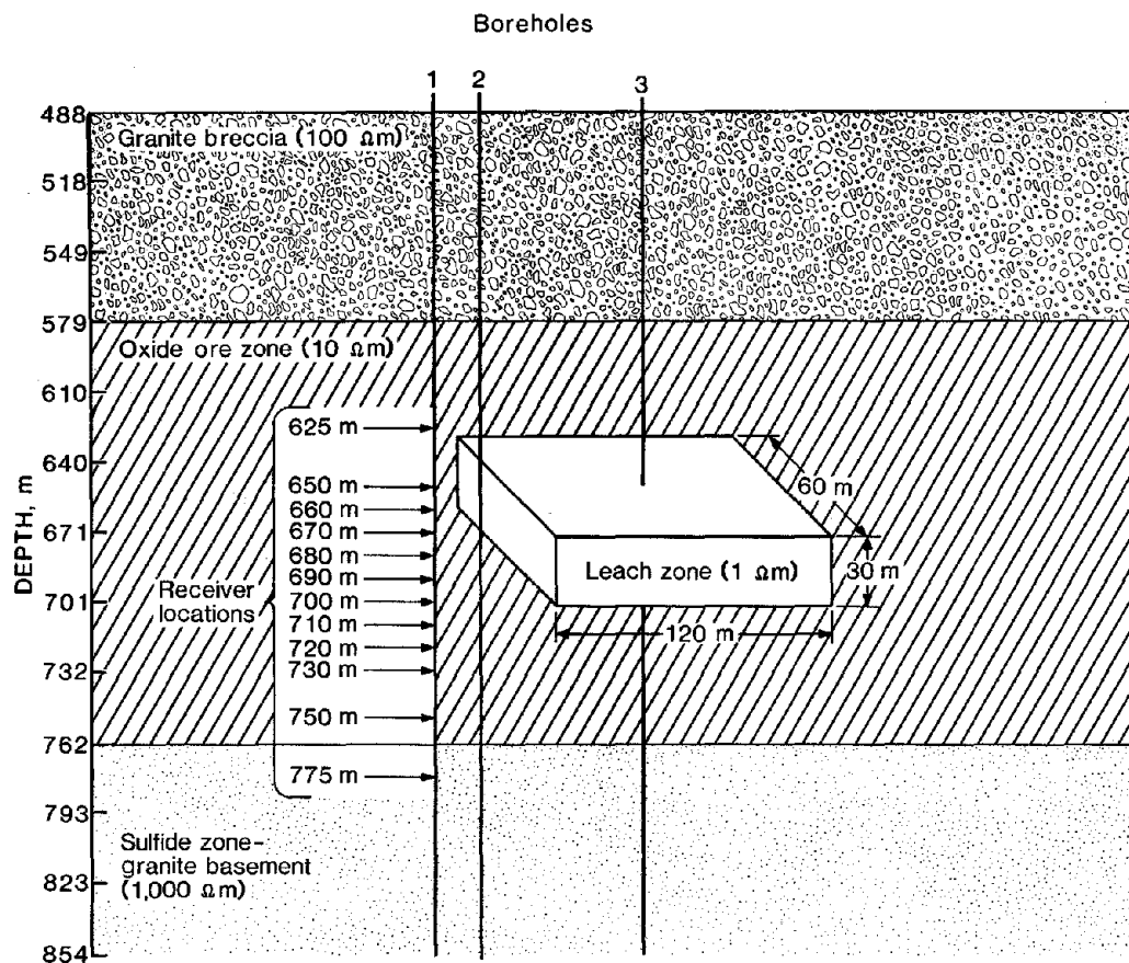
Figure 14.—Layered-earth model and leach zone.
