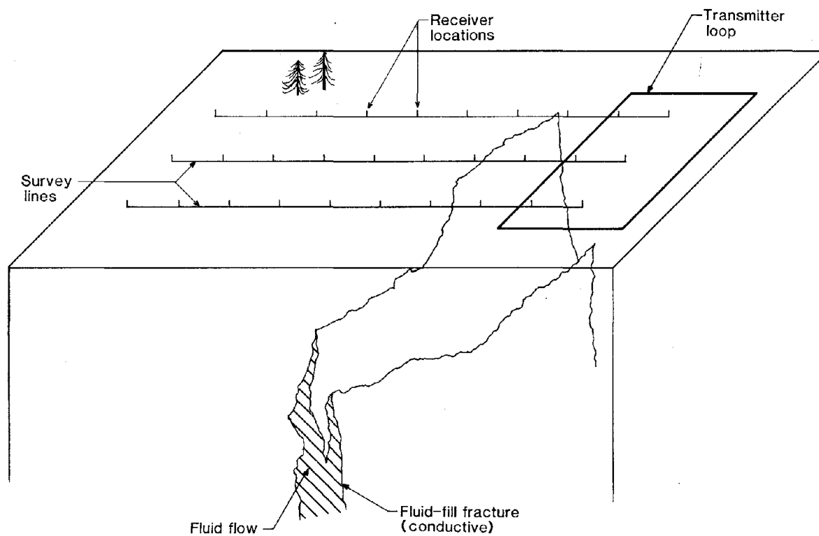
Figure 13.—Surface profiling over fluid-filled fracture zone.
