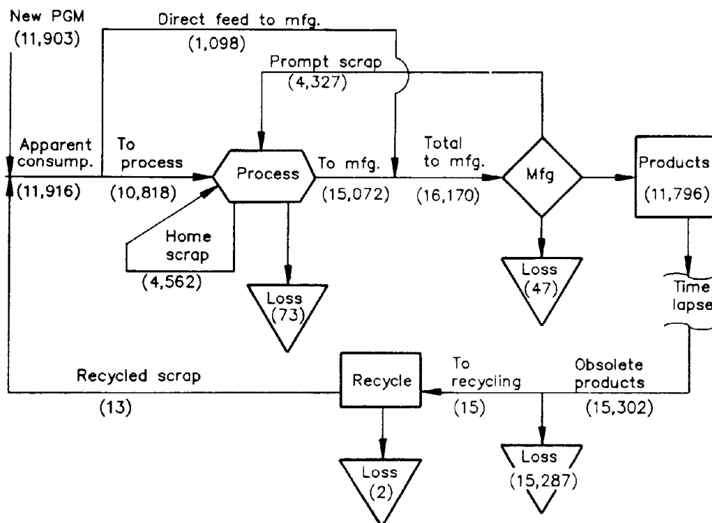
Figure 4.—Flow of PGM in dental and medical industry in 1989 (amounts in kilograms of contained PGM).
