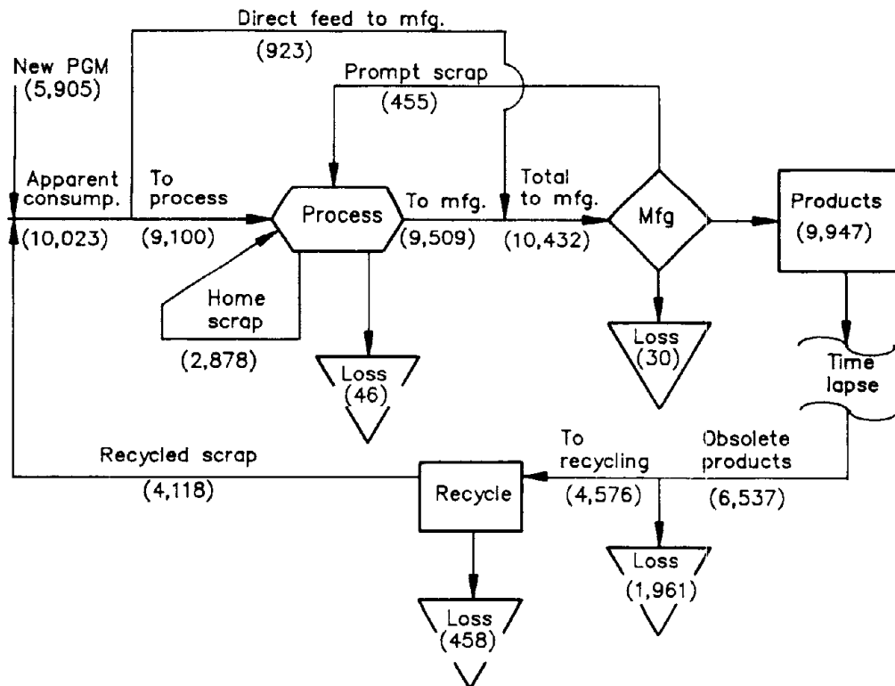
Figure 9.—Flow of PGM in miscellaneous other industries in 1989 (amounts in kilograms of contained PGM).
