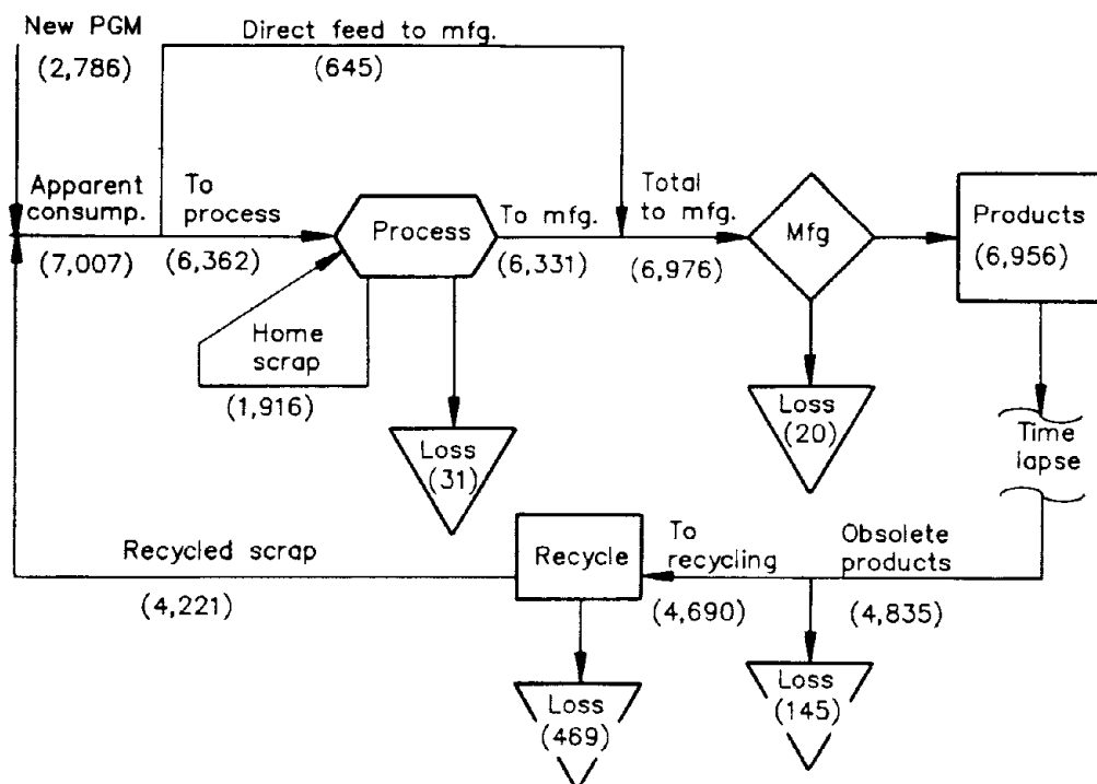
Figure 5.—Flow of PGM in petroleum industry in 1989 (amounts in kilograms of contained PGM).
