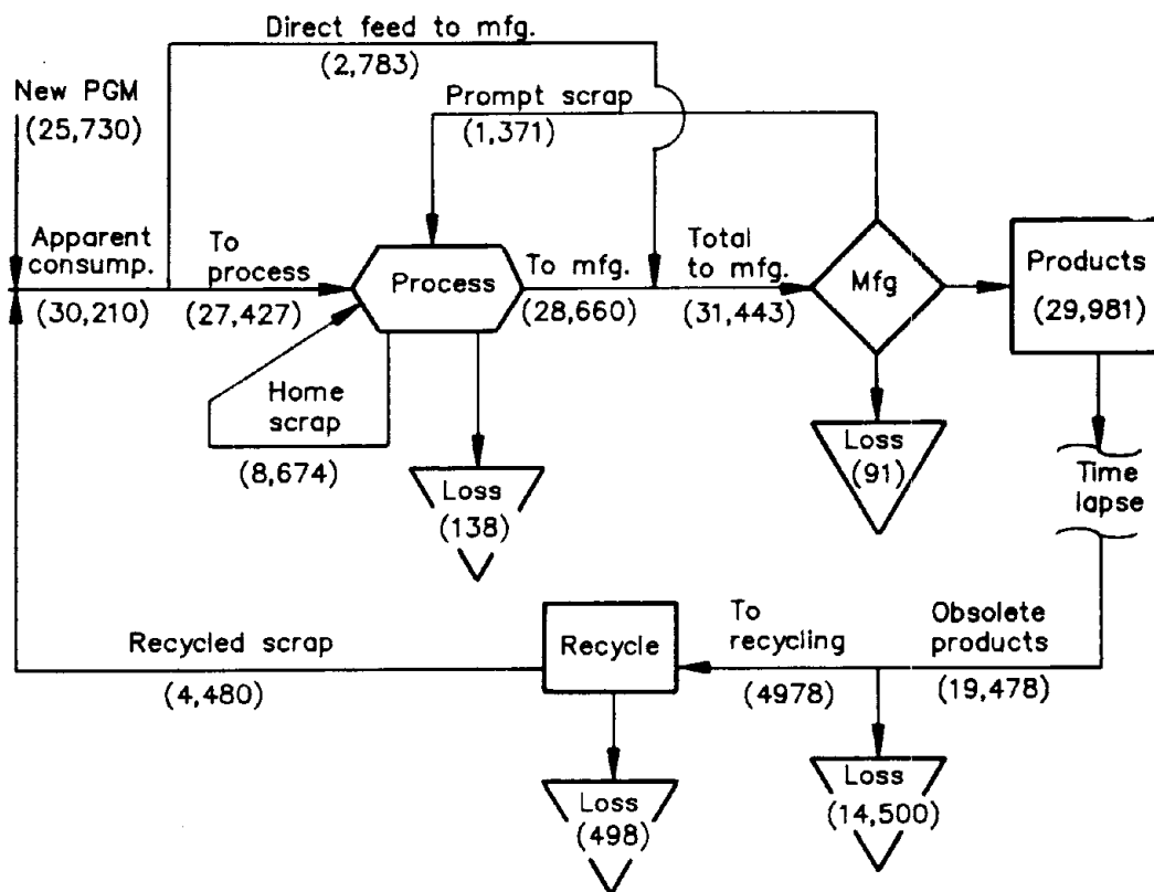
Figure 3.—Flow of PGM in electrical and electronics industry in 1989 (amounts in kilograms of contained PGM).
