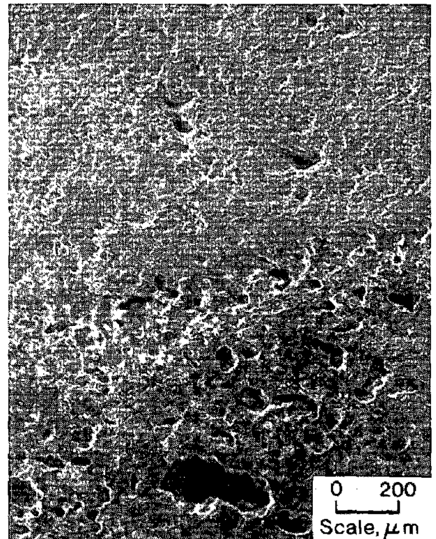
Figure 5.—SEI of Mn ore from Algoma-Zeno deposit (shown in figure 3) showing resulting porous topography after leaching Mn from lower half of mixed pyrolusite-hematite ore.
