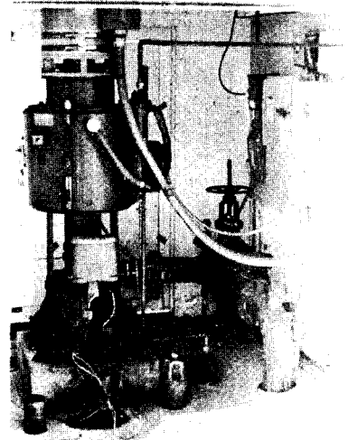
FIGURE 7. - Space heating system, Oregon Technical Institute, Klamath Falls, Oreg.
