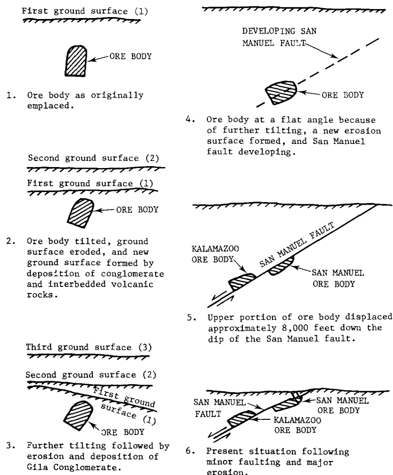
FIGURE 9. - Schematic cross-section drawings showing possible origin of Kalamazoo ore body. (Adapted from Lowell, Econ. Geol., v. 63, No. 6, 1968.)
