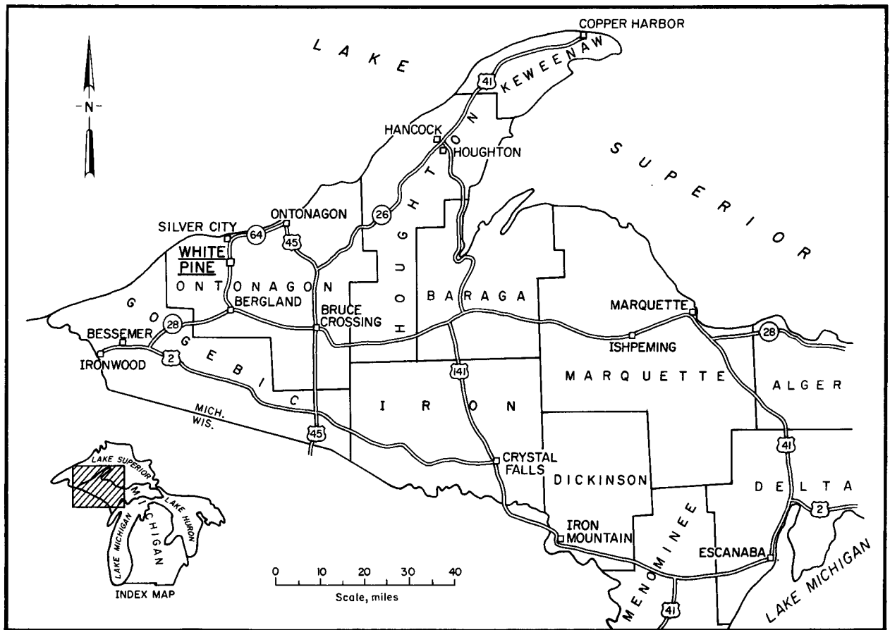
FIGURE 17. - Location map, White Pine copper mine, Ontonagon County, Mich.
