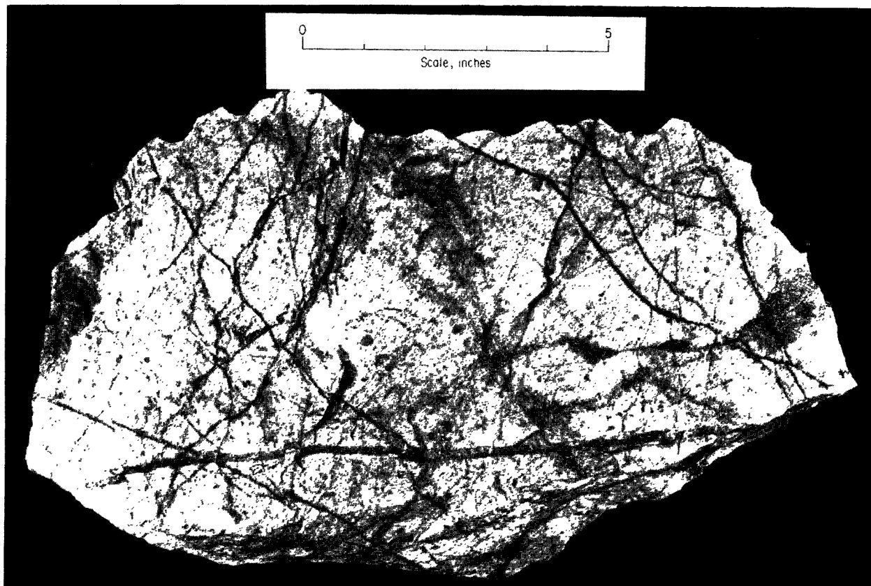
FIGURE 6. - Slab of ore showing typical stockwork of crisscrossing veinlets of molybdenite in gangue rock.
