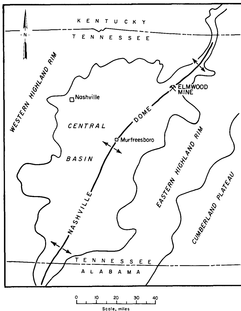
FIGURE 4. - Location map, Elmwood zinc deposit, central Tennessee. (Adapted from W. H. Callahan, Econ. Geol., v. 72, No. 7, 1977.)
