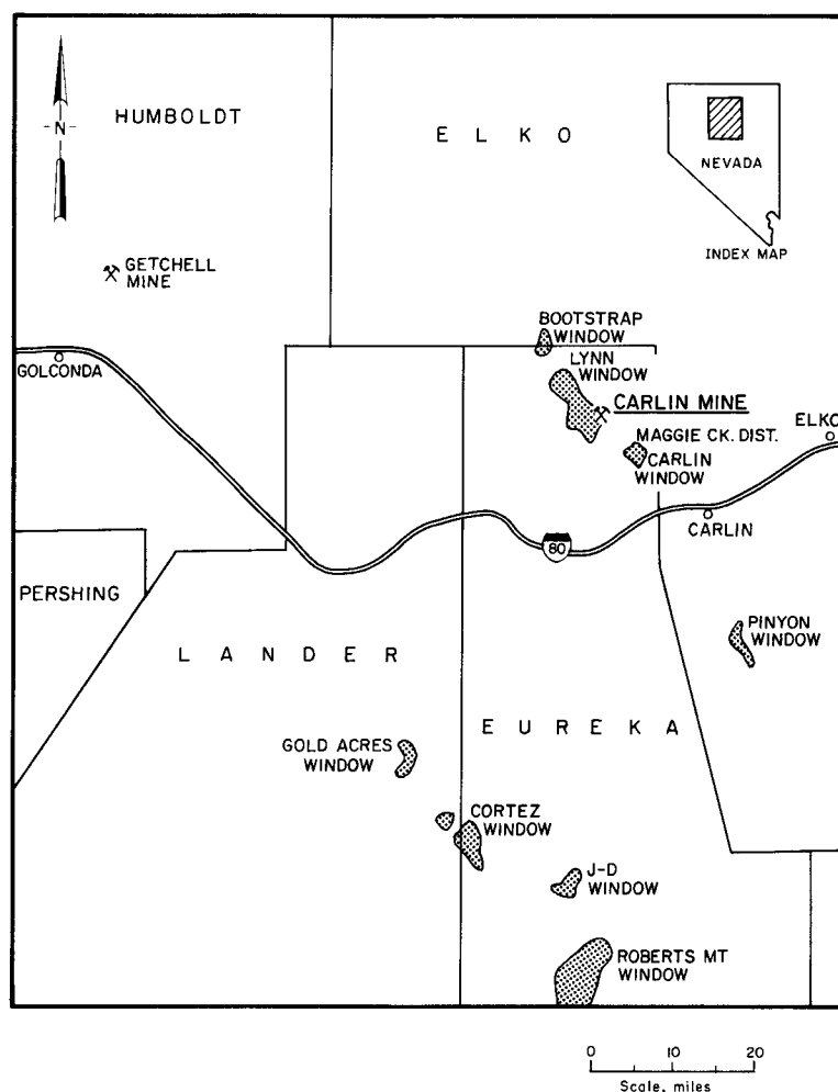
FIGURE 2. - Location map, Carlin gold mine, Eureka County, Nev. (Adapted from Ore Deposits of the United States, 1933-1967 , AIME, New York.)
