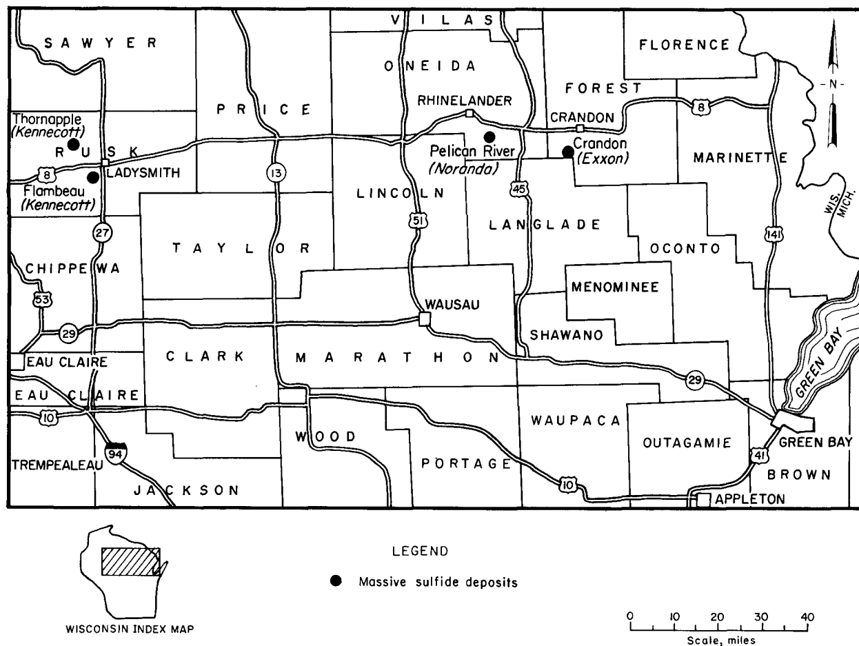
FIGURE 5. - Location map, massive sulfide deposits of northern Wisconsin.
