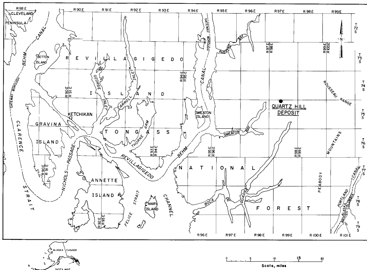
FIGURE 13. - Map showing approximate location of Quartz Hill molybdenum deposit, Tongass National Forest, southeastern Alaska.
