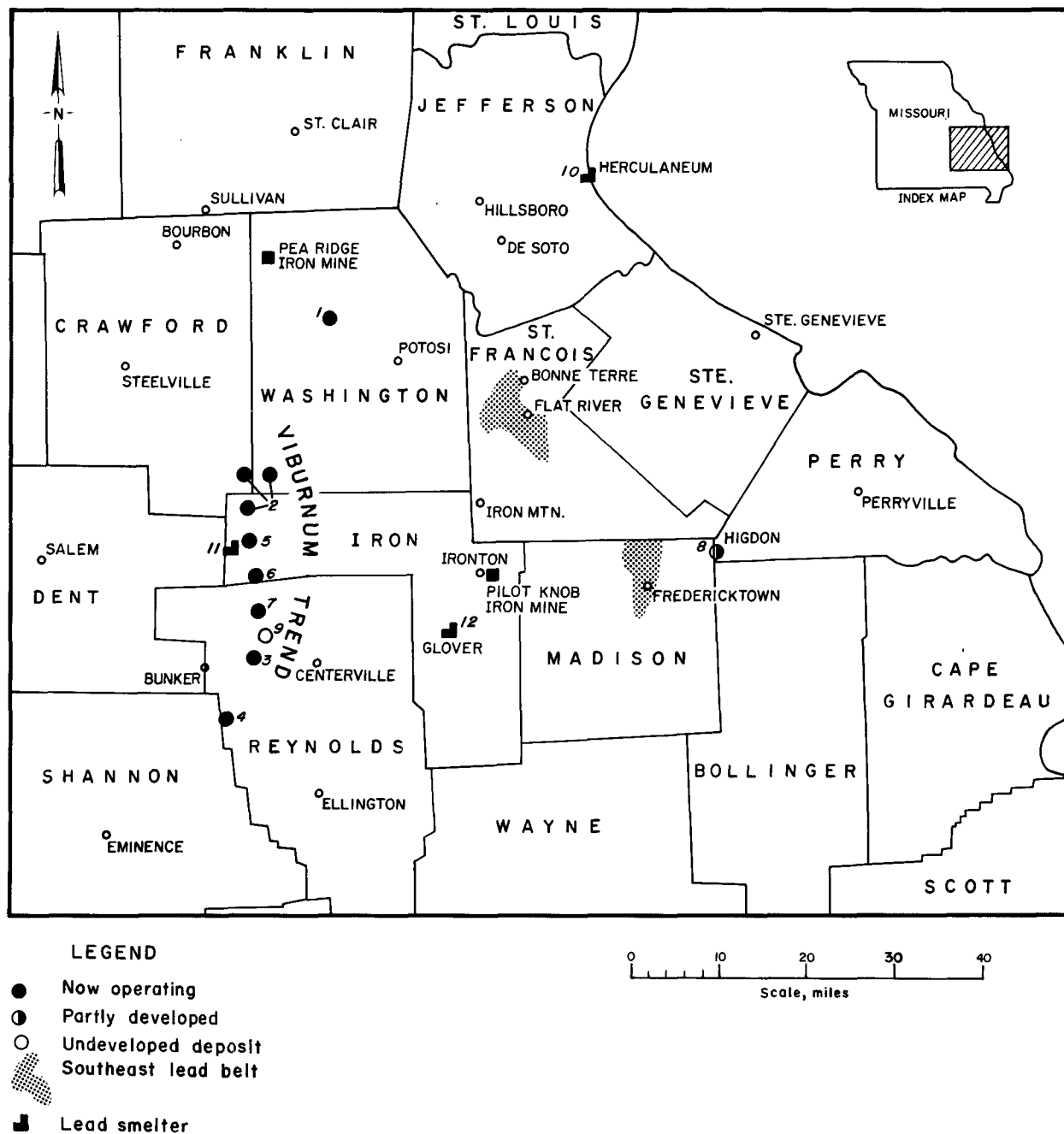
FIGURE 10. - Map showing lead deposits and operations in the southeast Missouri lead district. Lead-zinc-copper operations: 1, St. Joe Minerals Corp. Indian Creek Div. mines and mill; 2, St. Joe Minerals Corp. Viburnum Div. mines and mill; 3, St. Joe Minerals Corp. Fletcher Div. mine and mill; 4, Sweetwater mine and mill, Ozark Lead Co., subsidiary of Kennecott Copper Corp.; 5, Magmont mine and mill, Cominco American Inc. and Dresser Industries Inc.; 6, Buick mine and mill, AMAX-Homestake (AMAX Lead Co. of Missouri and AMAX-Homestake Missouri lead complex); 7, Brushy Creek Div. mine and mill; 8, Higdon mine, the Bunker Hill Co. and NL Industries, Inc.; 9, West Fork deposit, American Smelting and Refining Co. (ASARCO). Lead smelters: 10, St. Joe Minerals Corp. Herculaneum Div. plant; 11, AMAX-Homestake Buick smelter; 12, ASARCO Clover plant. (Adapted from the Viburnum Trend Guidebook, Missouri Department of Natural Resources.)
