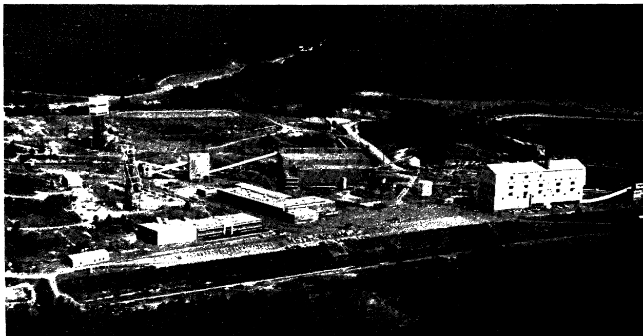
FIGURE 11. - Surface plant, mill, and pellet plant at the Pea Ridge iron mine, Washington County, Mo.
