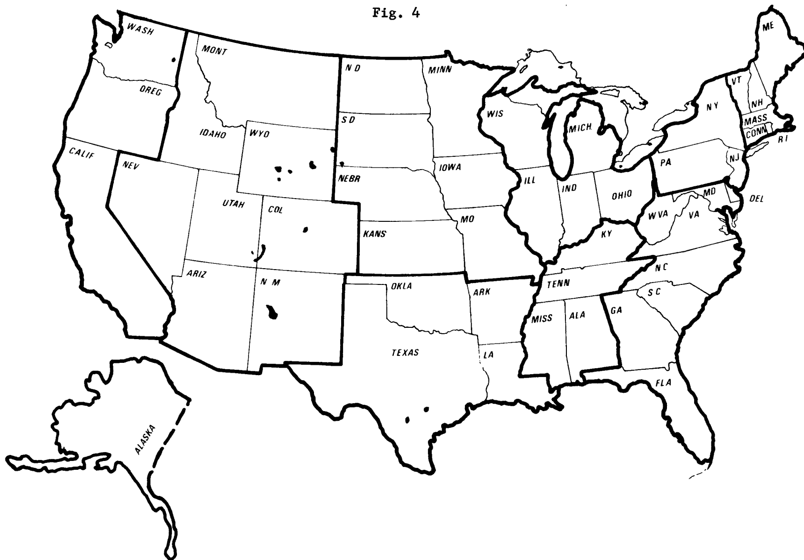
FIGURE 4. - Principal uranium deposits of the United States.
