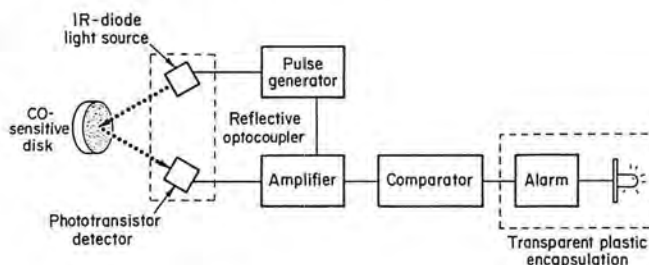
Figure 3.—PEMCOAL 2 electrical function diagram.
