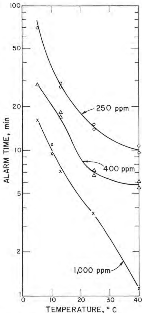
Figure 8.—Effect of temperature on PEMCOAL alarm times.
