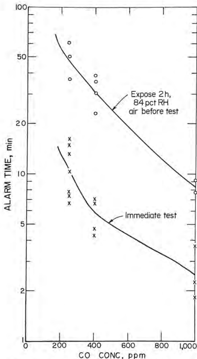
Figure 6.—Effect of CO concentration and humidity on the PEMCOAL alarm time.
