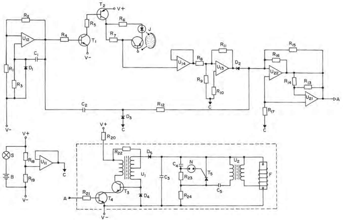
Figure A-1.-Electrical schematic for PEMCOAL 2. See table A-1 for a description of components.
