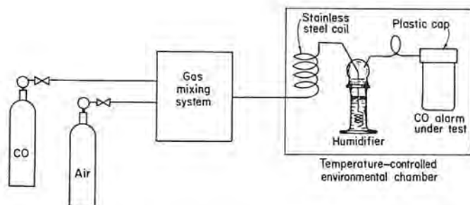
Figure 5.—Apparatus for test of carbon monoxide alarm.
