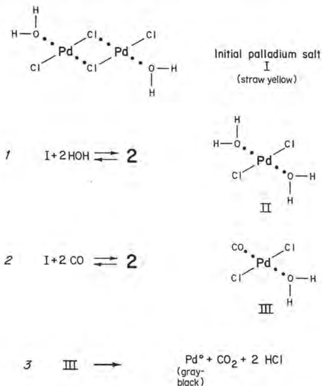
Figure 9.—Proposed reaction sequences for palladium chloride with carbon monoxide and water.
