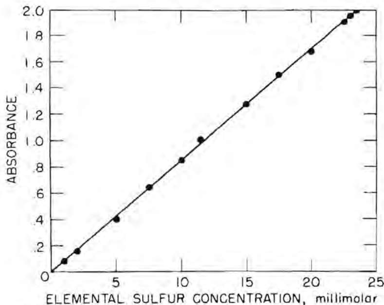
FIGURE 1. - Trichloroethylene solution absorbance as a function of sulfur concentration (1-millimeter cell).
