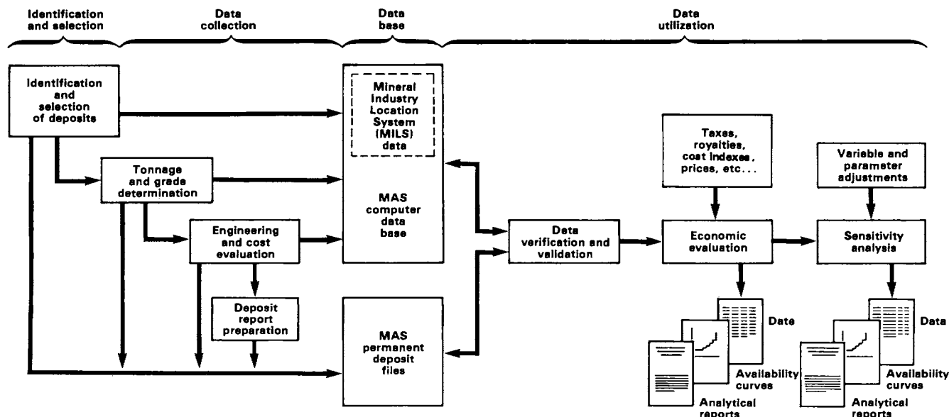
FIGURE 2. - MAS program workflow.
