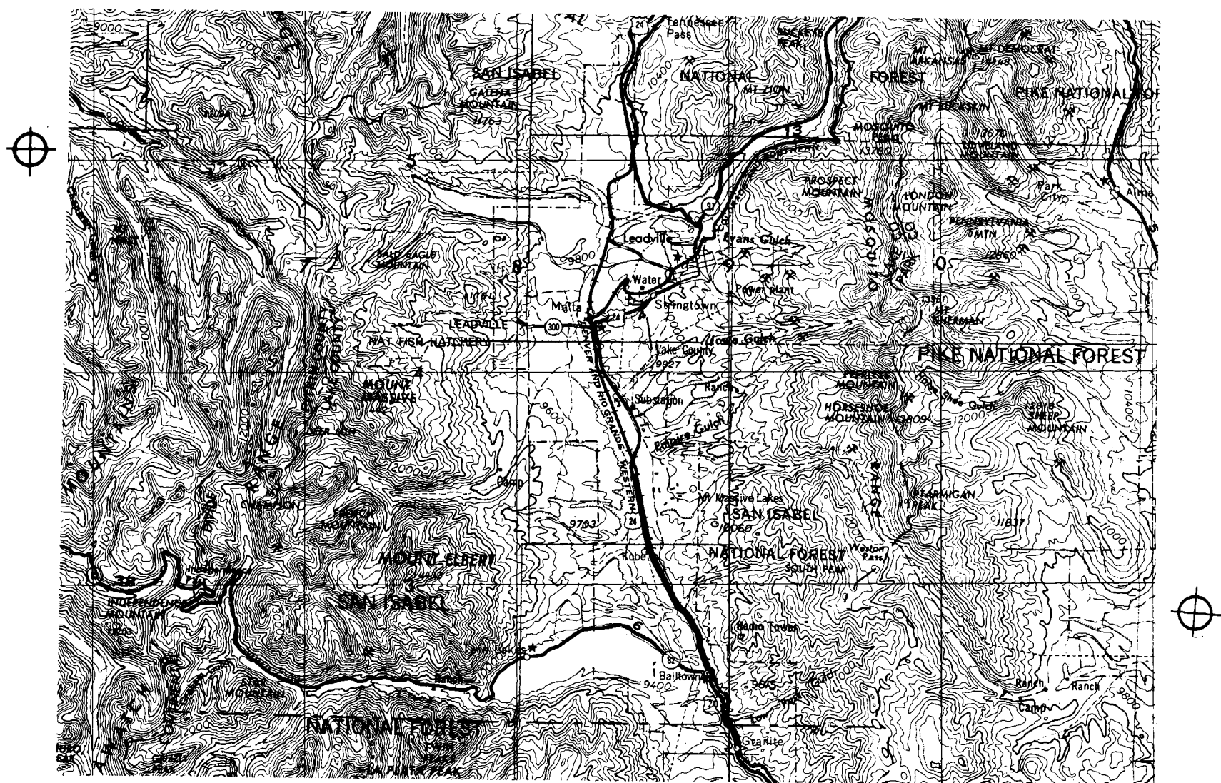
FIGURE 10. - Leadville, Colo., 1:250,000 scale quadrangle.
