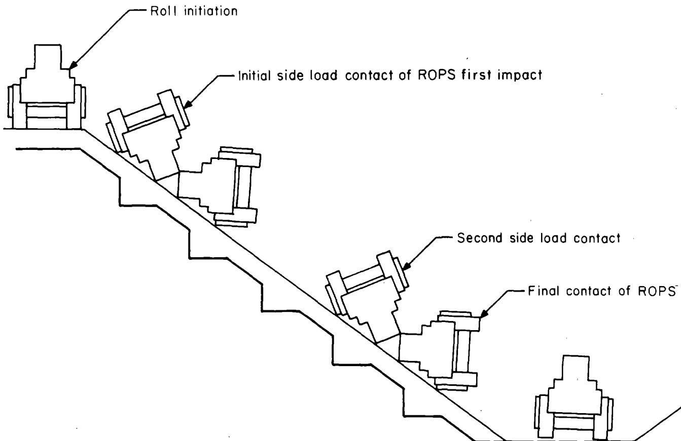
Figure 1. — Equivalent rollover, 720°.
