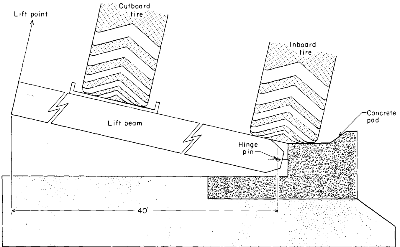
Figure 2. — Tilt table.
