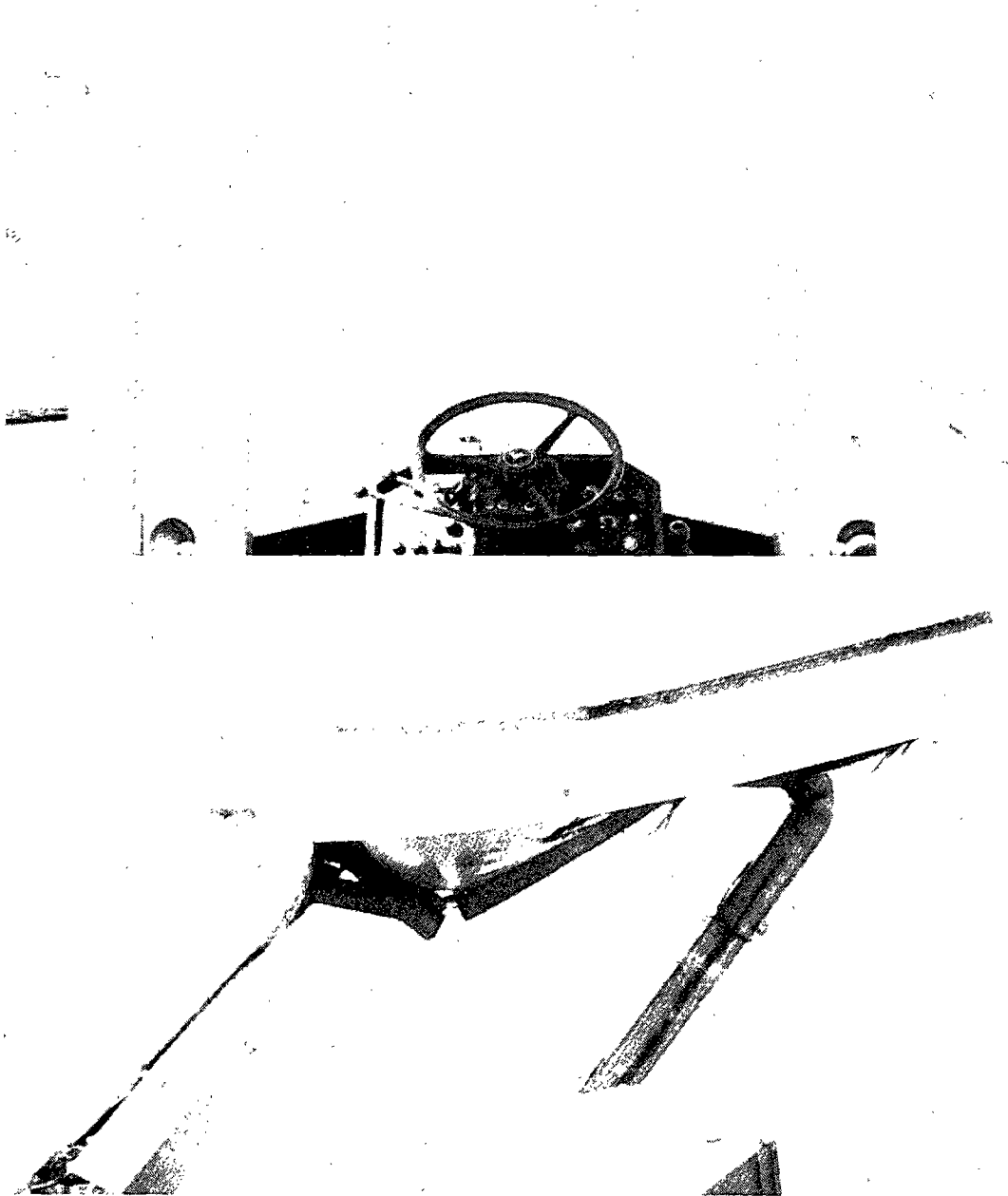
Figure 4. — ROPS before (top) and after (bottom) rollover, 52,000-lb-GVW, wheeled, front-end loader.
