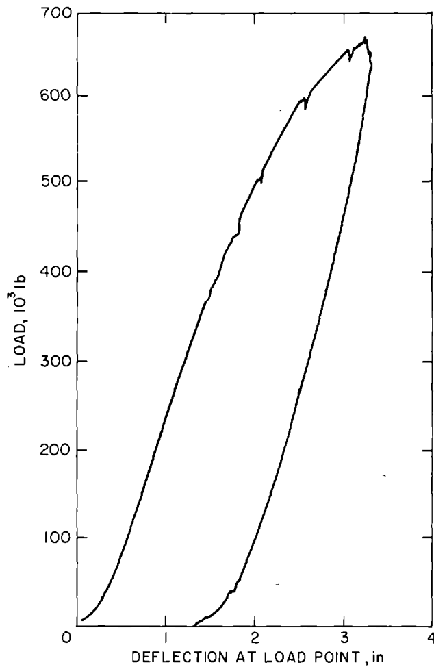
Figure 10. — Static test longitudinal load deflection curve, 390,000-lb-GVW, wheeled, front-end loader.
