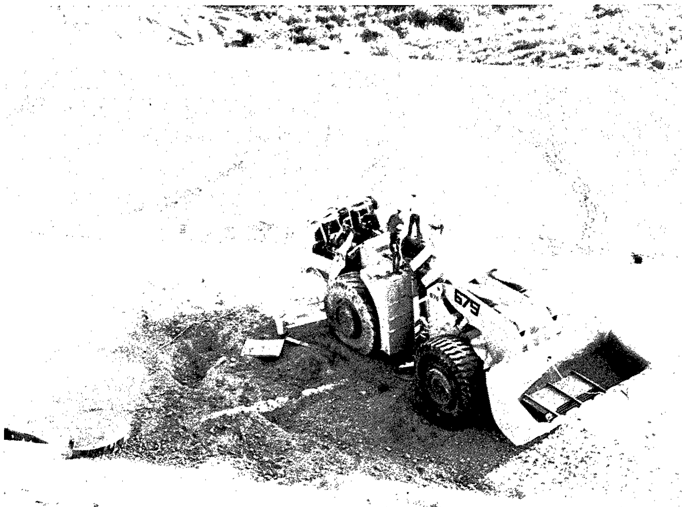
Figure 5. — First 390,000-lb-GVW, wheeled, front-end loader after rollover.
