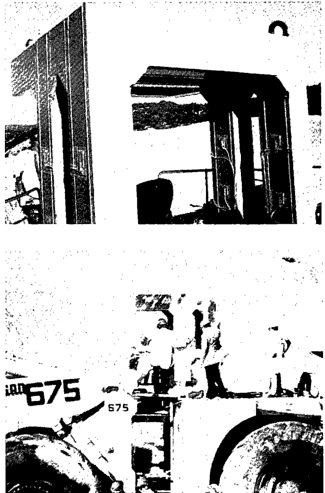
Figure 7. — Second 390,000-lb-GVW, wheeled, front-end loader before (top) and after (bottom) rollover.
