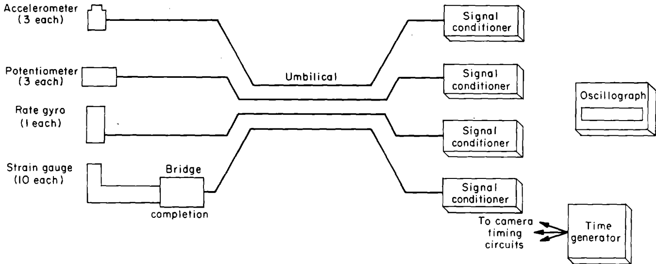
Figure 3. — Instrumentation schematic.
