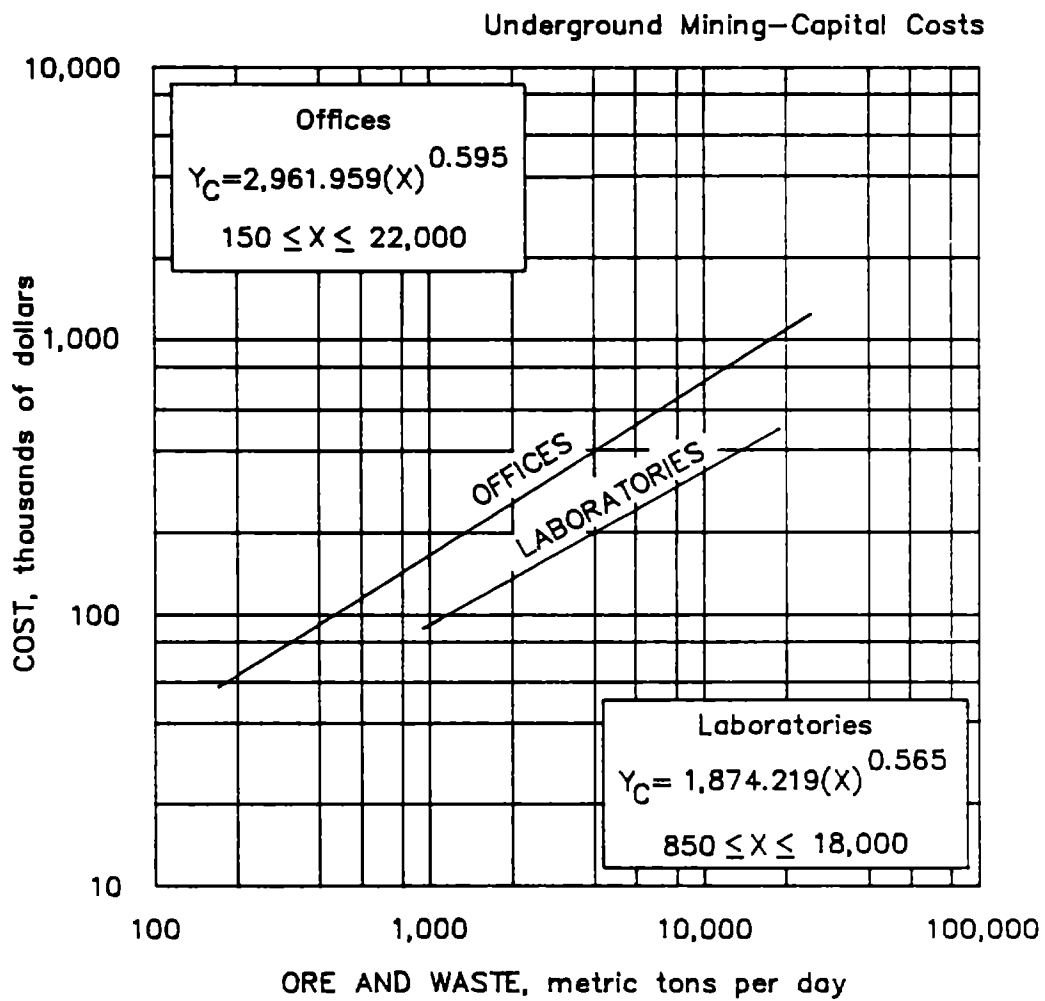
4.2.5.6.b Offices and laboratories
