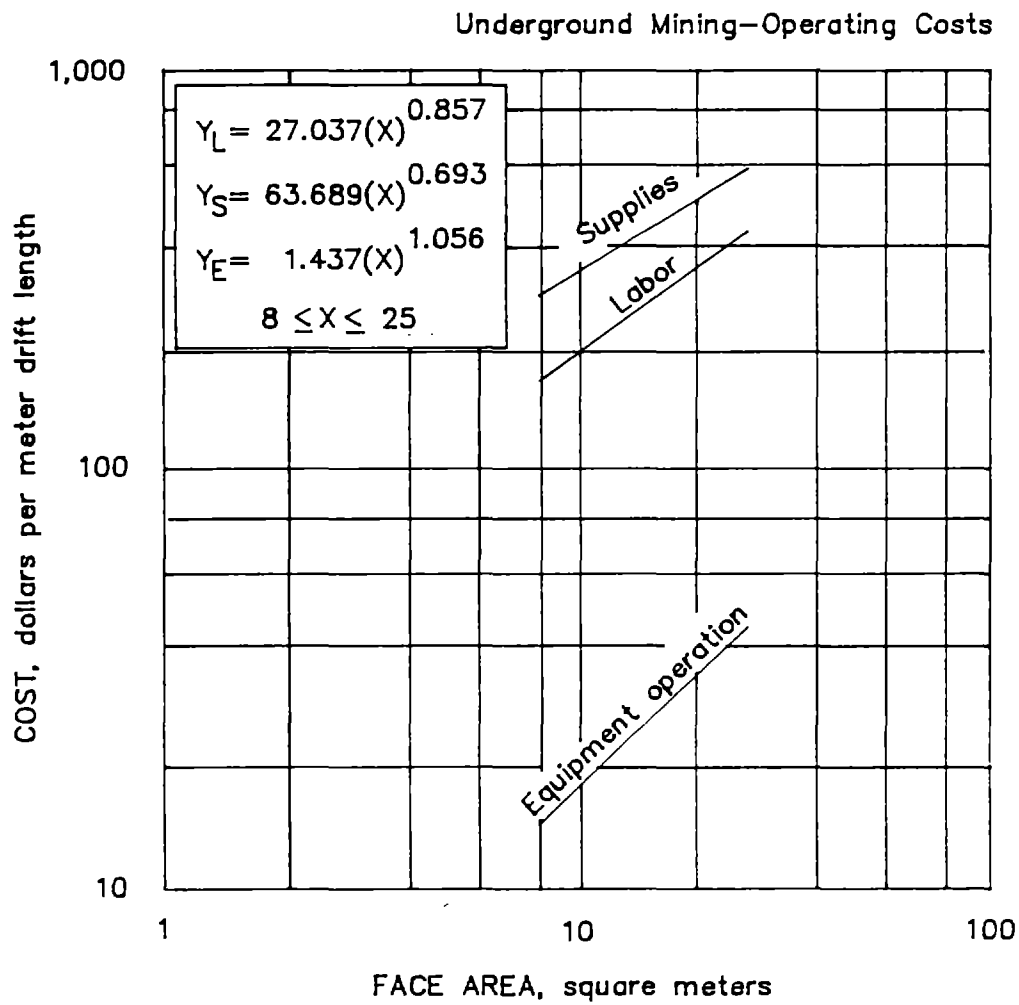
5.2.1.4.4. Drift development LARGE DRIFTS FOR RAIL HAULAGE
