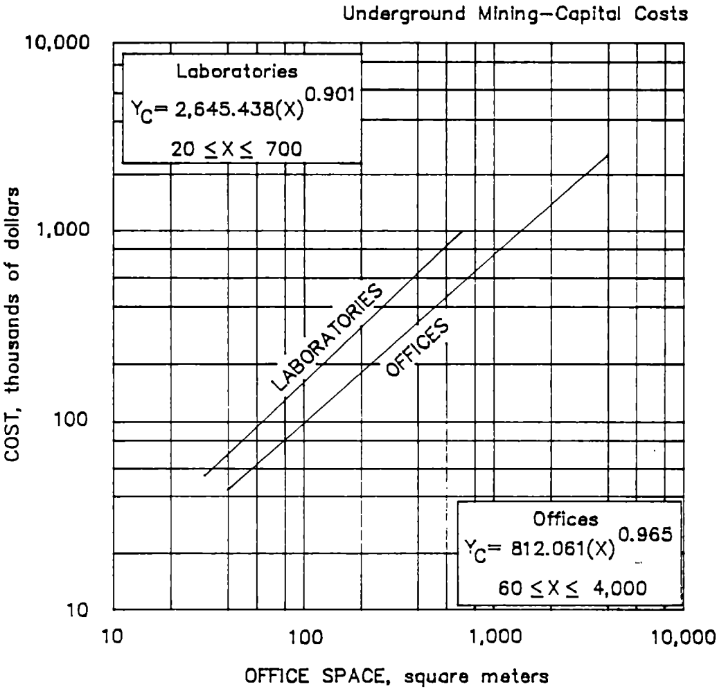
4.2.5.6.a Offices and laboratories
