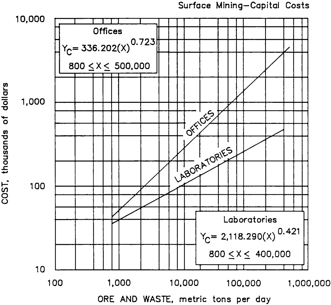
2.2.4.5.b Offices and laboratories
