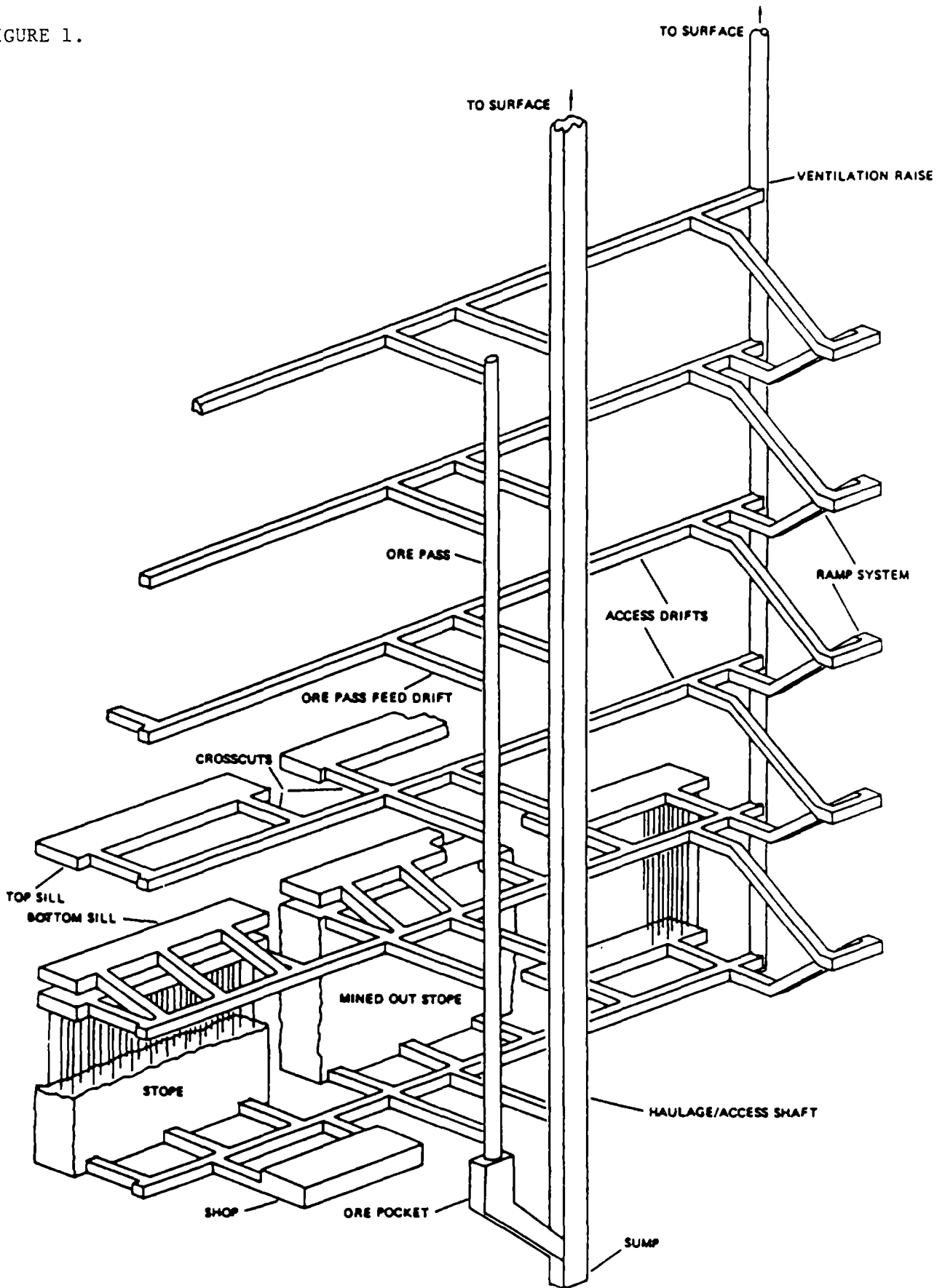
GENERALIZED VERTICAL CRATER RETREAT MINE
