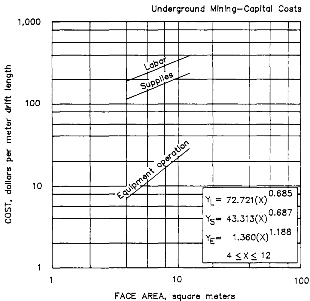
4.2.1.4.2. Drift development SMALL DRIFTS FOR RUBBER-TIRED HAULAGE
