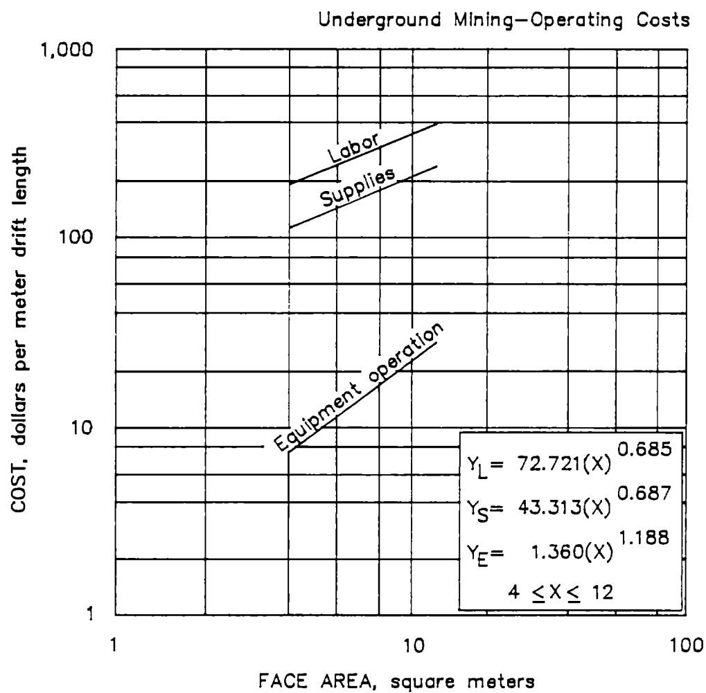
5.2.1.4.2. Drift development SMALL DRIFTS FOR RUBBER-TIRED HAULAGE
