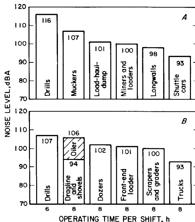
Figure 8-4.—Typical noise levels of machinery in underground (A) and surface (B) mining (18). (Courtesy of U.S. Mine Safety and Health Administration)
