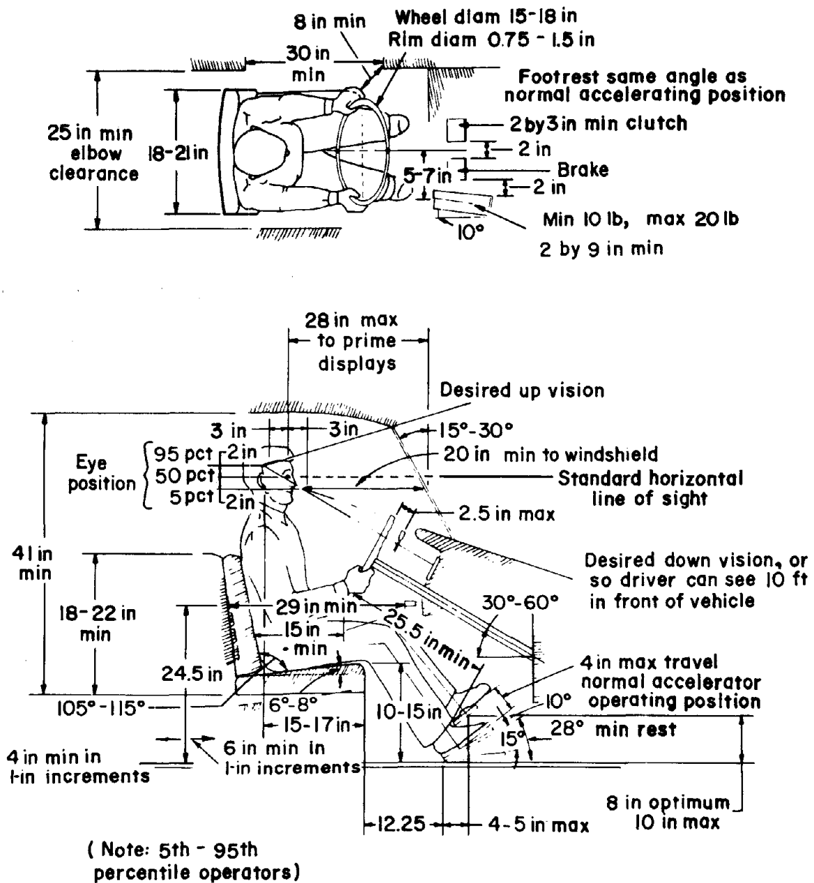
Figure 6-16.—Recommended configurations of a vehicle cab (32). (Copyright 1972 by John Wiley and Sons Ltd., and reprinted by permission)
