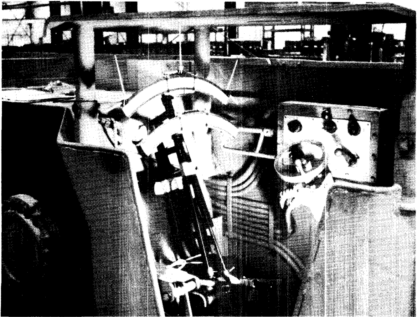
Figure 6-30.—Human eye reference measurement instrument (HERMI) used to assess fields of visibility from operators' cabs. The white arcs represent the 95th percentile male and 5th percentile female eye positions allowing reasonable head and trunk flexion (26).
