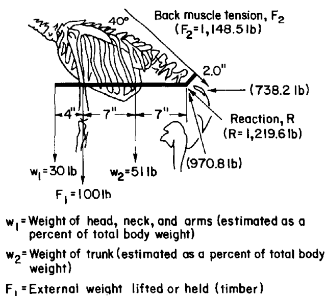
Figure 7-15.—Calculated lower-back muscle force and compressive (reactive) forces acting on L_5-S_1 disk resulting from lifting a timber post (6). (Copyright 1983 by the Human Factors Society Inc., and reproduced by permission)
