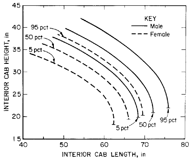
Figure 6-22.—Relationship between interior cab height and required interior cab length needed to accommodate various sized people. Assumes a 10^\circ seam pitch and 2-in helmet clearance (7). (Courtesy of R. Cooksey, University of New England)
