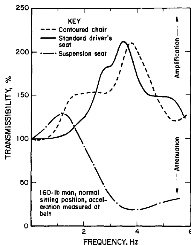
Figure 8-9.—Mechanical response of a person's body to vibrations when sitting in different seats (39).
