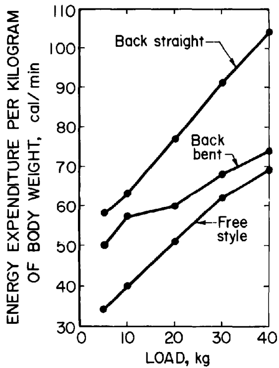
Figure 7.7.—Effect of weight of objects being lifted and lift posture on energy expenditure (27). (Courtesy of National Institute for Occupational Safety and Health)
