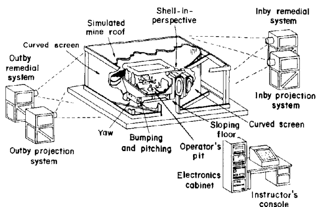
Figure 9-3.—Shuttle car training system full-task simulator (29).
