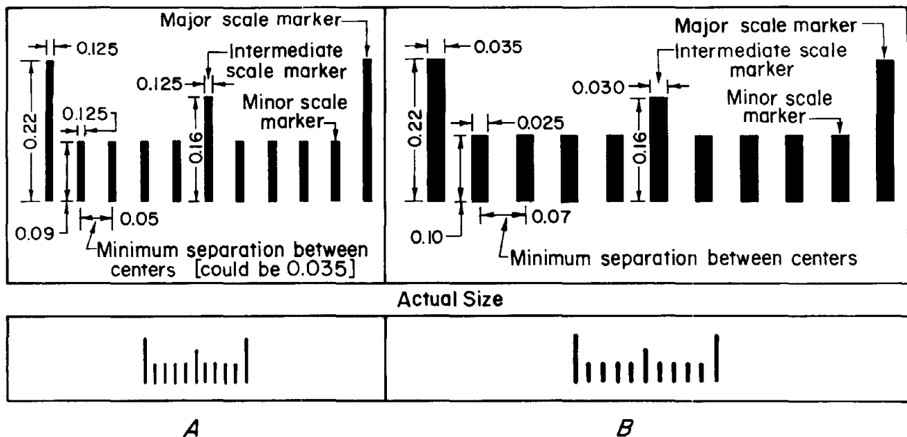
Figure 5-3.—Recommended format for quantitative scales under normal (A) and low (B) illumination conditions (adapted by McCormick (12) from reference 7). (Courtesy of McGraw-Hill)
