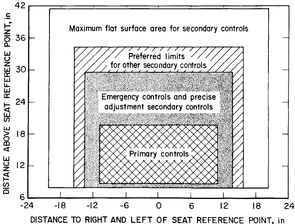
Figure 6-14.—Preferred vertical surface areas and limits for various types of control functions operated by a seated operator (adapted from 20). (Courtesy of McGraw-Hill)
