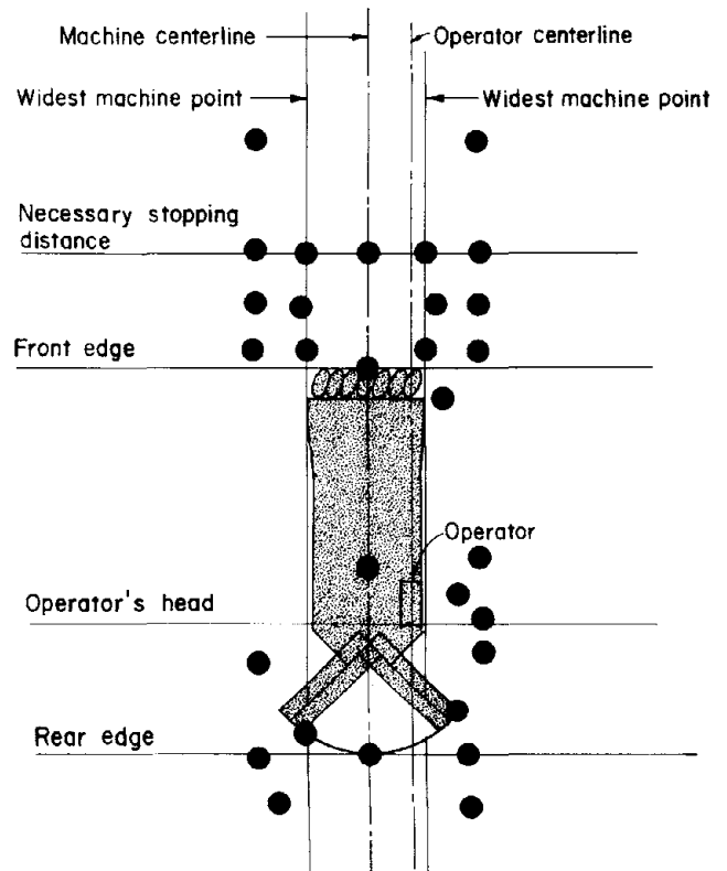
Figure 6-29.—Plan view of visual attention locations (VAL's) identified for continuous miner operators. Several vertical heights are represented at each VAL (25).
