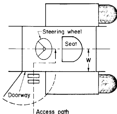
Figure 6-35.—Schematic diagram showing relationship of seat, steering wheel, and doorway on a typical tractor ( W is effective platform width) (3). This design requires the driver to maneuver around the steering wheel. (Courtesy of Butterworth Scientific Ltd.)
