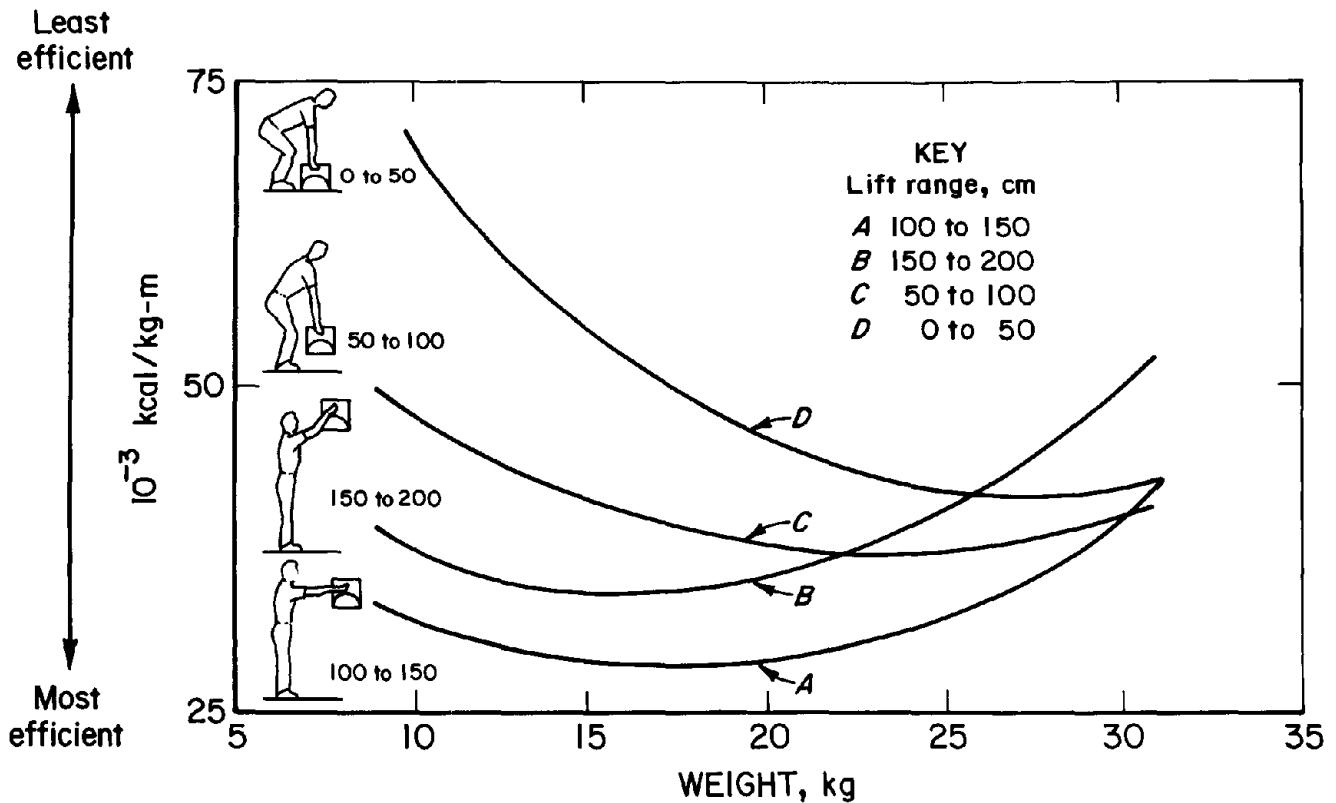
Figure 7.9.—Energy efficiency of lifting various weights from different starting positions (12). (Courtesy of Butterworth Scientific Ltd.)
