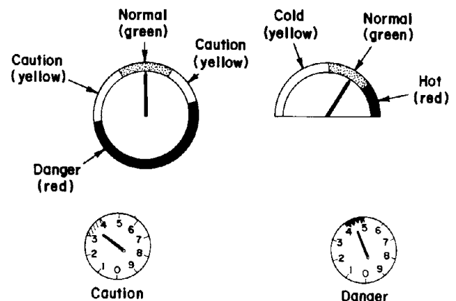
Figure 5-4.—Illustrations of coding methods for marking zones of instruments that are to be read qualitatively (12). (Courtesy of McGraw-Hill)
