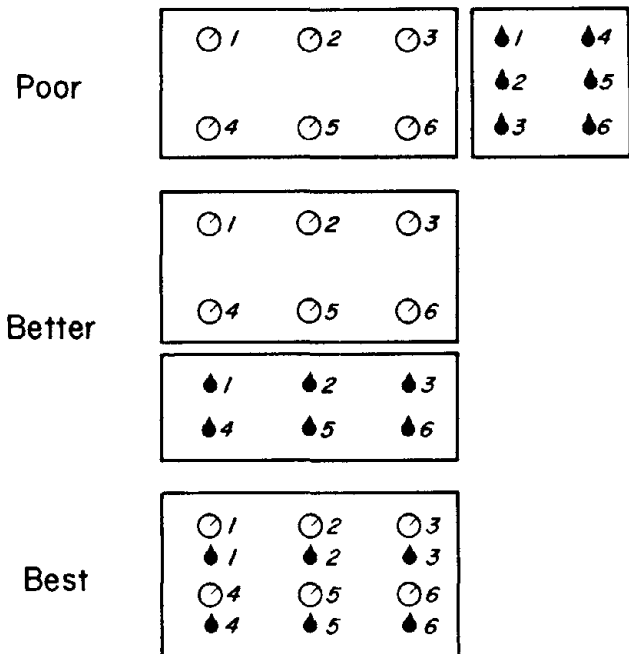
Figure 6-10.—Examples of spatial compatibility between a bank of controls and displays.
