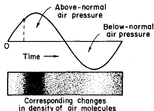
Figure 8-2.—Sine wave sound pressure wave showing one cycle with corresponding changes in air pressure.
