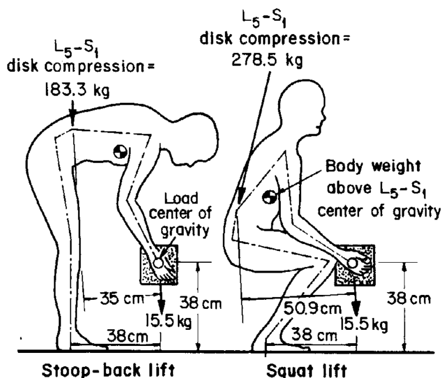
Figure 7-17.—Comparison of lower-back compression forces associated with stoop-back and squat methods of lifting a wide object (29). (Copyright 1974 by the American Institute of Industrial Engineers, and reprinted by permission)
