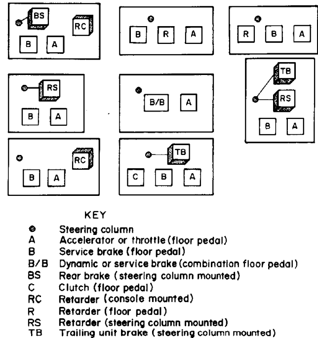
Figure 6-12.—Brake, clutch, and throttle control placement on eight 120-st-capacity and smaller haulage trucks (adapted from 6).
