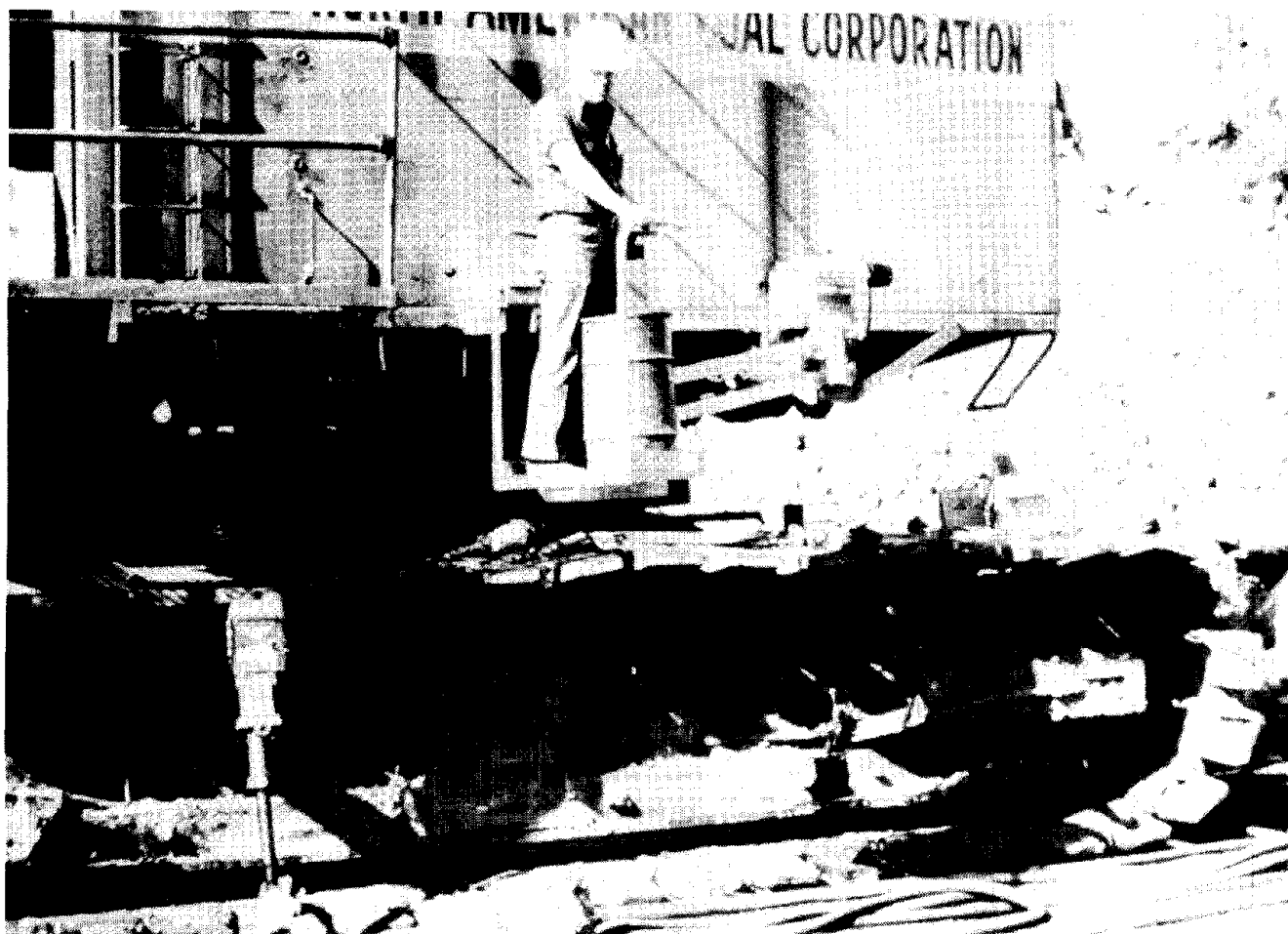
Figure 6-39.—Bureau-sponsored hydraulic “power” step for egress and ingress from tractors, dozers, and shovels (18).
