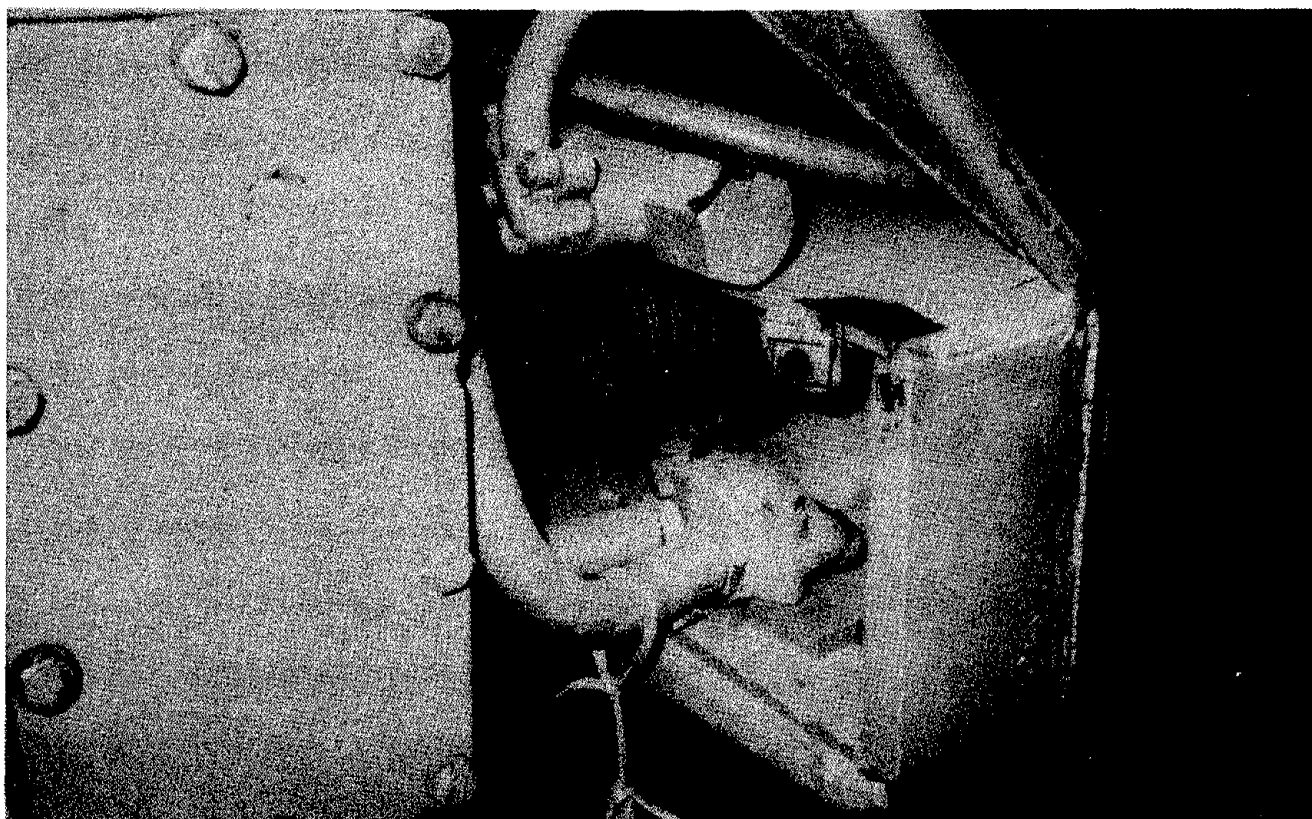
Figure 2.—Inadequate access openings prevent visual inspection or the use of proper tools for making repairs.
