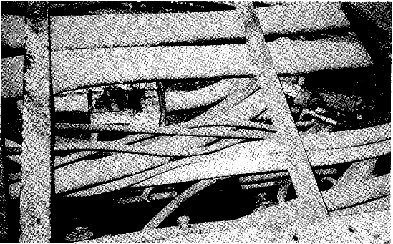
Figure 5.—The closely packed routing of hydraulic and electrical lines makes even simple hose repair jobs a major task.
