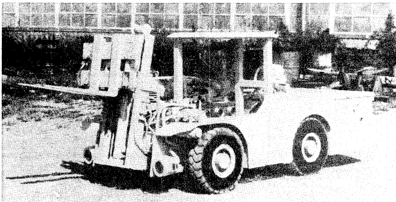
Figure 5.—Prototype battery-powered underground forklift.
