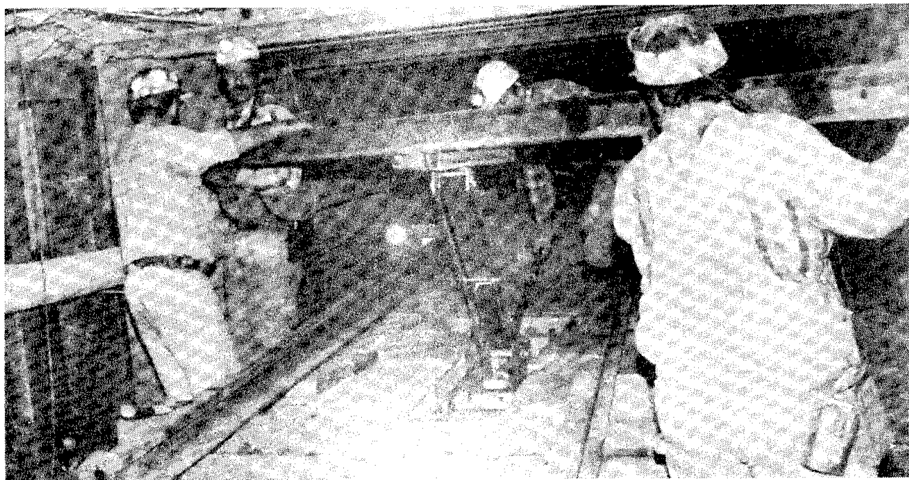
Figure 5.—Installation of a 15-ft section of rail (weighing 525 lb) in an eastern Ohio coal mine.
