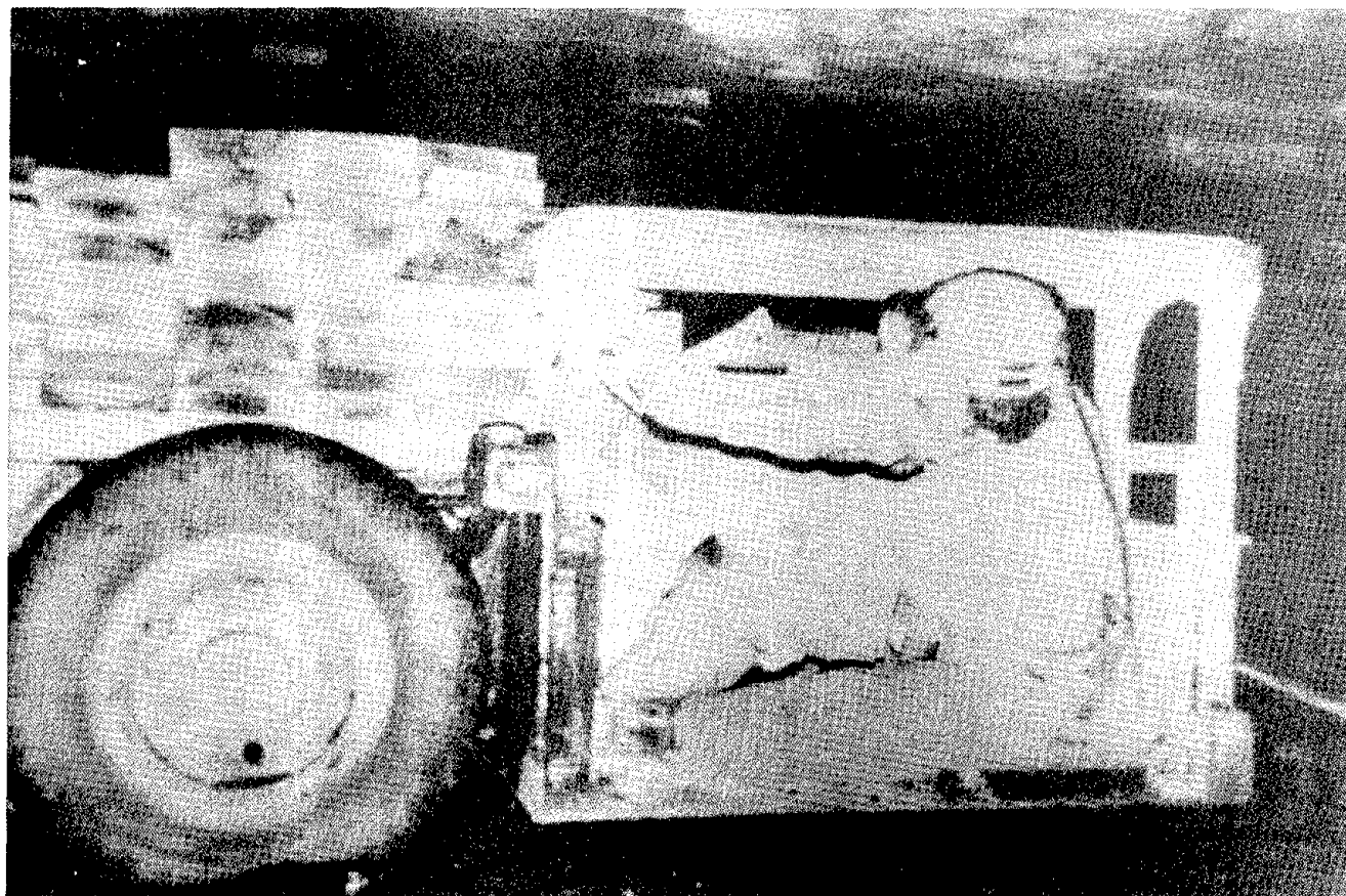
Figure 1.—Cramped operator stations and poor visibility often force miners to lean outside the safe confines of the cab.
