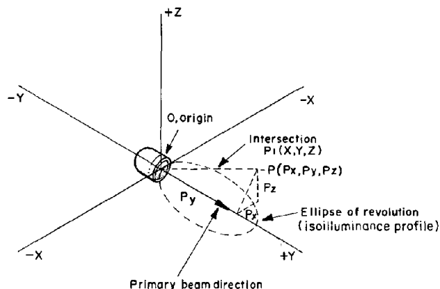
Figure A-4.—Isoilluminance profile model for headlamps: definition of ( X', Y' ) coordinate system.
