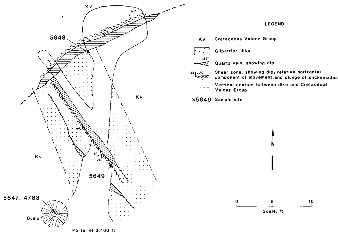
FIGURE 24.—Sample location map for upper level of Gilpatrick Dike Mine
