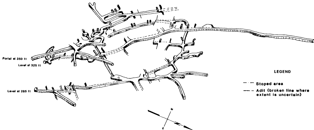
FIGURE 12.—Normal axonometric projection of accessible levels in Granite Mine.
