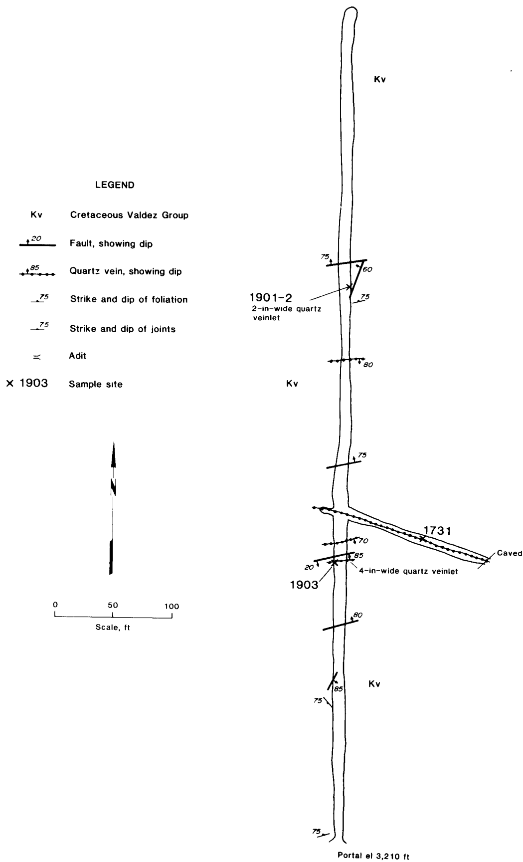
FIGURE 9.—Sample location map for 3,210-ft level of Gold King Mine.
