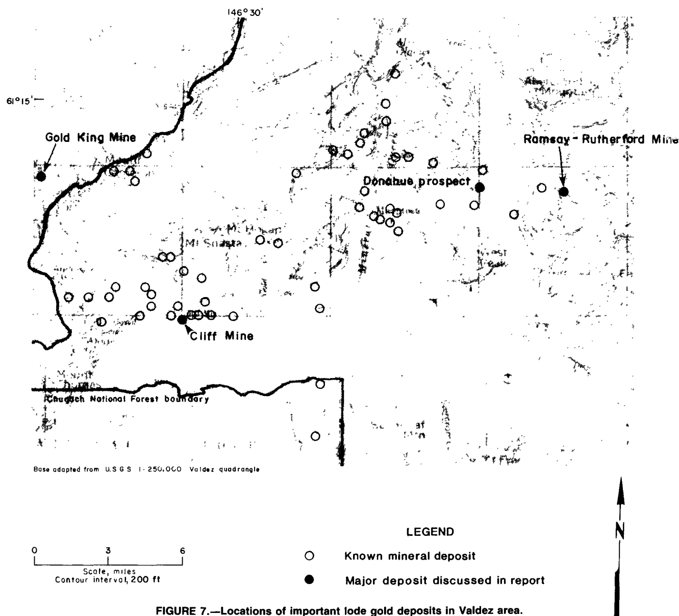
FIGURE 7.—Locations of important lode gold deposits in Valdez area.
