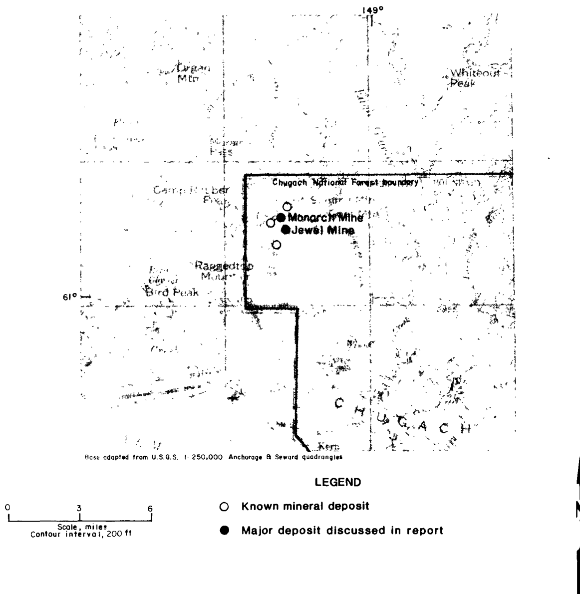
FIGURE 29.—Locations of important lode gold deposits in Girdwood area.
