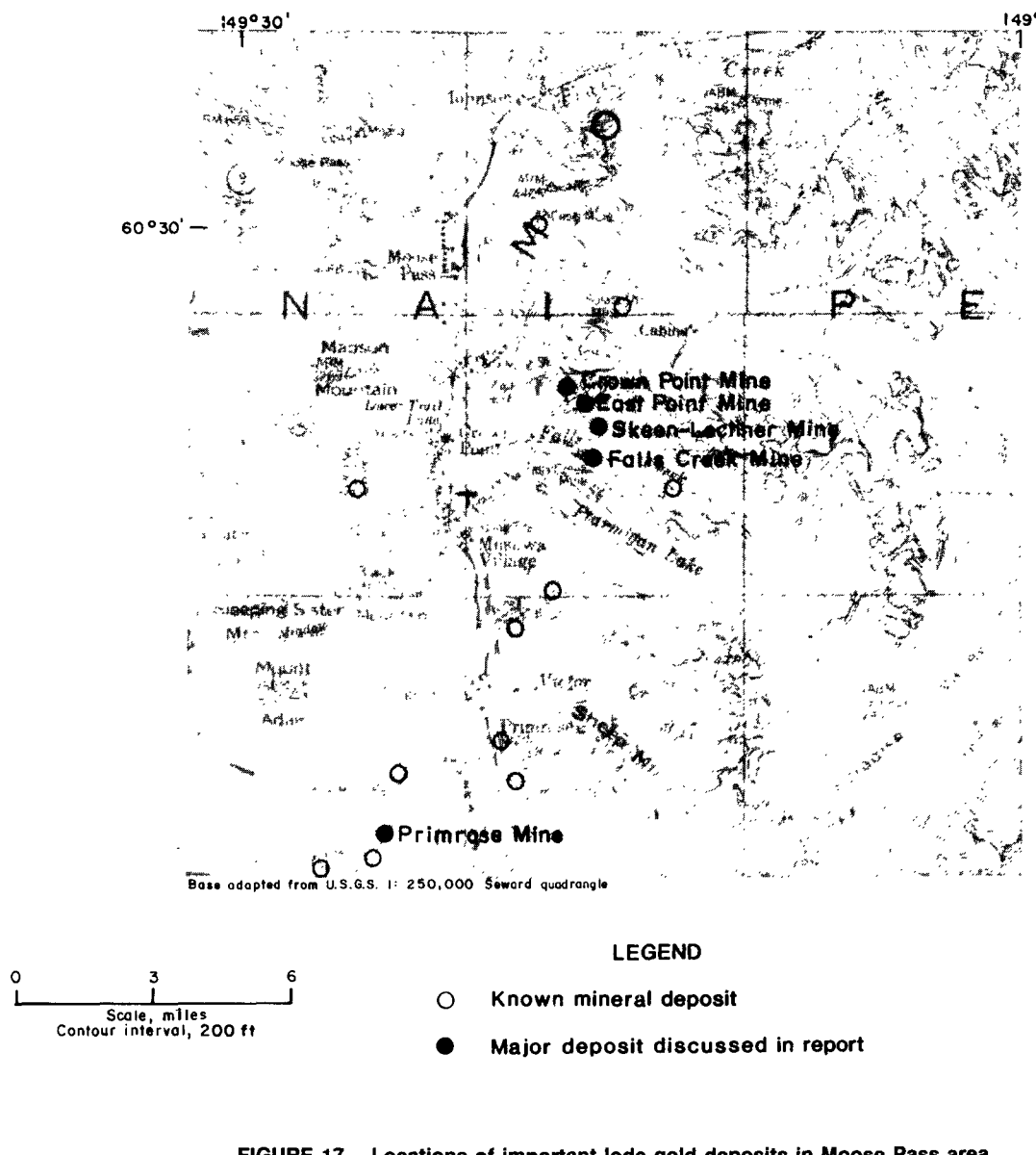
FIGURE 17.—Locations of important lode gold deposits in Moose Pass area.
