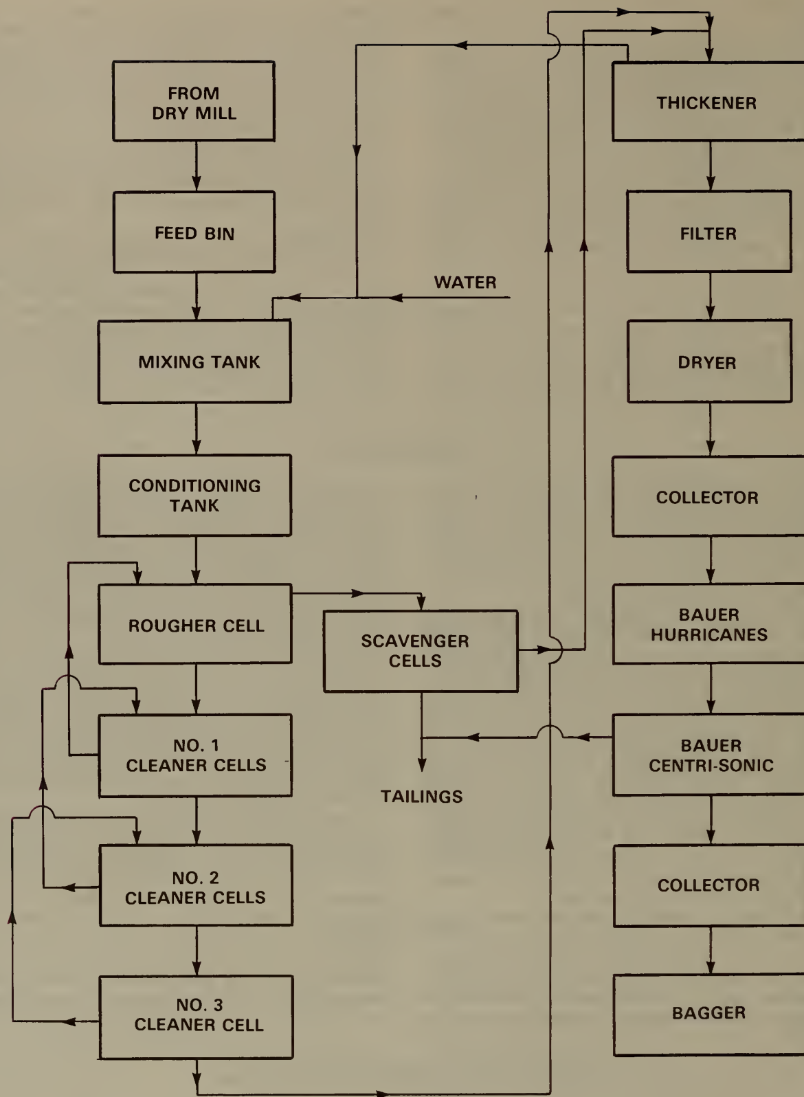
Figure 1.—Flowsheet for a talc flotation mill.
