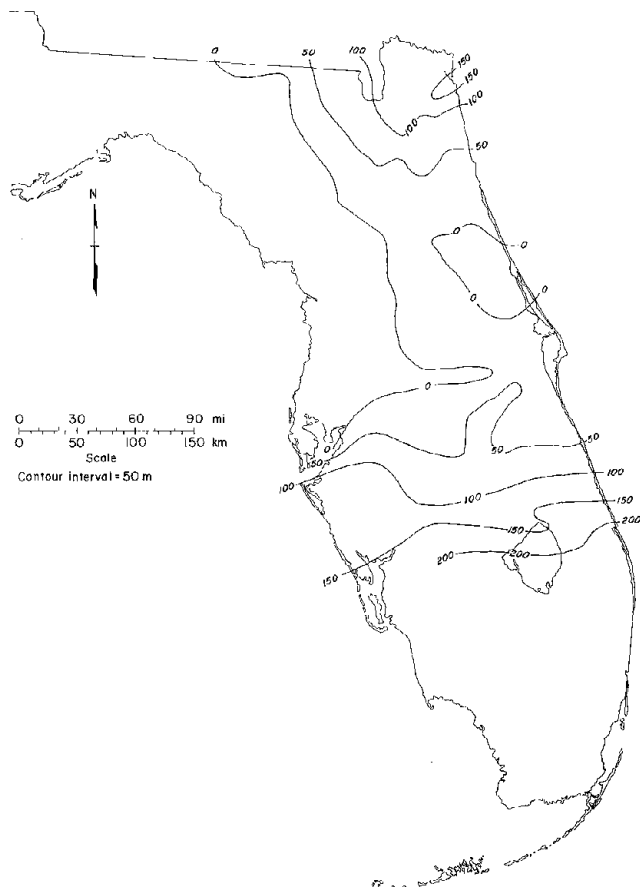
FIGURE 5. - Isopach map, Hawthorn Formation in Florida (modified from and courtesy of Florida Bureau of Geology, 1983).
