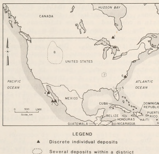
FIGURE 7. - Location map, North American deposits. 1, Cargill; 2, San Hilario (inferred only); 3, San Juan de la Costa; 4, Santo Domingo; 5, Florida; 6, North Carolina; 7, Tennessee; 8, Western United States (Idaho, Montana, Utah, Wyoming).
