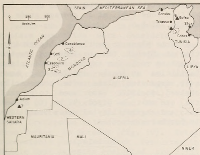
FIGURE 8. - Location map, north African deposits. 1, Djebel Onk; 2, Ganntour Plateau; 3, Meskala District; 4, Oulad Abdoun Plateau; 5, South Basin (Kef Eschfair, M'Dilla, Metloui, M'Rata, Moulares, Redeyef, and Sehib); 6, Kalaa Khasba; 7, Bou Craa.
