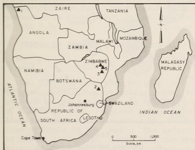
FIGURE 15. - Location map, southern African deposits. 1, Lacunga River; 2, Palabora; 3, Chishanya (inferred only); 4, Dorowa; 5, Shawa (inferred only).
