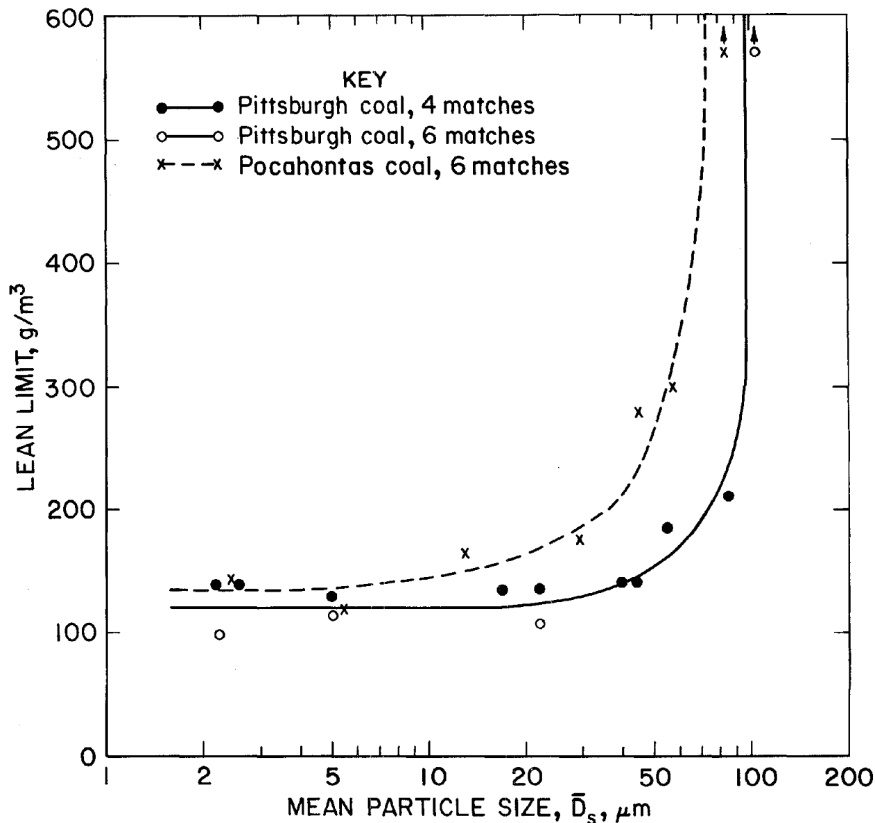
FIGURE 26. • Lean flammable limit for Pittsburgh and Pocahontas coals as a function of particle size.
