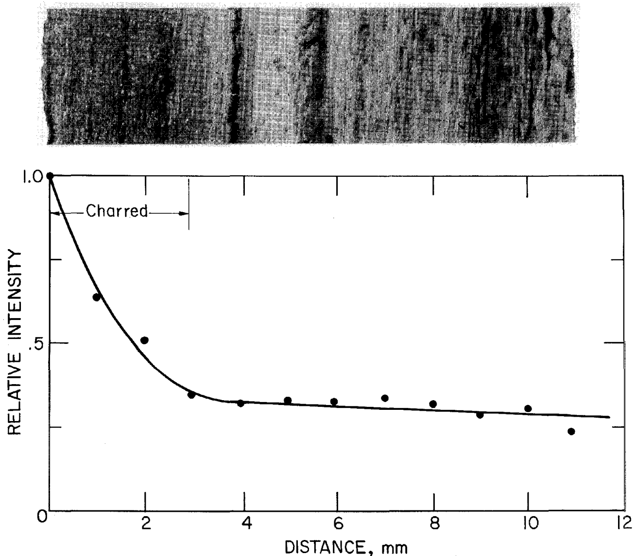
FIGURE 52. - Relative distribution of phosphorus as a function of distance from the surface, in chemically treated oak timber after charring.
