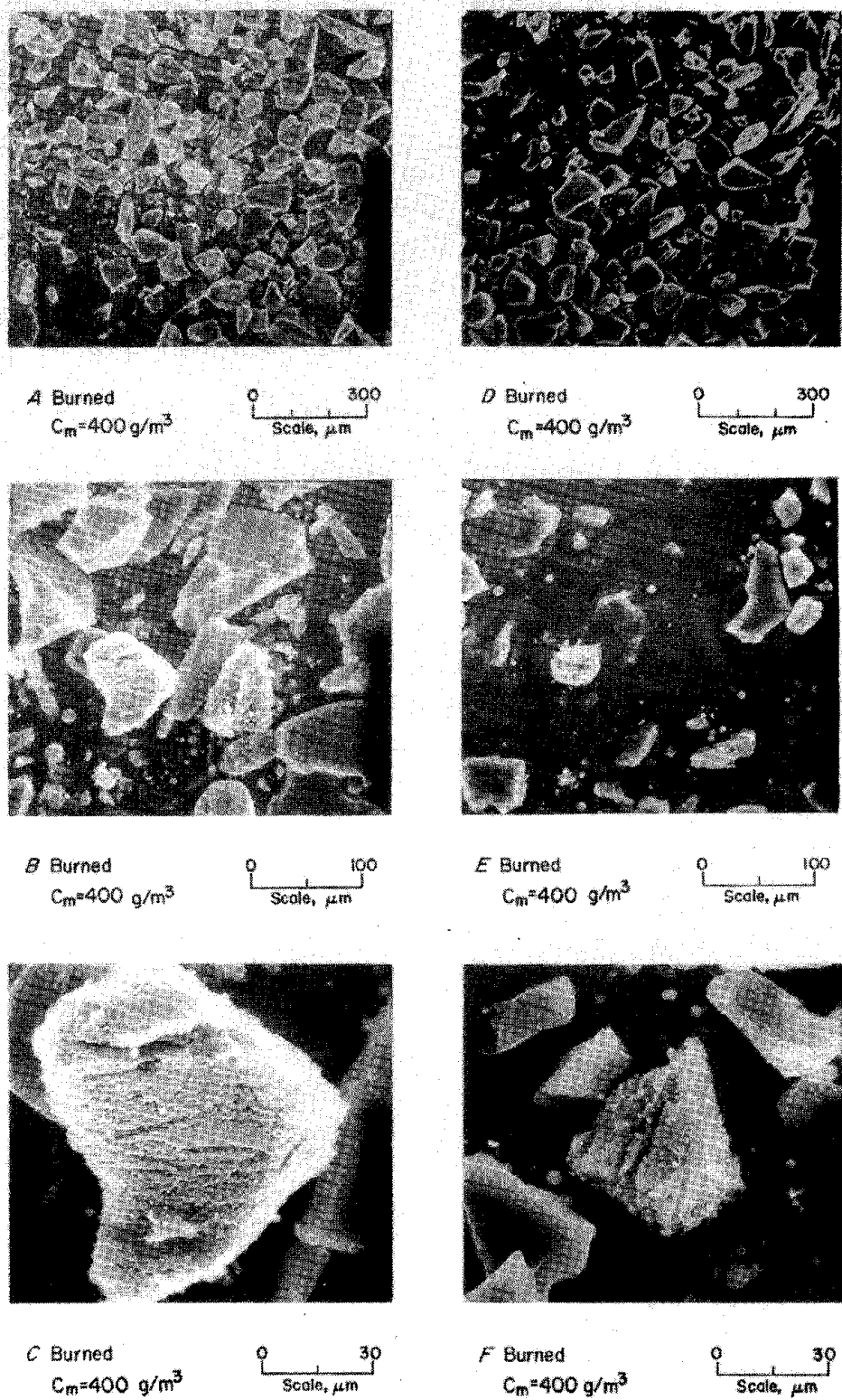
FIGURE 31. - Anthracite dust, burned in 50% O 2 .
