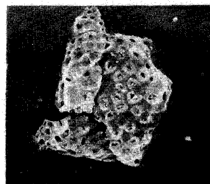
F Heated, T=600^{\circ}\text{C} C_m=260 \text{ g/m}^3 0 30 Scale, \mu\text{m}
