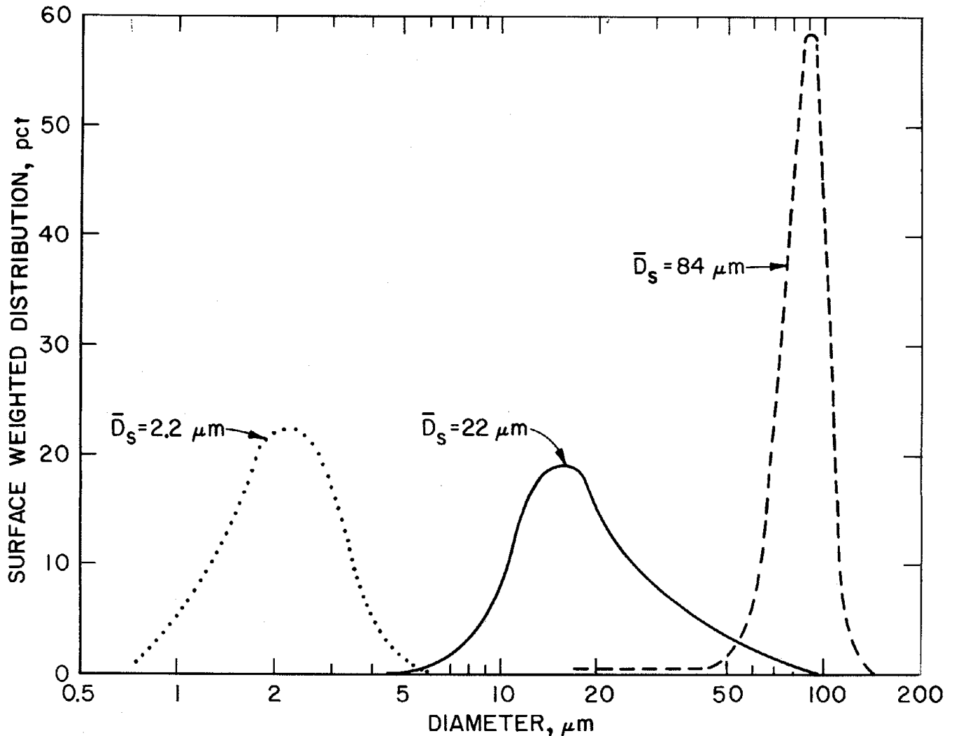
FIGURE 9. - Coulter Counter size distributions of three classified Pittsburgh coal dusts.
