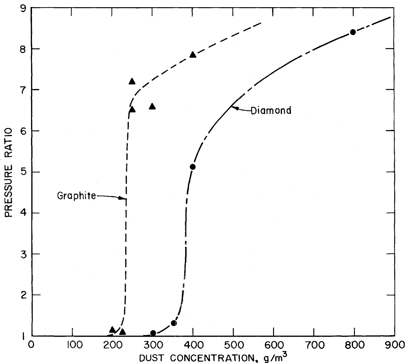
FIGURE 32. - Flammability data from the 8-L chamber for graphite and diamond dust in 50% O 2 .
