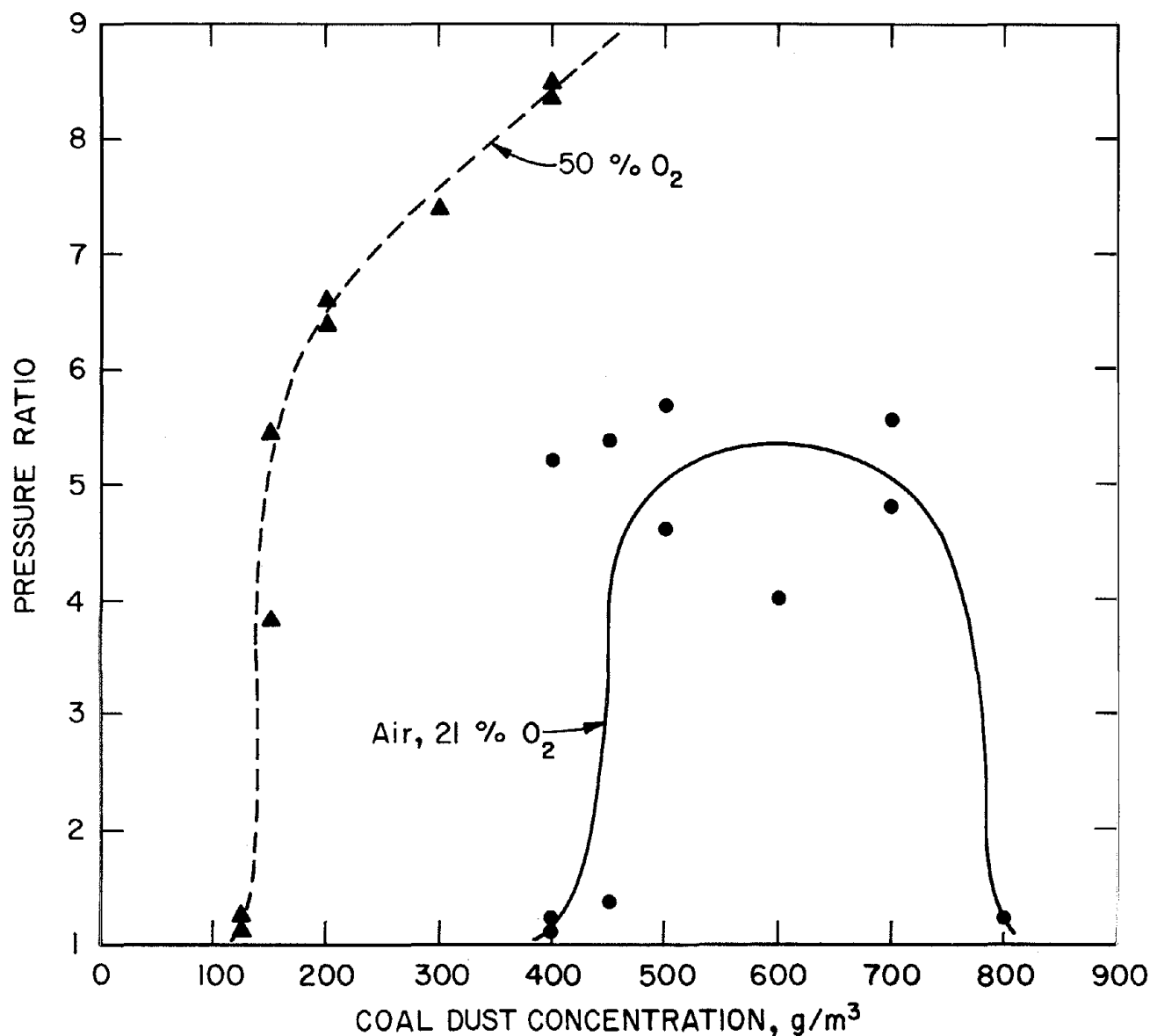
FIGURE 29. • Flammability data from the 8-L chamber for anthracite in air and in 50% O 2 .
