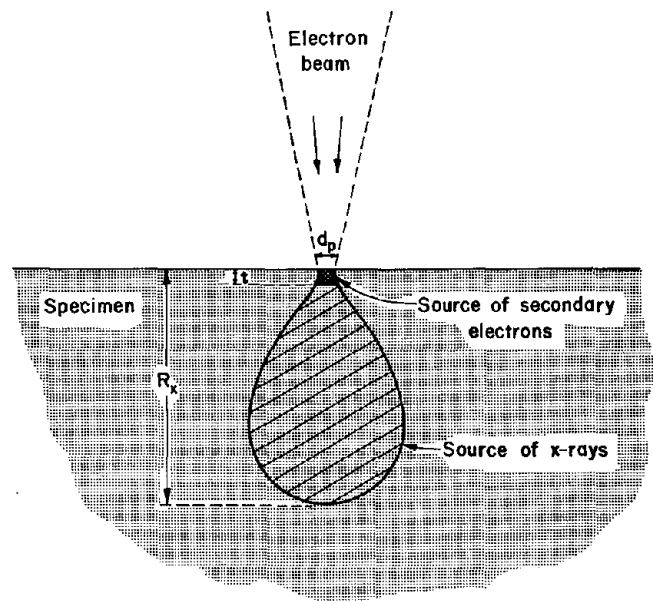
FIGURE 2. - Electron beam interaction region with specimen.
