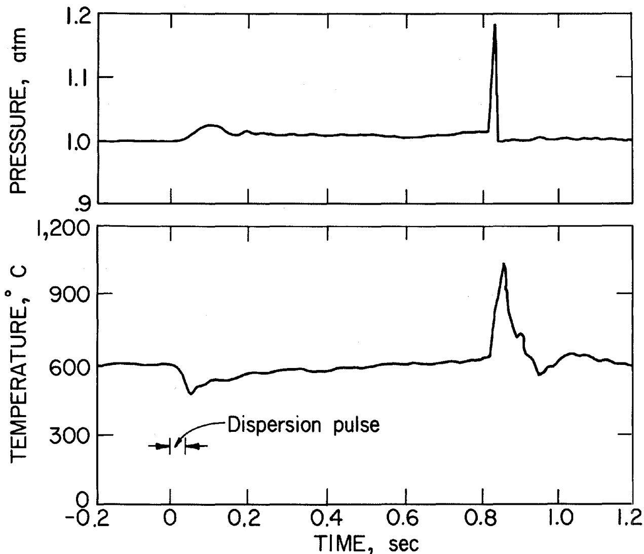
FIGURE 43. - Pressure and thermocouple recorder traces from an explosion in the 1.2-L furnace.
