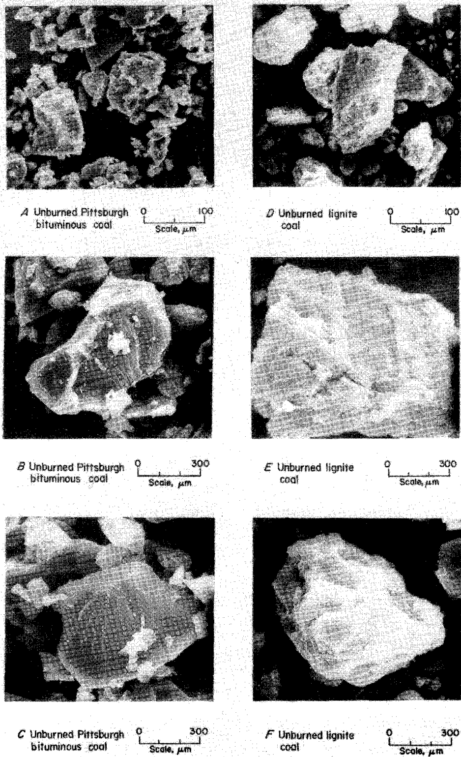
FIGURE 50. - Comparison of surface characteristics of bituminous and lignite coals.
