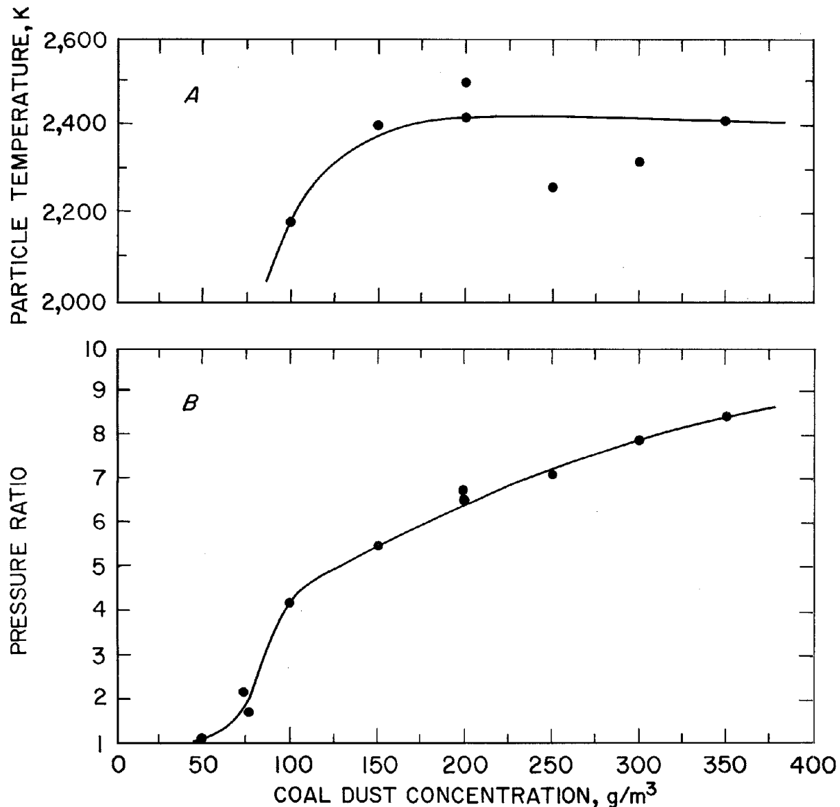
FIGURE 17. - Flammability data from the 8-L chamber for 22- \mu\text{m} Pittsburgh coal dust in 50% \text{O}_2 .
