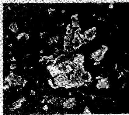
D Heated, T=600^{\circ}\text{C} C_m=260 \text{ g/m}^3 0 100 Scale, \mu\text{m}
