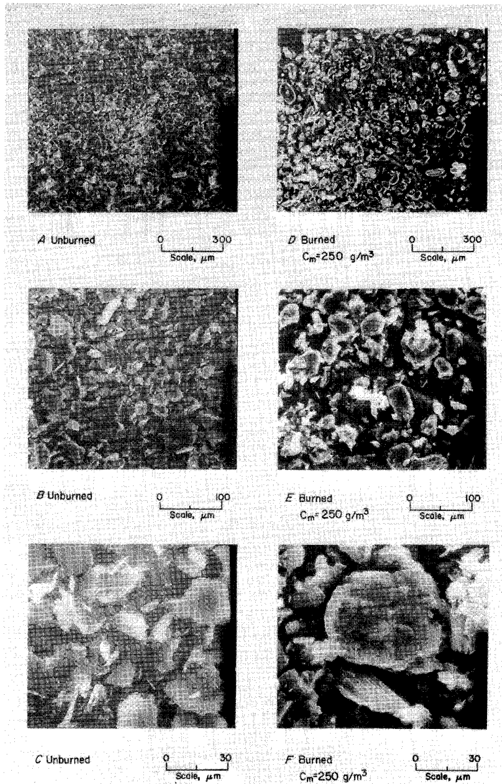
FIGURE 33. - Graphite dust (4- \mu\text{m} ), unburned and burned in 50% O 2 .
