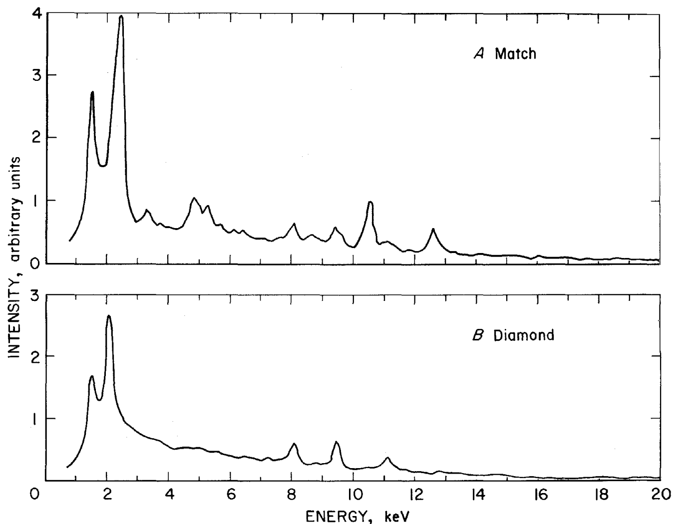
FIGURE 35. - X-ray spectra of diamond and match particles.
