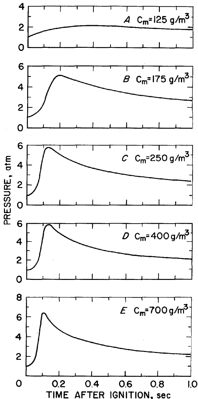
FIGURE 11. - Pressure traces for explosions of 22\text{-}\mu\text{m} Pittsburgh coal dust in air.
