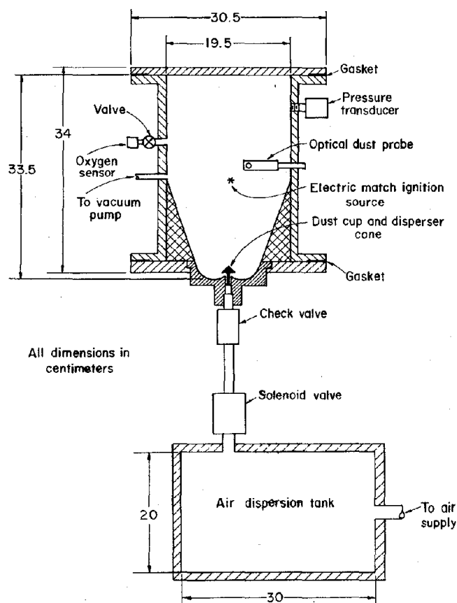
FIGURE 8. - 8-L flammability chamber.
