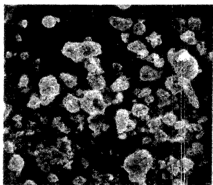
B Burned C_m = 700 \text{ g/m}^3 0 100 Scale, \mu\text{m}
