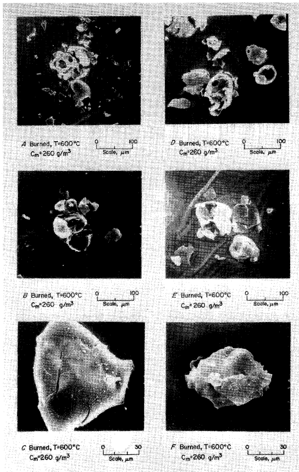
FIGURE 47. - Pittsburgh coal dust (55-μm) after an explosion in the 1.2-L furnace.
