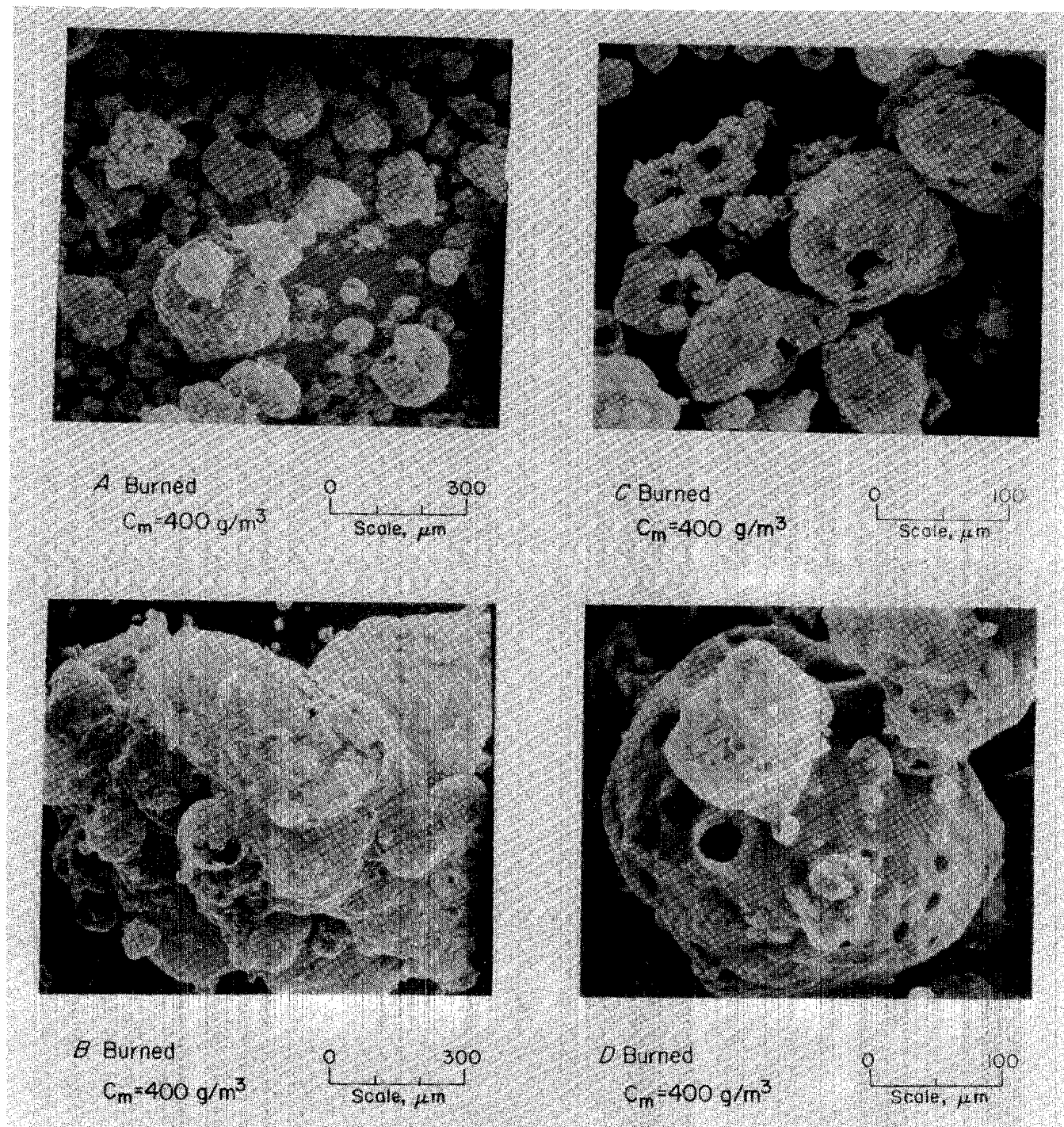
FIGURE 14. - Pittsburgh coal dust (22-μm), high concentration burned in air.
