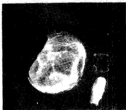
B Heated, T=600^{\circ}\text{C} C_m=260 \text{ g/m}^3 0 30 Scale, \mu\text{m}
