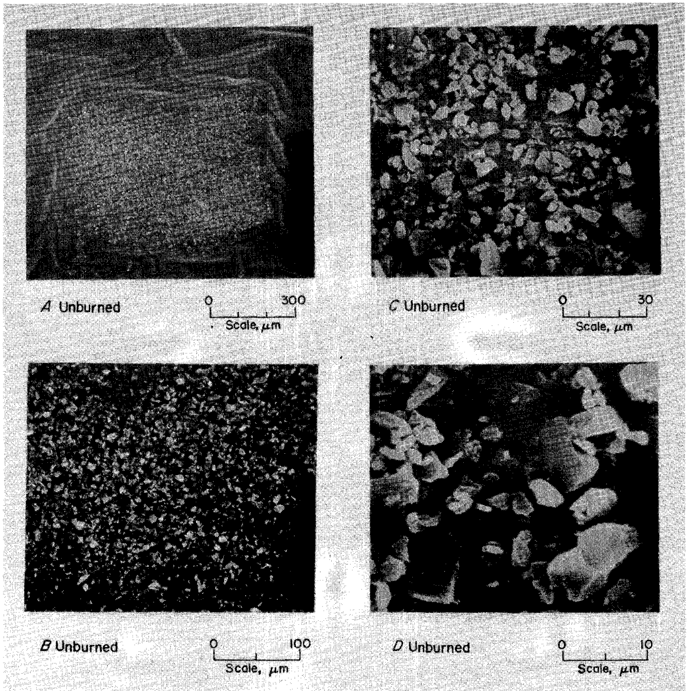
FIGURE 22. • Unburned Pittsburgh coal dust (2- \mu\text{m} ).
