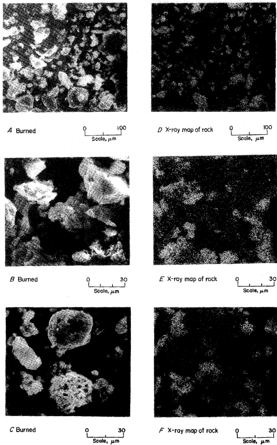
FIGURE 41. - Pittsburgh coal and rock dust (60% I), postexplosion sample from the Bruceton Experimental Mine. X-ray maps made using the Ca line.
