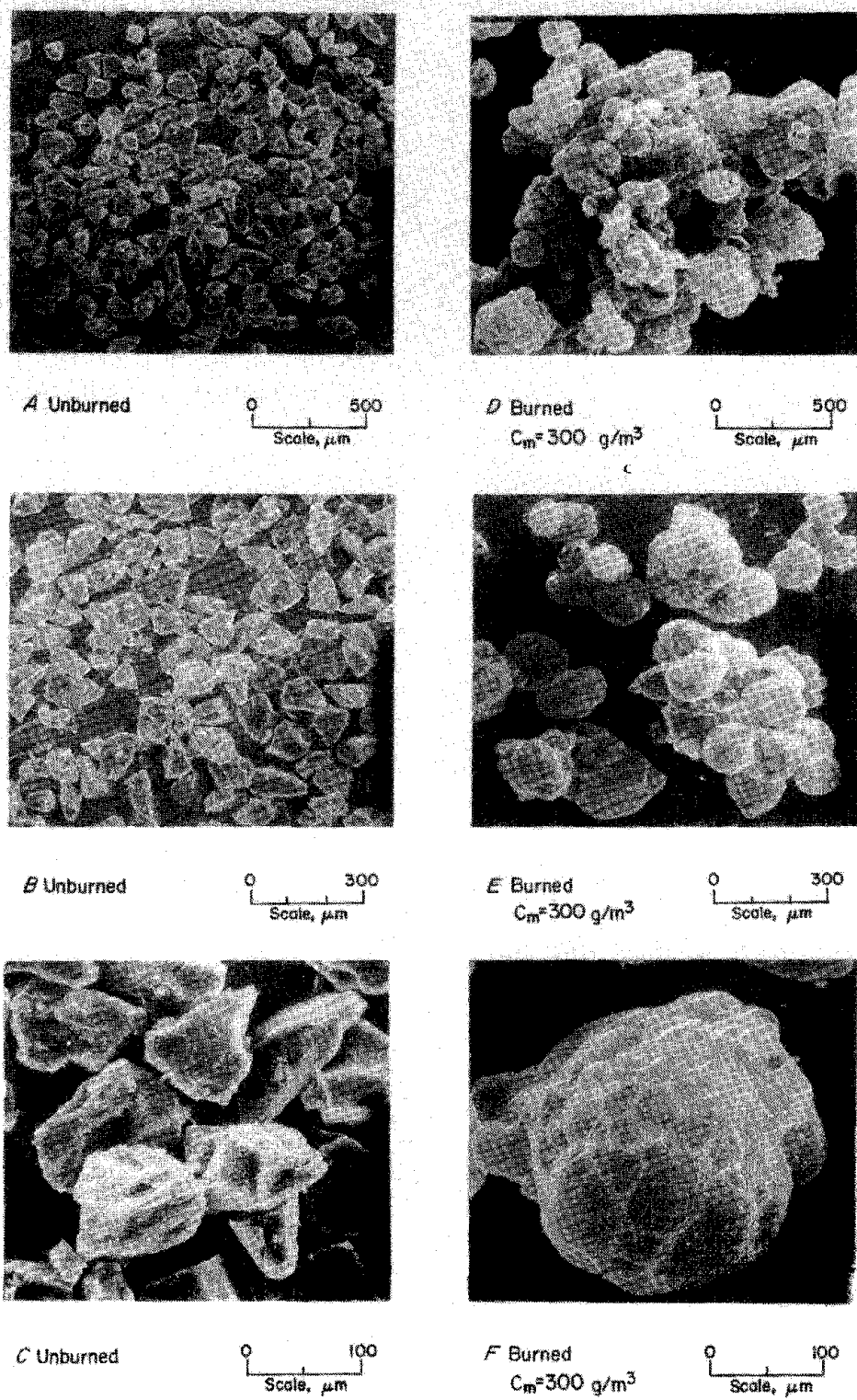
FIGURE 25. - Pittsburgh coal dust (84-μm), unburned and burned in air.
