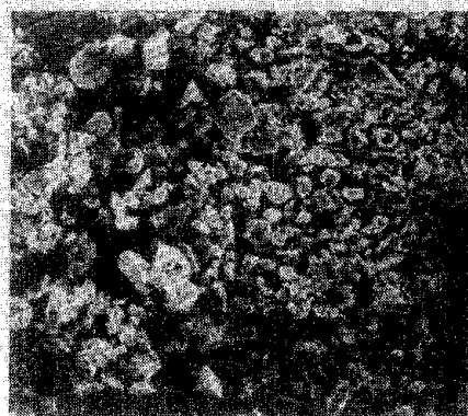
A Burned Coal C_m = 400 \text{ g/m}^3 Scale, \mu\text{m}
