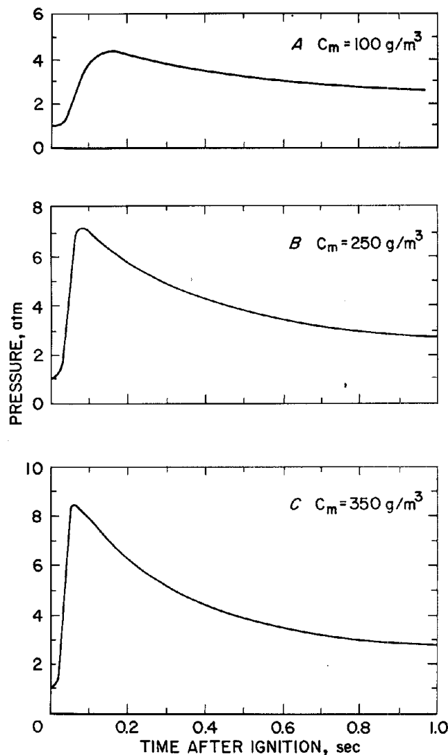
FIGURE 18. - Pressure traces for explosions of 22- \mu\text{m} Pittsburgh coal dust in 50% \text{O}_2 .
