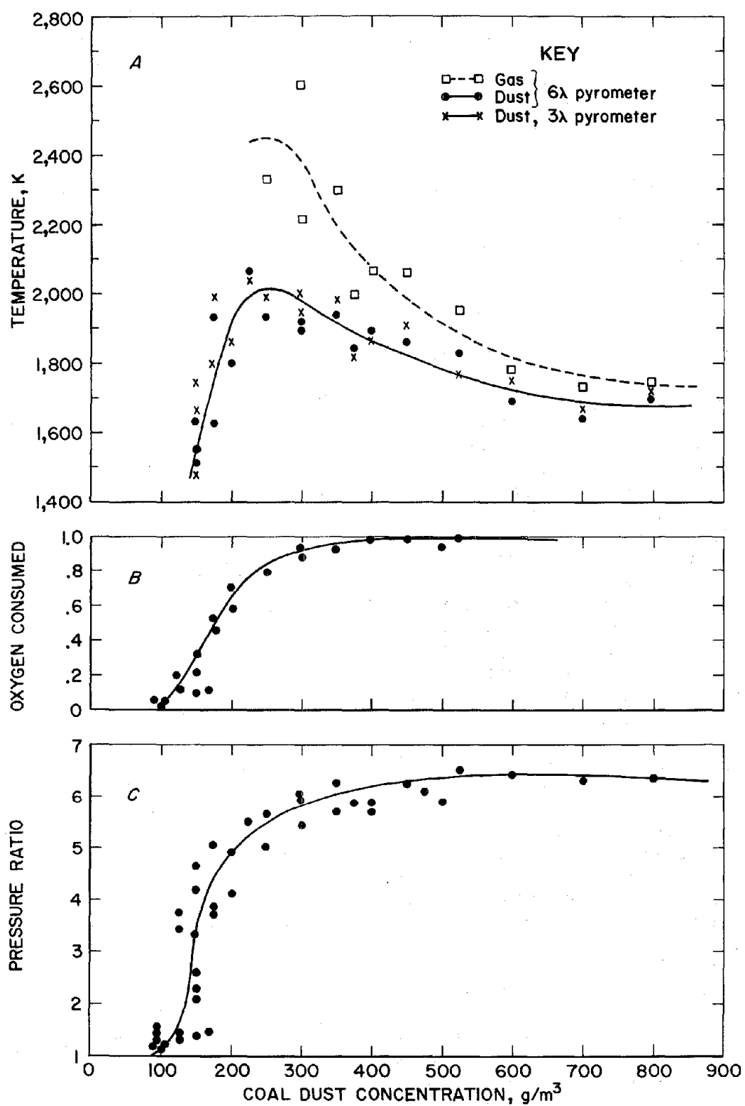
FIGURE 10. - 8-L chamber flammability data for 22- \mu\text{m} Pittsburgh coal dust in air.
