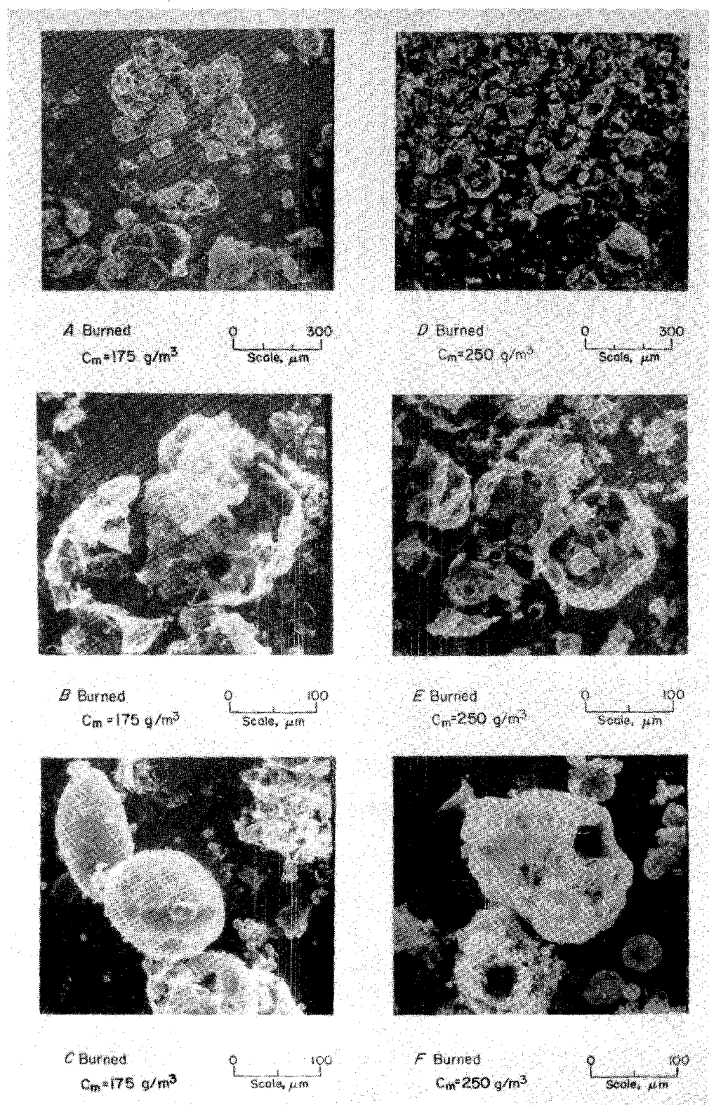
FIGURE 13. - Pittsburgh coal dust (22- \mu\text{m} ), intermediate concentrations burned in air.
