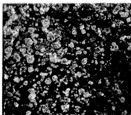
A Burned C_m = 700 \text{ g/m}^3 0 300 Scale, \mu\text{m}
