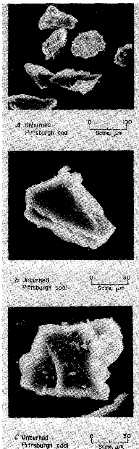
FIGURE 45. - Unburned Pittsburgh coal dust (55- \mu\text{m} ).
