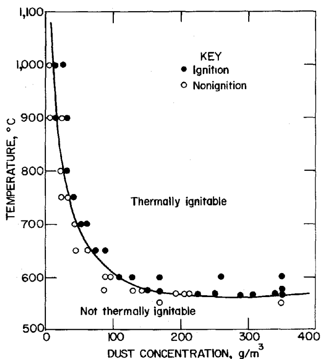
FIGURE 44. - Dust cloud thermal ignition data from the 1.2-L furnace for 55- \mu m Pittsburgh coal in air.
