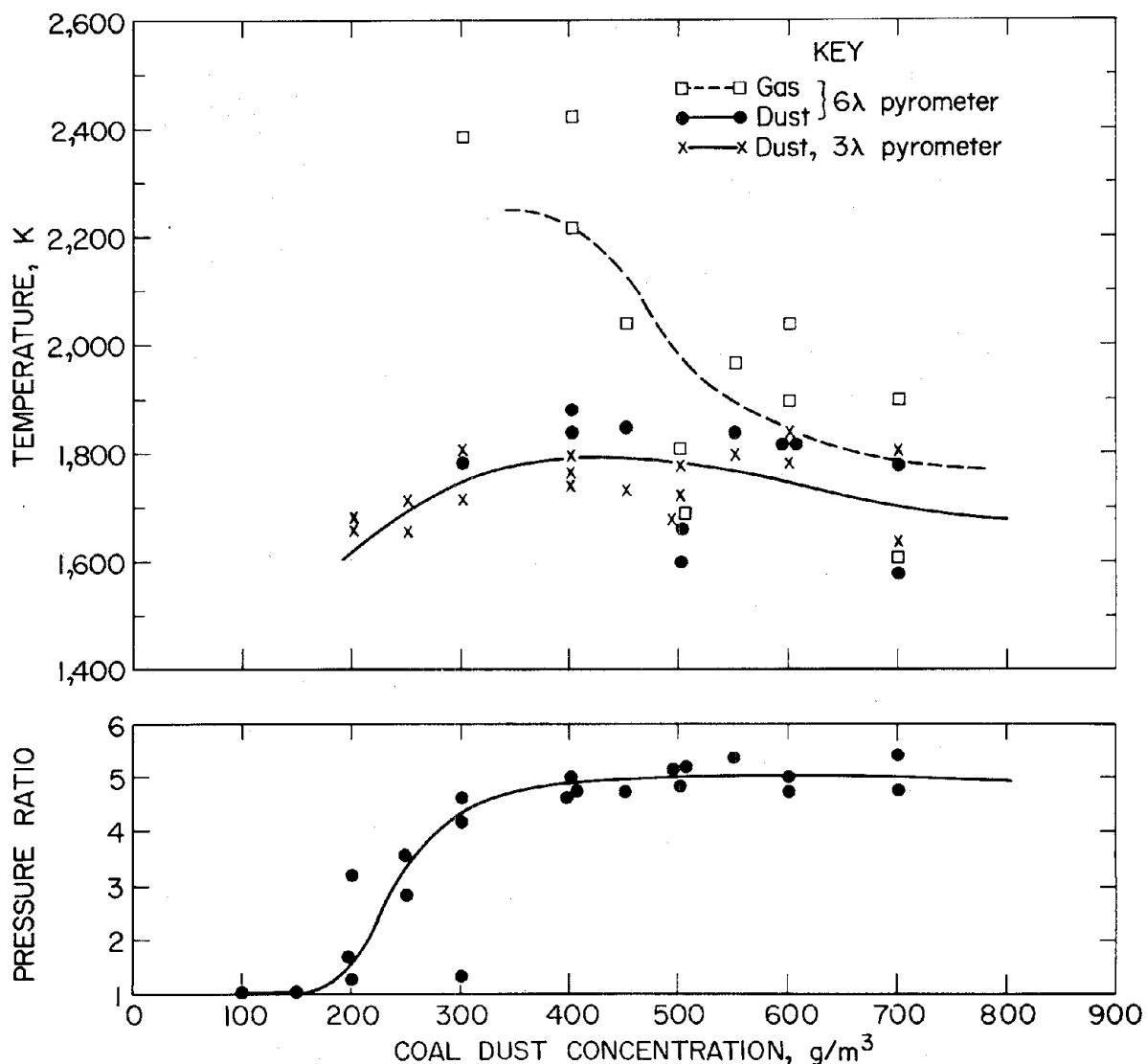
FIGURE 24. • Flammability data from the 8-L chamber for 84- \mu m Pittsburgh coal dust in air.
