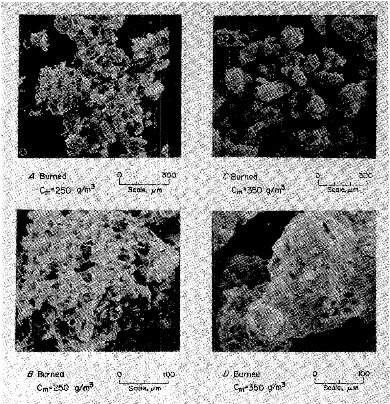
FIGURE 20. - Pittsburgh coal dust (22-μm), burned in 50% O 2 .
