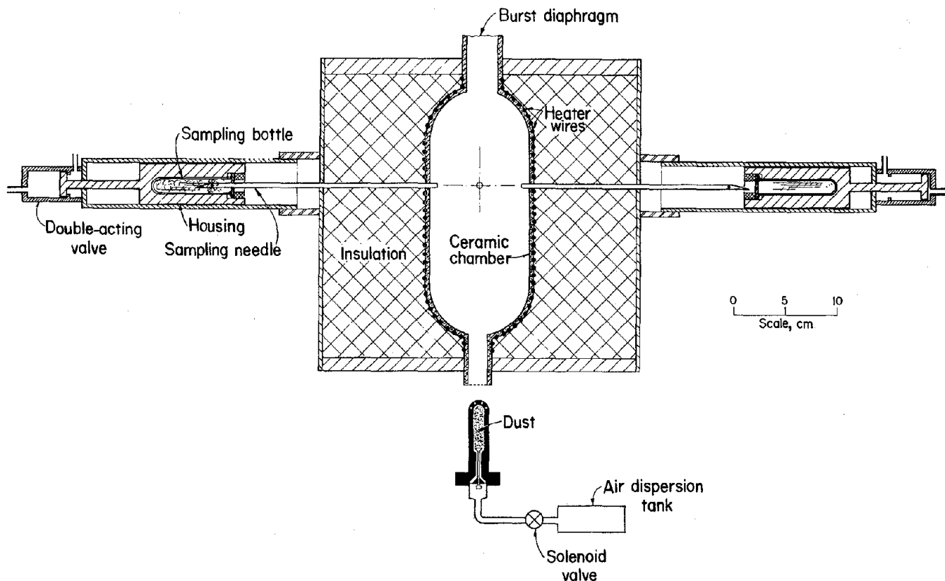
FIGURE 42. - 1.2-L furnace and rapid sampling system (8).
