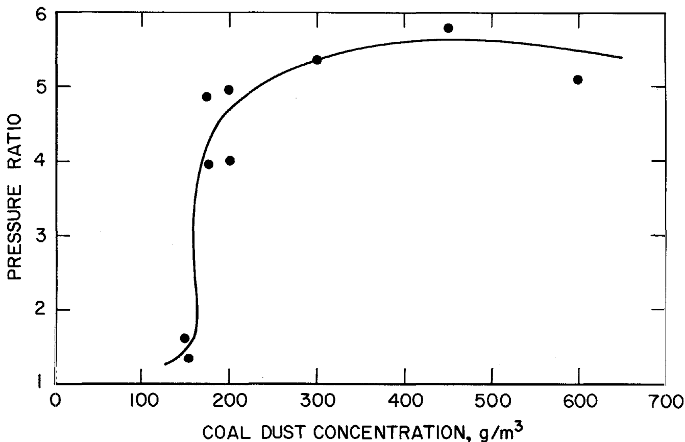
FIGURE 27. - Flammability data from the 8-L chamber for 13- \mu m Pocahontas coal dust in air.
