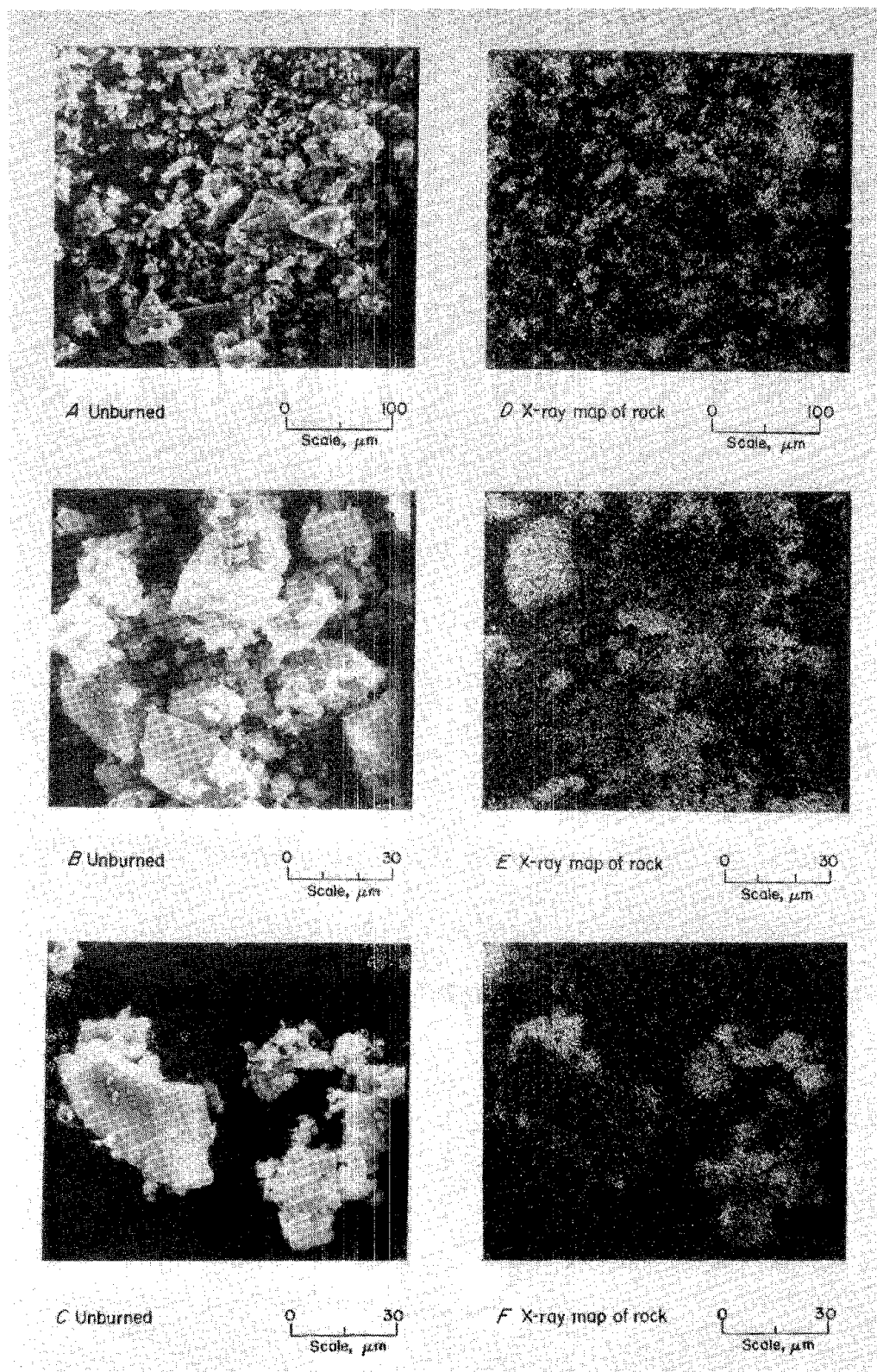
FIGURE 40. - Unburned Pittsburgh coal and rock dust mixture (60% I). X-ray maps made using the Ca line.
