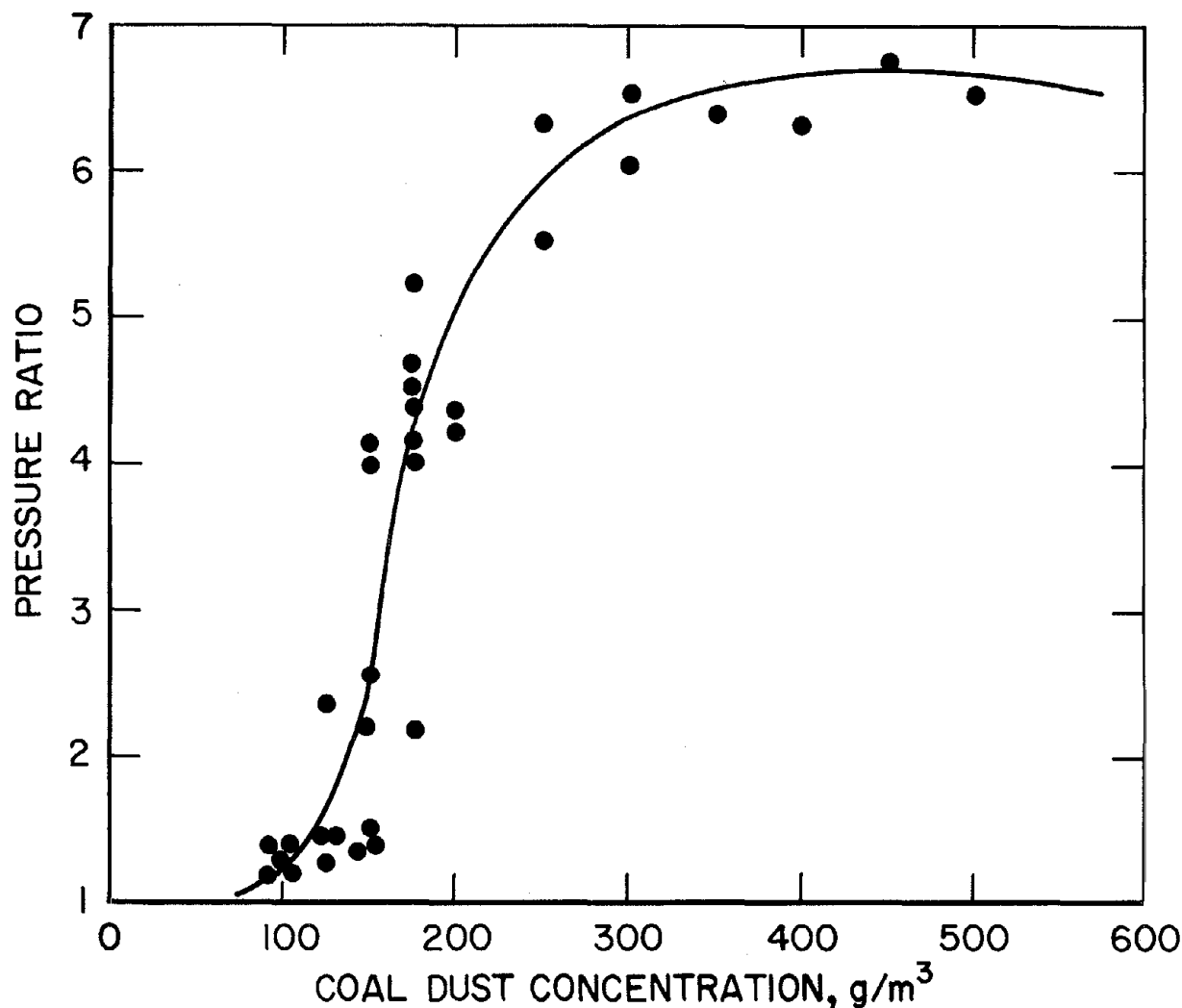
FIGURE 21. • Flammability data from the 8-L chamber for 2- \mu m Pittsburgh coal dust in air.
