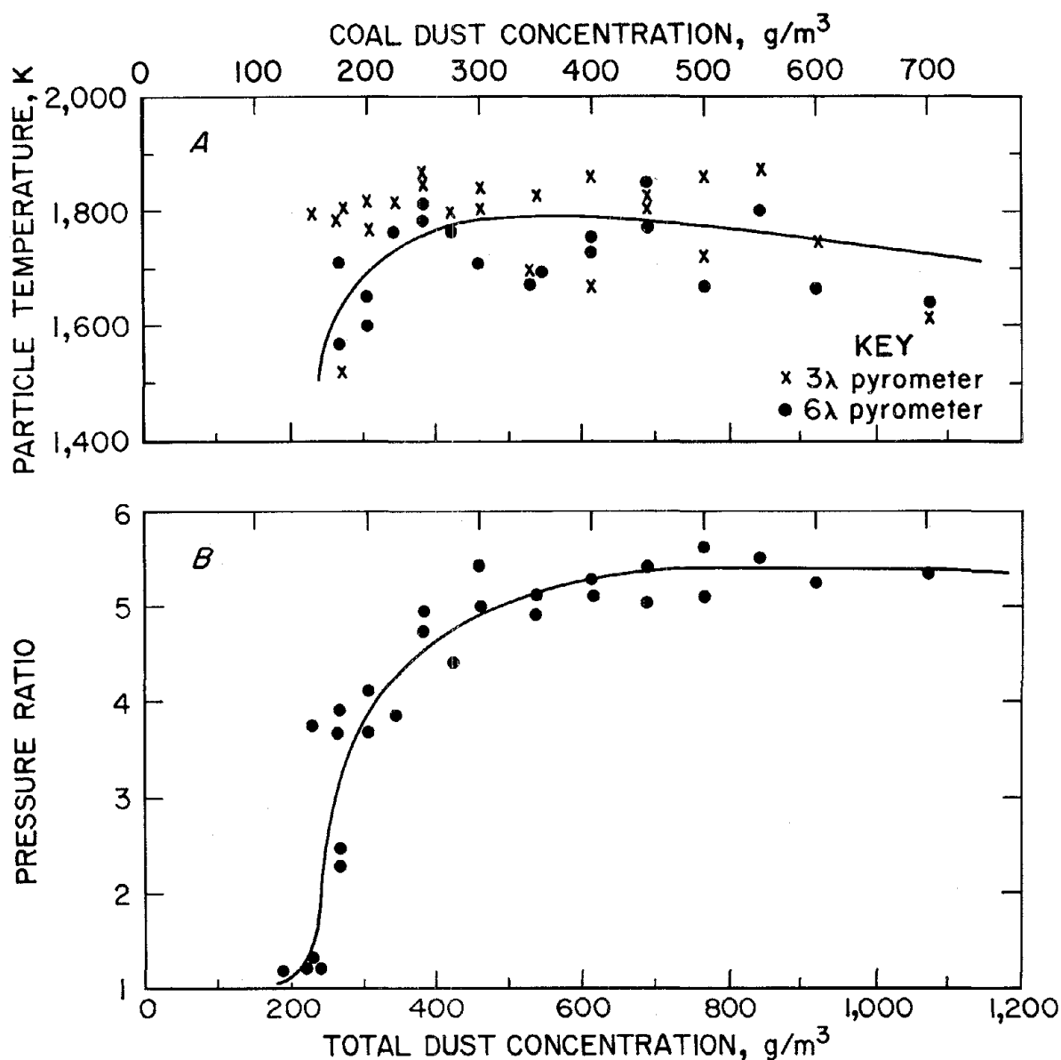
FIGURE 36. - Flammability data from the 8-L chamber for a Pittsburgh coal and rock dust mixture (40% l).
