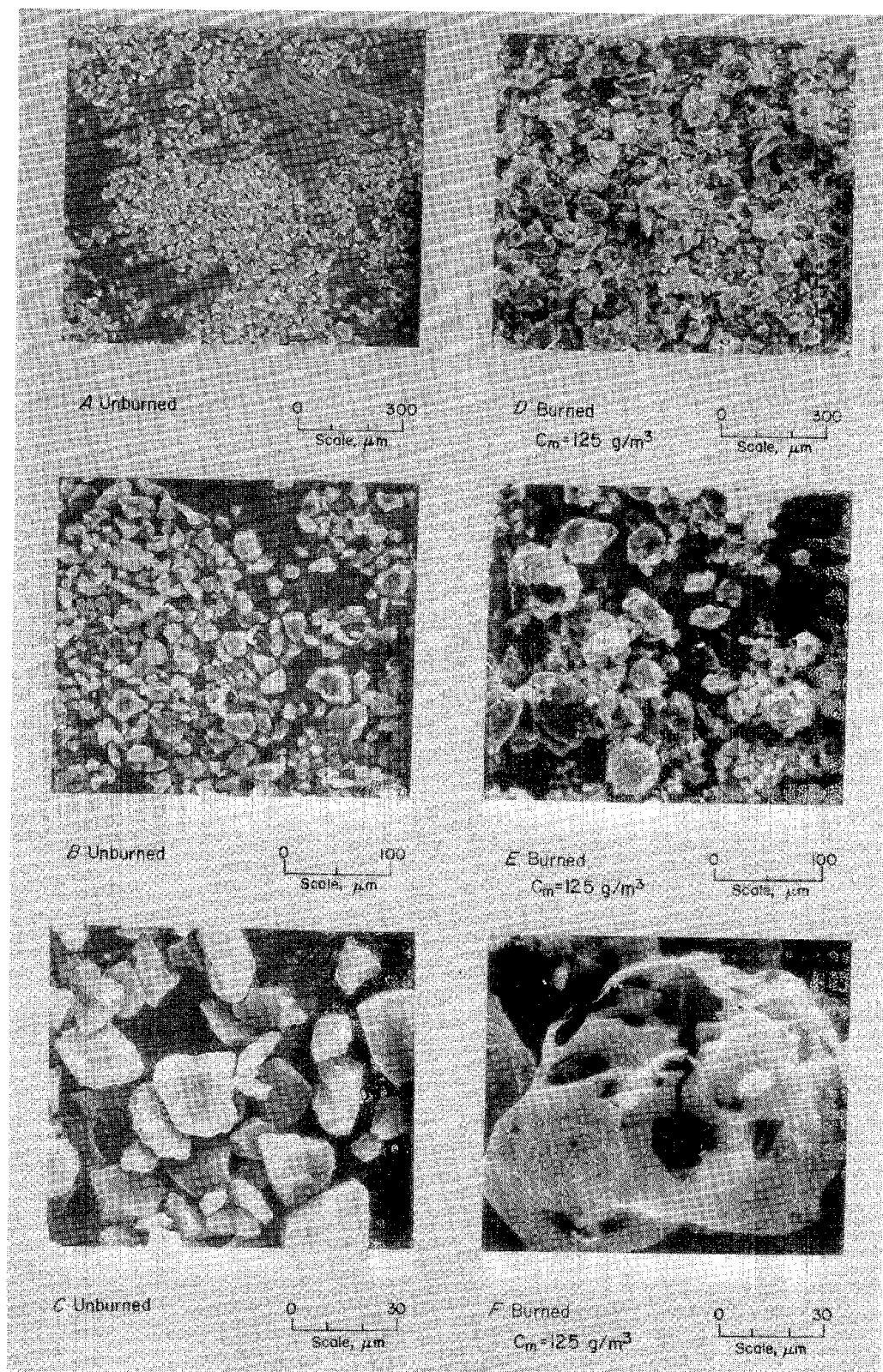
FIGURE 12. - Pittsburgh coal dust (22- \mu\text{m} ), unburned and a low concentration burned in air.
