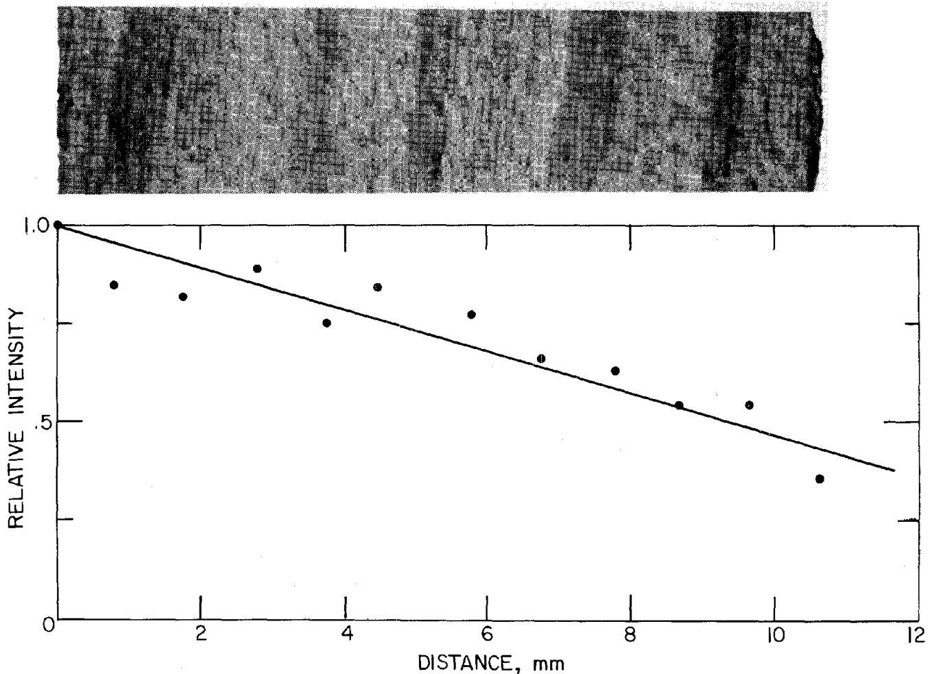
FIGURE 51. - Relative distribution of phosphorus as a function of distance from the surface, in oak timber chemically treated with NCX inhibitor.
