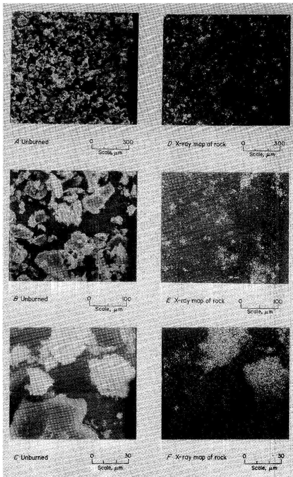
FIGURE 37. - Unburned Pittsburgh coal and rock dust mixture (40% I). X-ray maps made using the Ca line.
