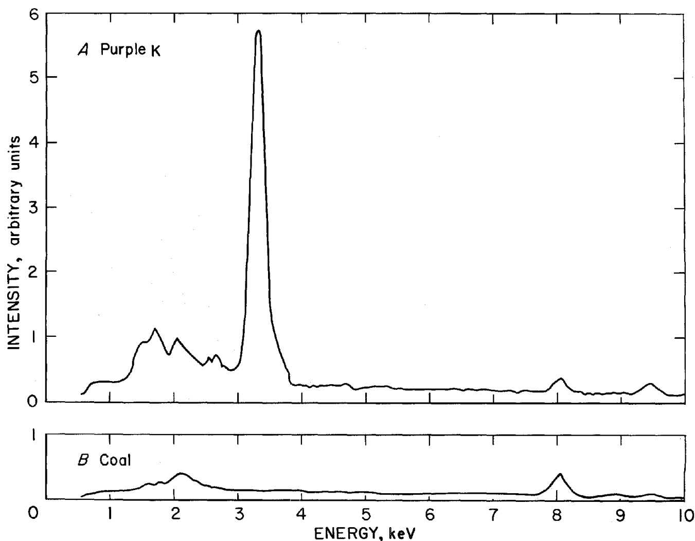
FIGURE 6. - X-ray spectra of coal and Purple K dust.
