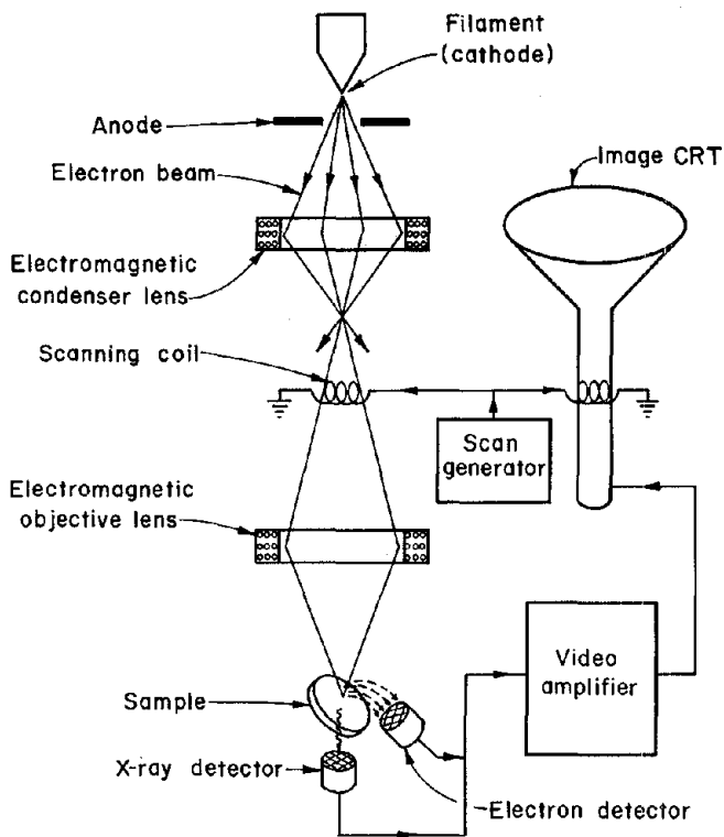
FIGURE 1. - Schematic of scanning electron microscope.
