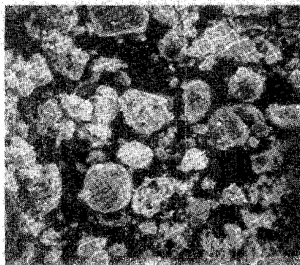
B Burned Coal C_m = 400 \text{ g/m}^3 Scale, \mu\text{m}
