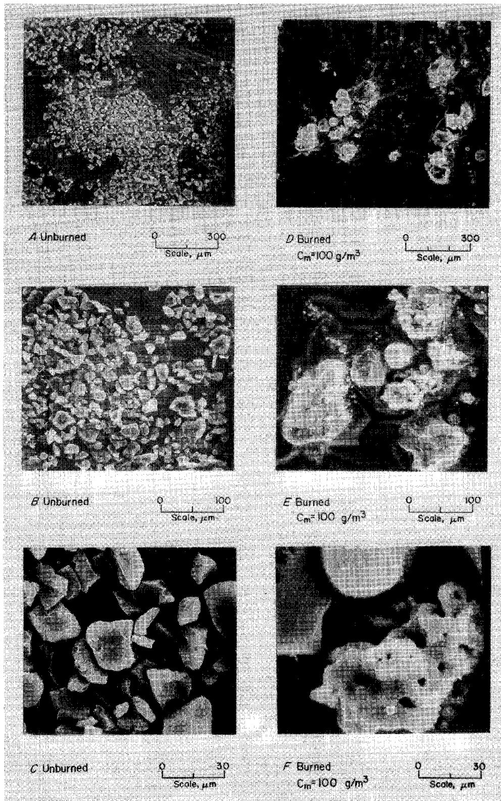
FIGURE 19. - Pittsburgh coal dust (22- \mu\text{m} ), unburned and burned in 50% \text{O}_2 .
