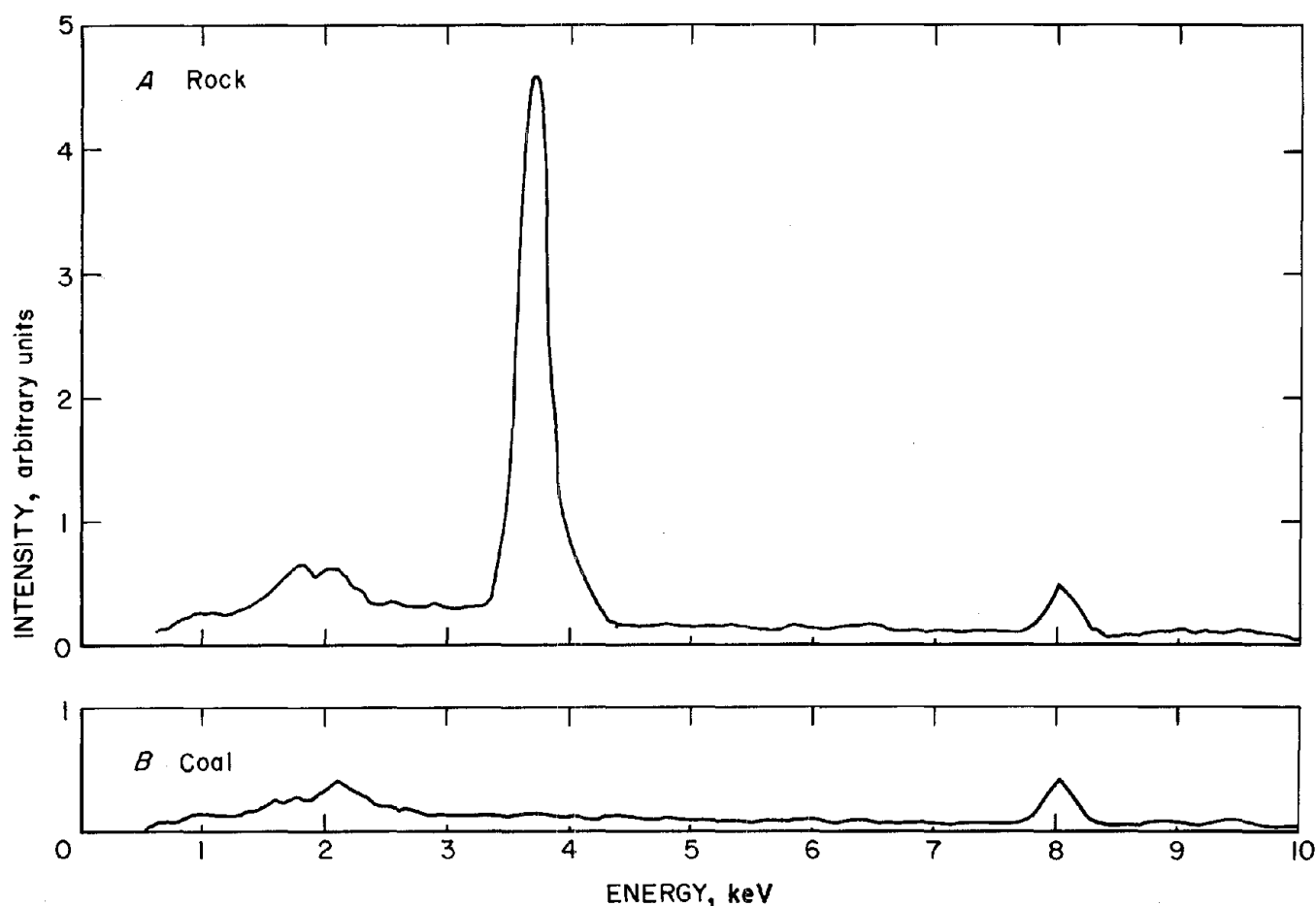
FIGURE 38. - X-ray spectra of limestone rock and coal particles.
