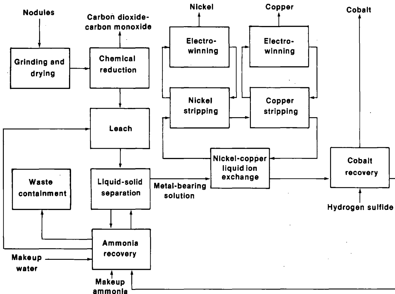
Figure 1.—Gas reduction and ammoniacal leach process.
