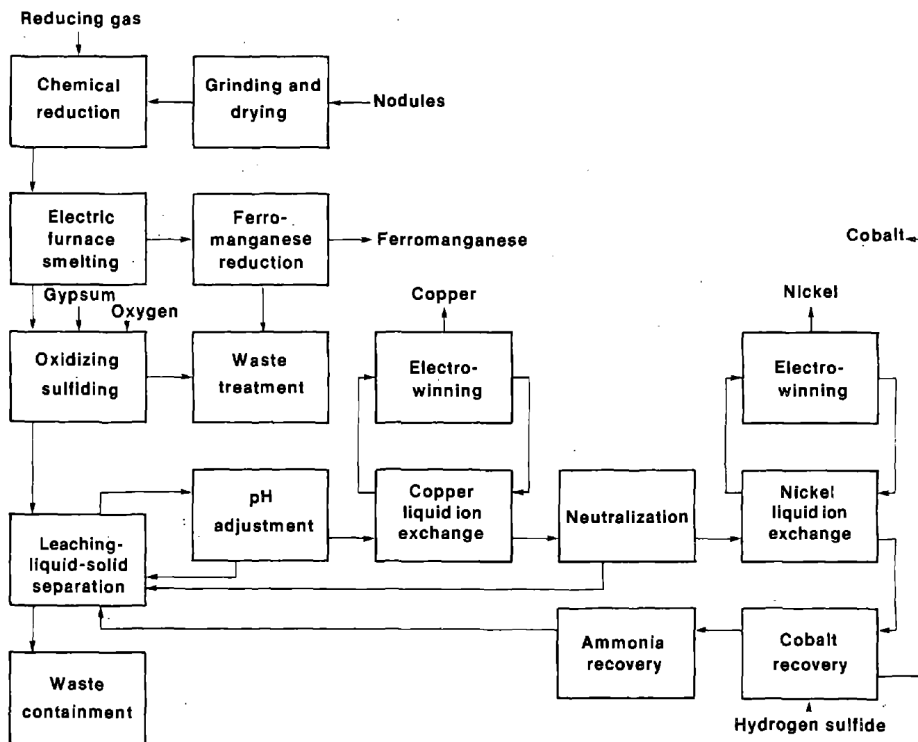
Figure 5.—Smelting and H_2SO_4 leach process.
