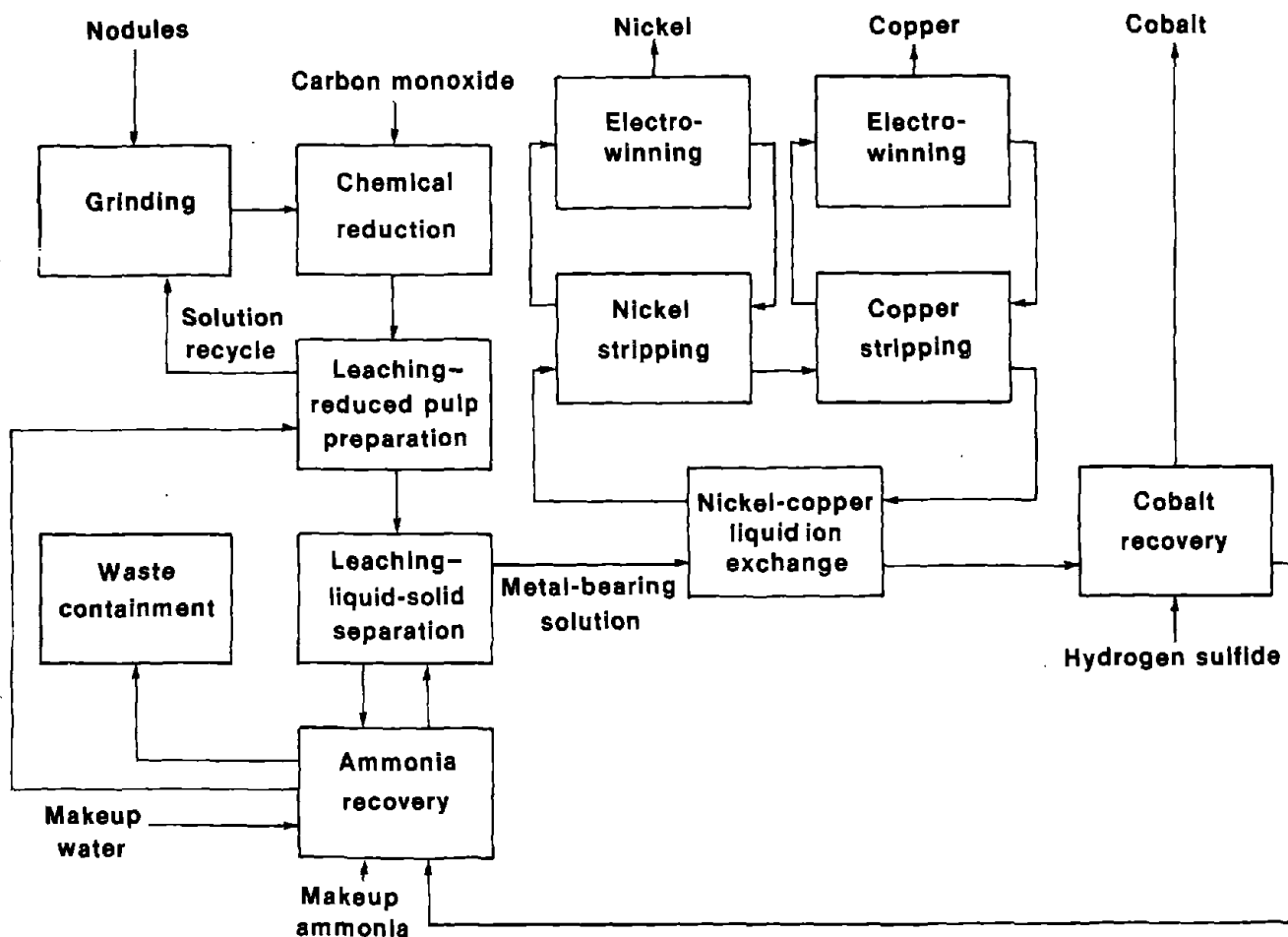
Figure 2.—Cuprion ammoniacal leach process.
