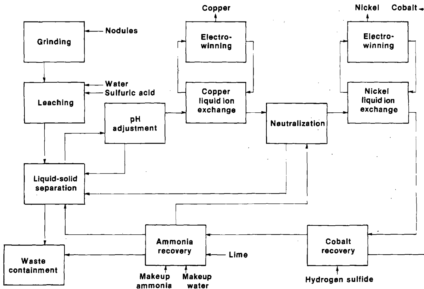
Figure 3.—High-temperature and high-pressure \text{H}_2\text{SO}_4 leach process.
