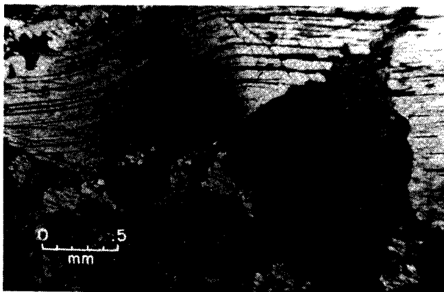
FIGURE 7. - Photomicrograph of deformed clinopyroxene grain in clinopyroxenite from upper Kanuti River ultramafic body. Groundmass consists of granulated clinopyroxene and minor olivine.
