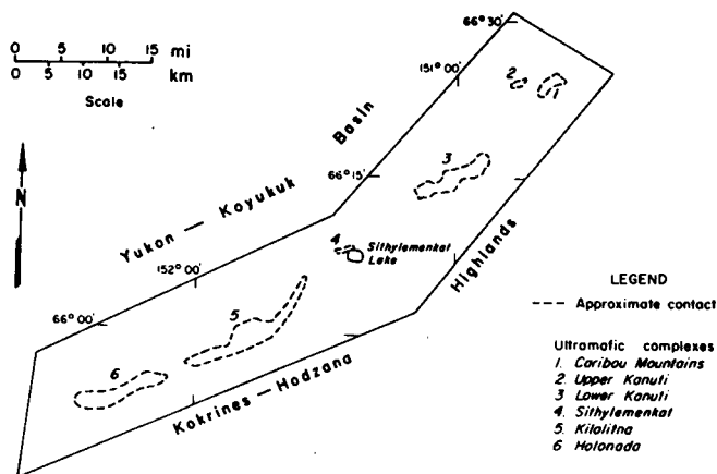
FIGURE 3. - Map showing location of the six ultramafic complexes within the Caribou Mountain-Melozitna ultramafic belt. Adapted from figure 2 in Patton and Miller, 1970 (6).
