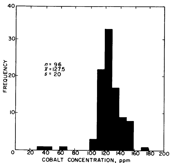
FIGURE 13. - Histogram for cobalt in 96 rock samples.
