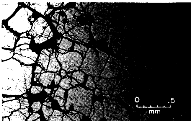
FIGURE 24. - Photomicrograph of polished section (sample G) showing coalescent habit among chromite anhedral.
