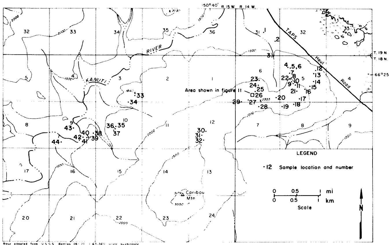
FIGURE 10. - Rock sample location map for Caribou Mountain and upper Kanuti River areas. Sample numbers are referenced in the appendixes.
