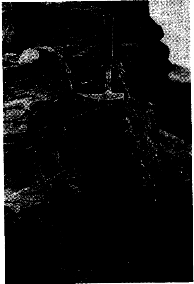
FIGURE 20. - Photograph of outcrop at chromite occurrence 12 showing alternating layers of chromite and dunite.
