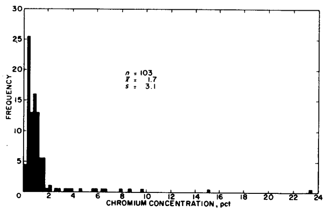
FIGURE 16. - Histogram for chromium in 103 rock samples.
