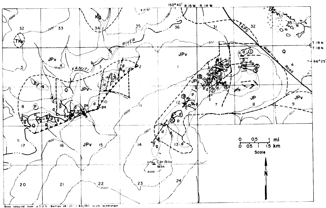
FIGURE 17. - Chromite occurrences and geologic map of Caribou Mountain and upper Kanuti River complexes.
