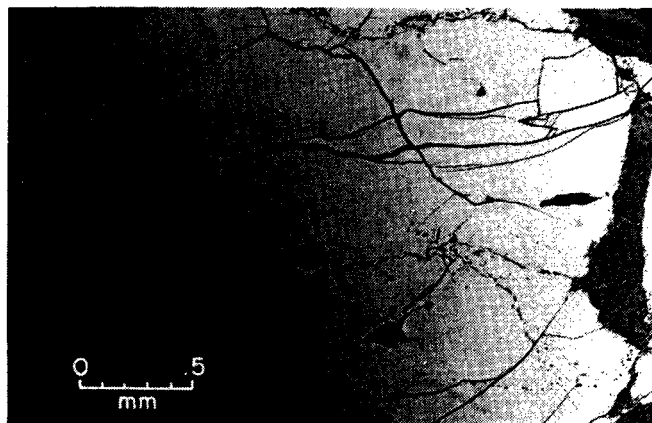
FIGURE 19. - Photomicrograph of polished section from Caribou Mountain showing fractures in massive chromite. These fractures are filled by serpentine and fine blebs of magnetite.
