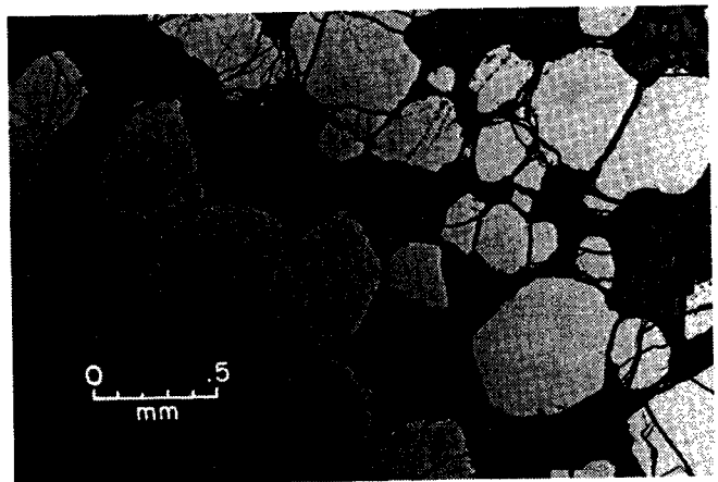
FIGURE 21. - Photomicrograph of disseminated, anhedral chromite grains in serpentinized dunite from chromite occurrence 12.
