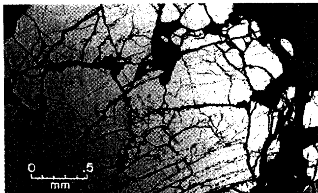
FIGURE 23. - Photomicrograph of polished section (sample F) showing fractures in massive chromite.
