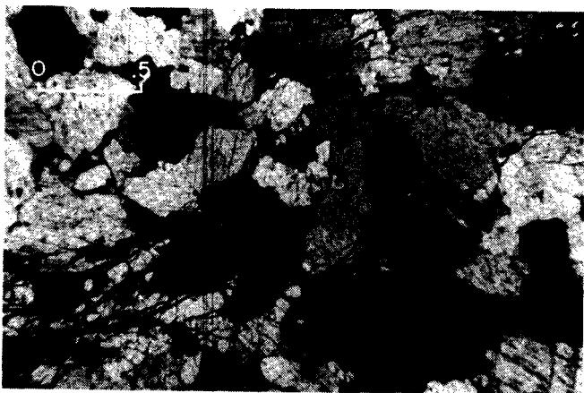
FIGURE 8. - Photomicrograph of medium-grained granular clinopyroxenite from Caribou Mountain ultramafic body.
