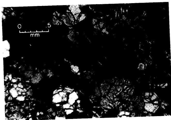
FIGURE 5. - Photomicrograph of dunite from Caribou Mountain showing mesh texture in partially serpentinized fine-grained, anhedral olivine.
