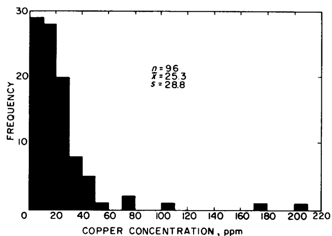
FIGURE 14. - Histogram for copper in 96 rock samples.
