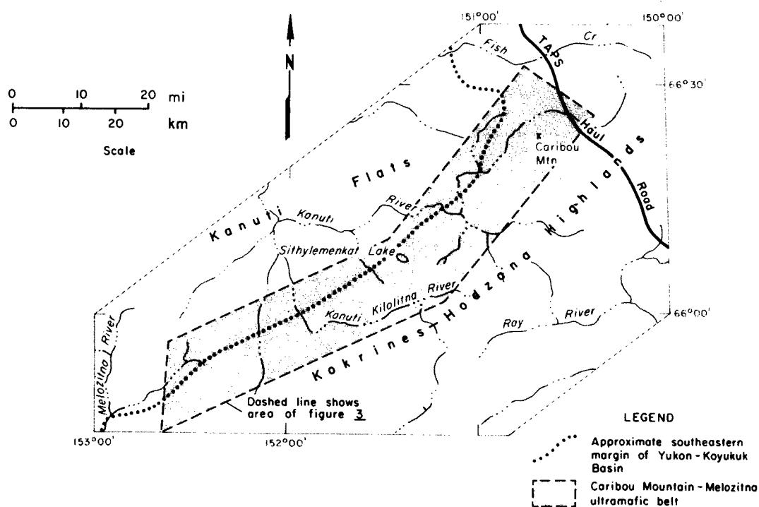
FIGURE 2. - Map showing location of Caribou Mountain-Melozitna ultramafic belt in relation to major physiographic units mentioned in the text. Adapted from figure 1 in Patton and Miller, 1970 (6).
