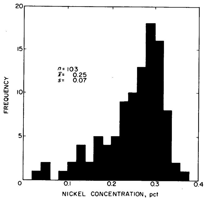
FIGURE 15. - Histogram for nickel in 103 rock samples.
