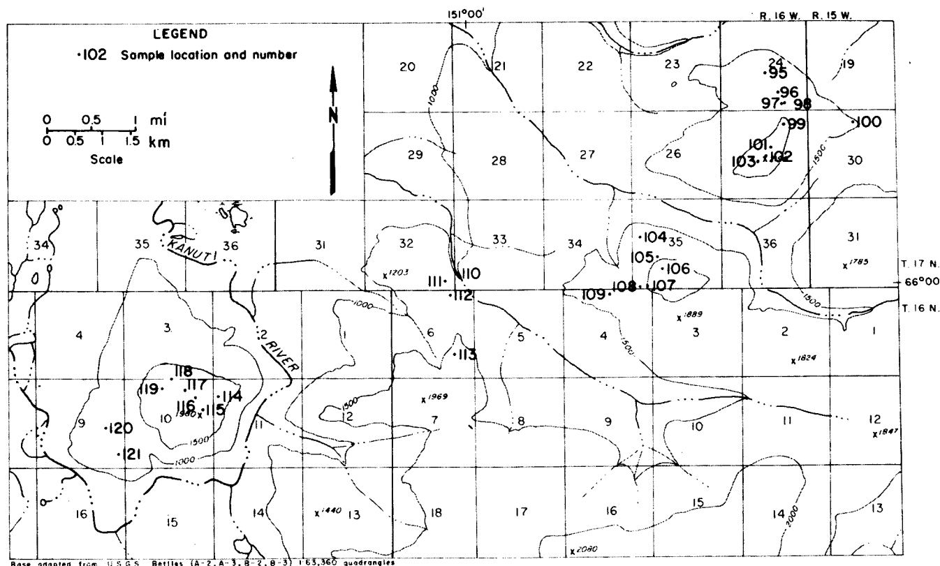
FIGURE 12. - Rock sample location map for lower Kanuti River area. Sample numbers are referenced in the appendixes.
