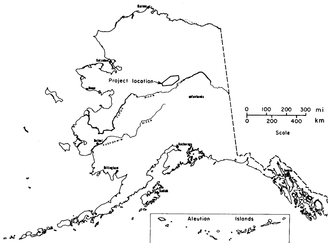
FIGURE 1. - Map of Alaska showing location of area investigated.
