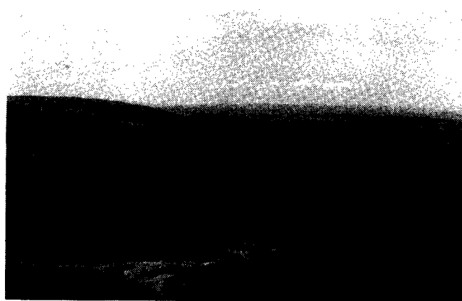
FIGURE 4. - View looking west across portion of lower Kanuti River ultramafic body. The massif in center of photograph is underlain by northwesterly dipping layers of peridotite and dunite.
