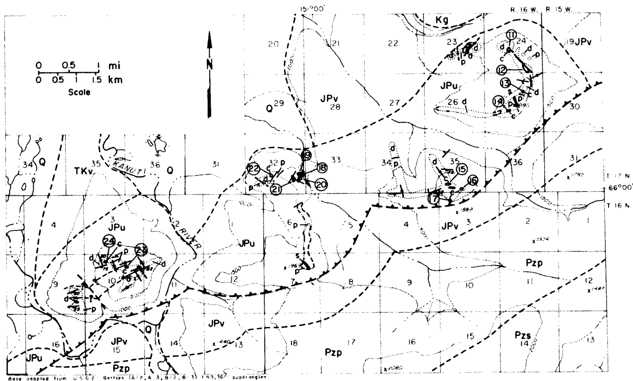
FIGURE 18. - Chromite occurrences and geologic map of lower Kanuti River complex.
