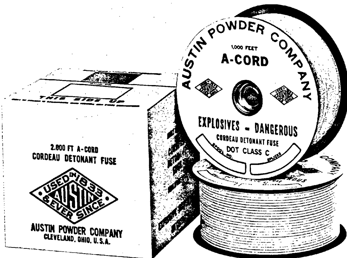
Figure 28.—Detonating cord. (Courtesy Austin Powder Co.)
