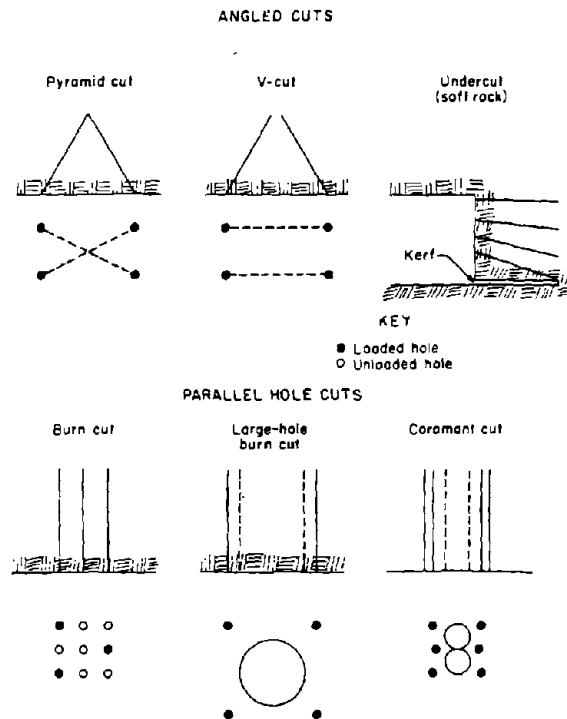
Figure 76.—Types of opening cuts.
