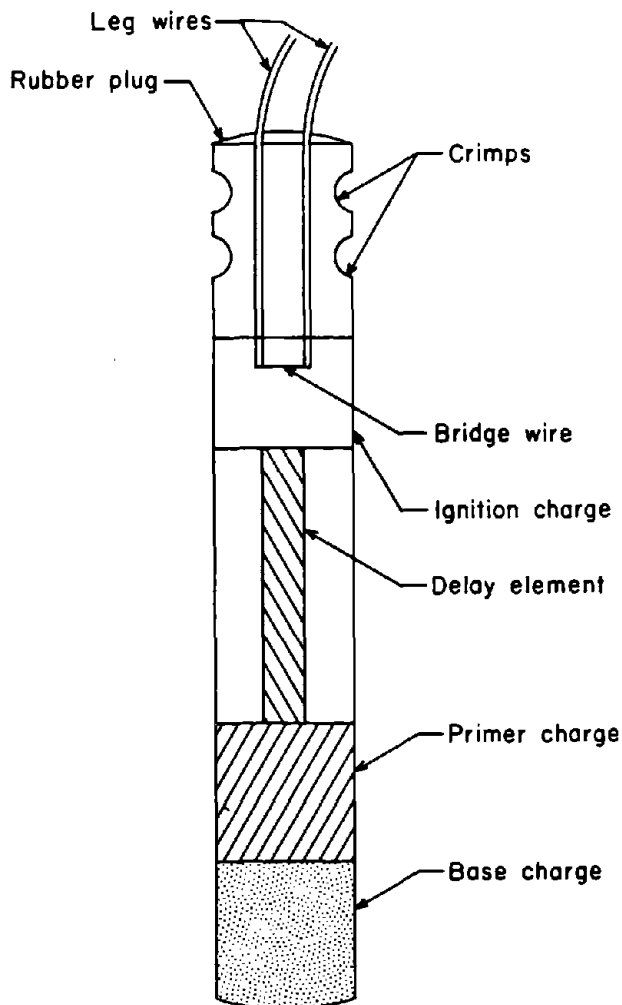
Figure 20.—Delay electric blasting cap.
