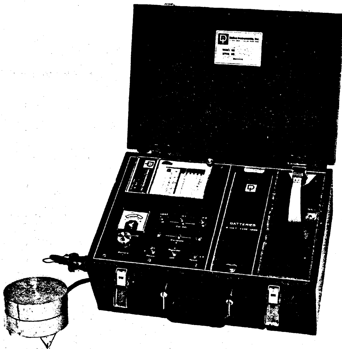
Figure 94.—Seismograph for measuring ground vibrations from blasting.
