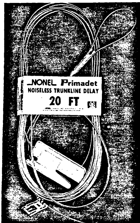
Figure 45.—Nonel noiseless trunkline delay unit. (Courtesy Ensign Bickford Co.)
