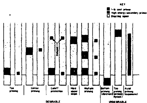
Figure 51.—Priming blasting agents in large-diameter blastholes.
