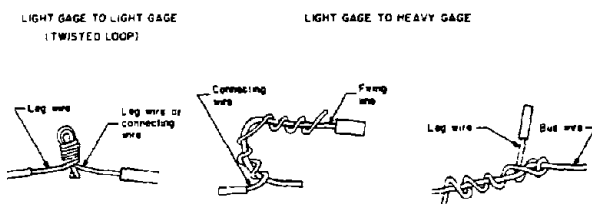
Figure 22.—Recommended wire splices.
