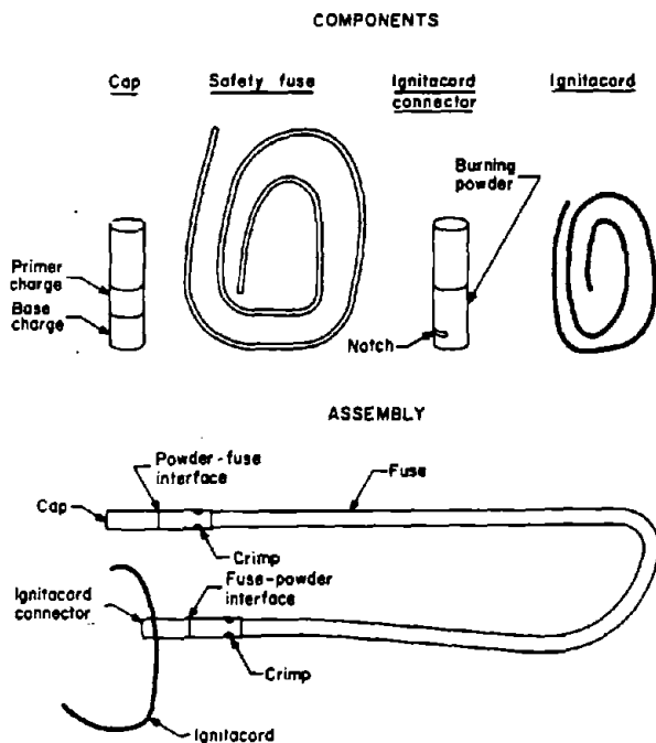
Figure 36.—Cap, fuse, and Ignitacord assembly.
