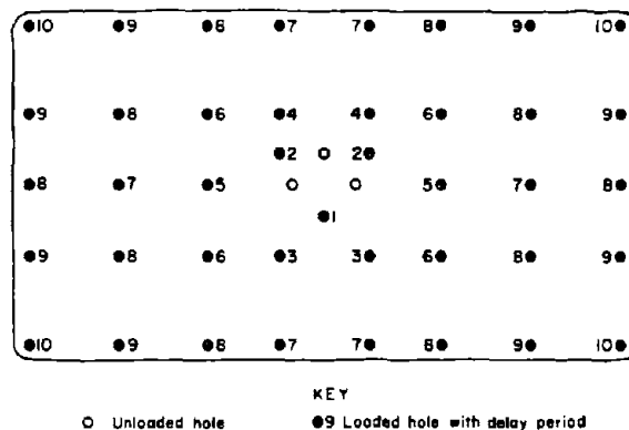
Figure 85.—Typical burn cut blast round delay pattern.
