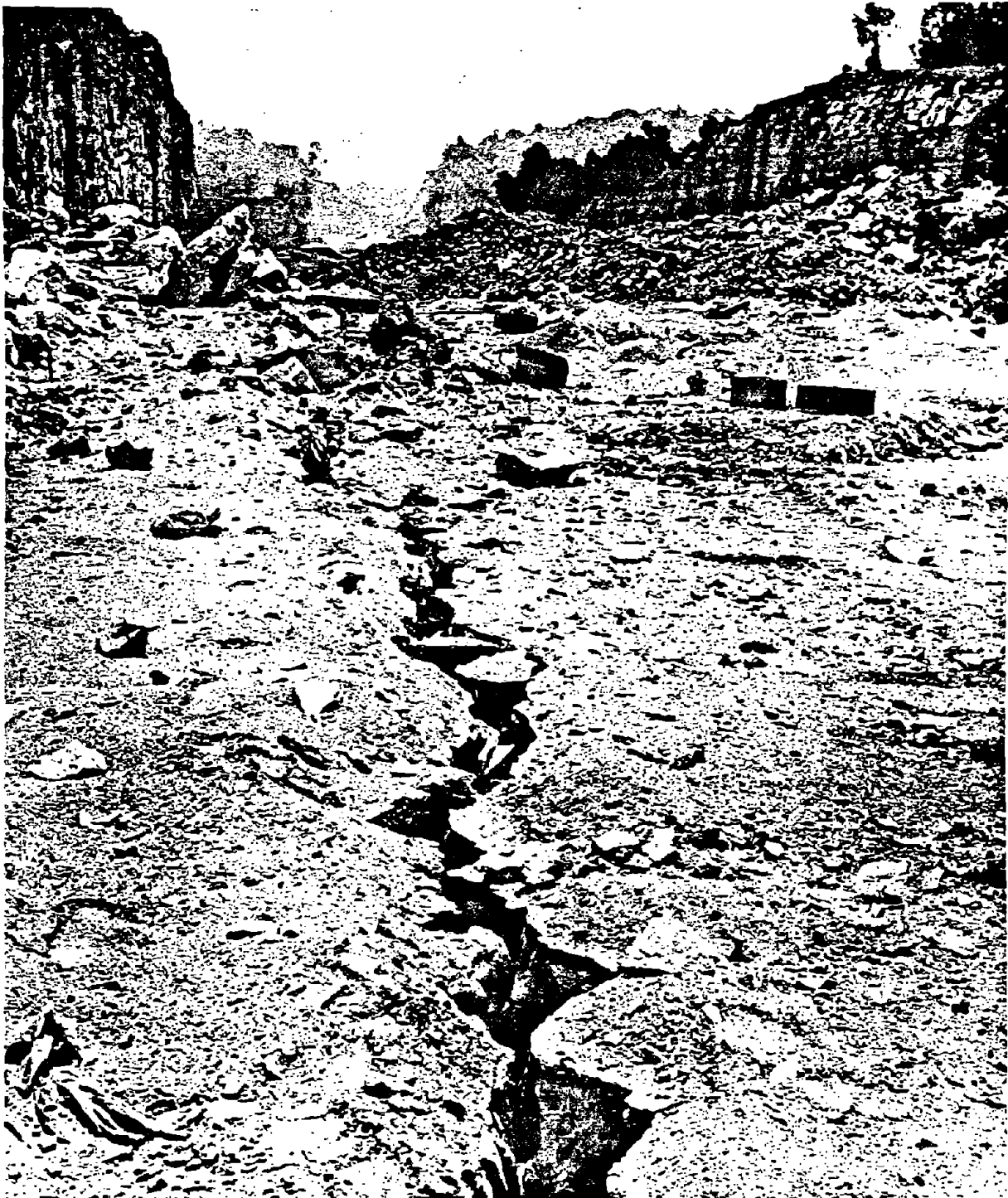
Figure 89.—Crack generated by a presplit blast. (Courtesy Austin Powder Co.)
