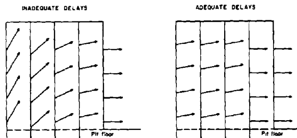
Figure 75.—The effect of inadequate delays between rows.
