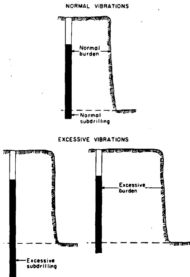
Figure 95.—Effects of confinement on vibration levels.
