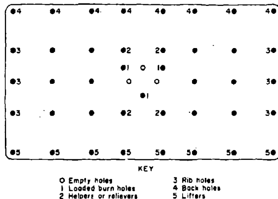
Figure 80.—Nomenclature for blastholes in a heading round.
