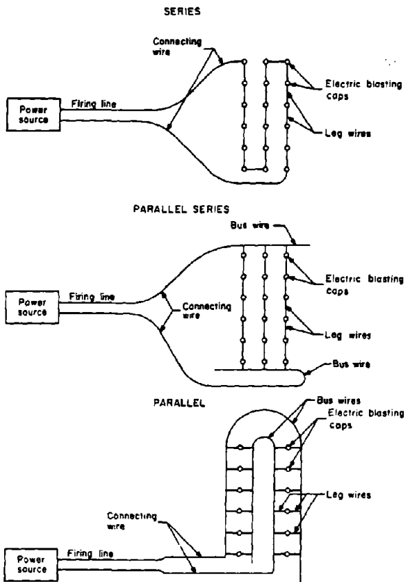
Figure 21.—Types of electric blasting circuits.
