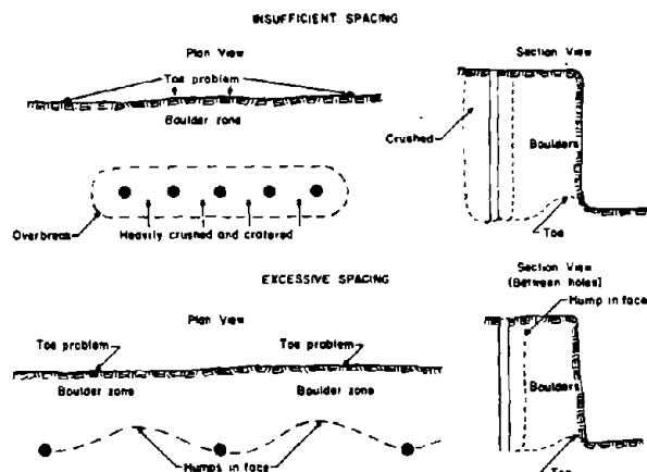
Figure 72.—Effects of Insufficient and excessive spacing.
