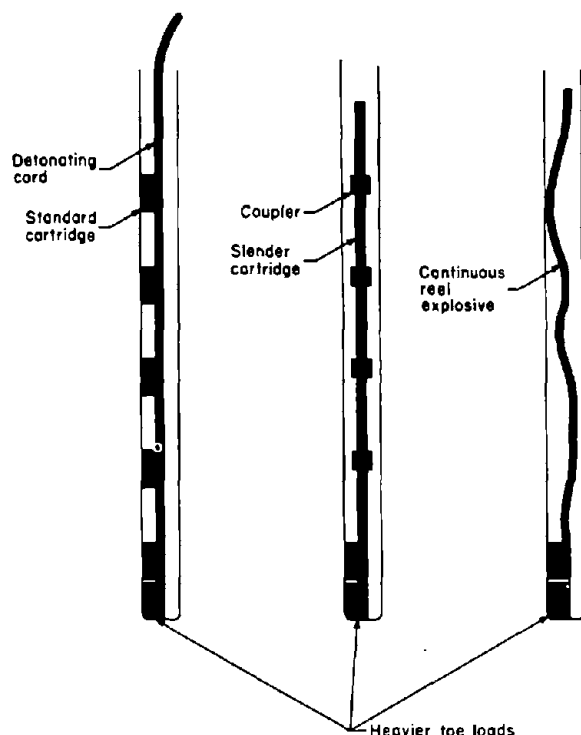
Figure 90.—Three typical blasthole loads for presplitting.
