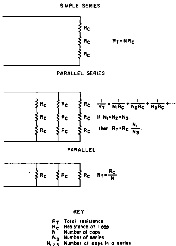
Figure 23.—Calculation of cap circuit resistance.
