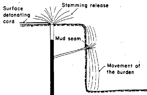
Figure 98.—Causes of airblast.
