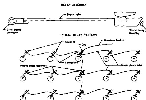
Figure 46.—Noiseless trunkline using Nonel delay assemblies.
