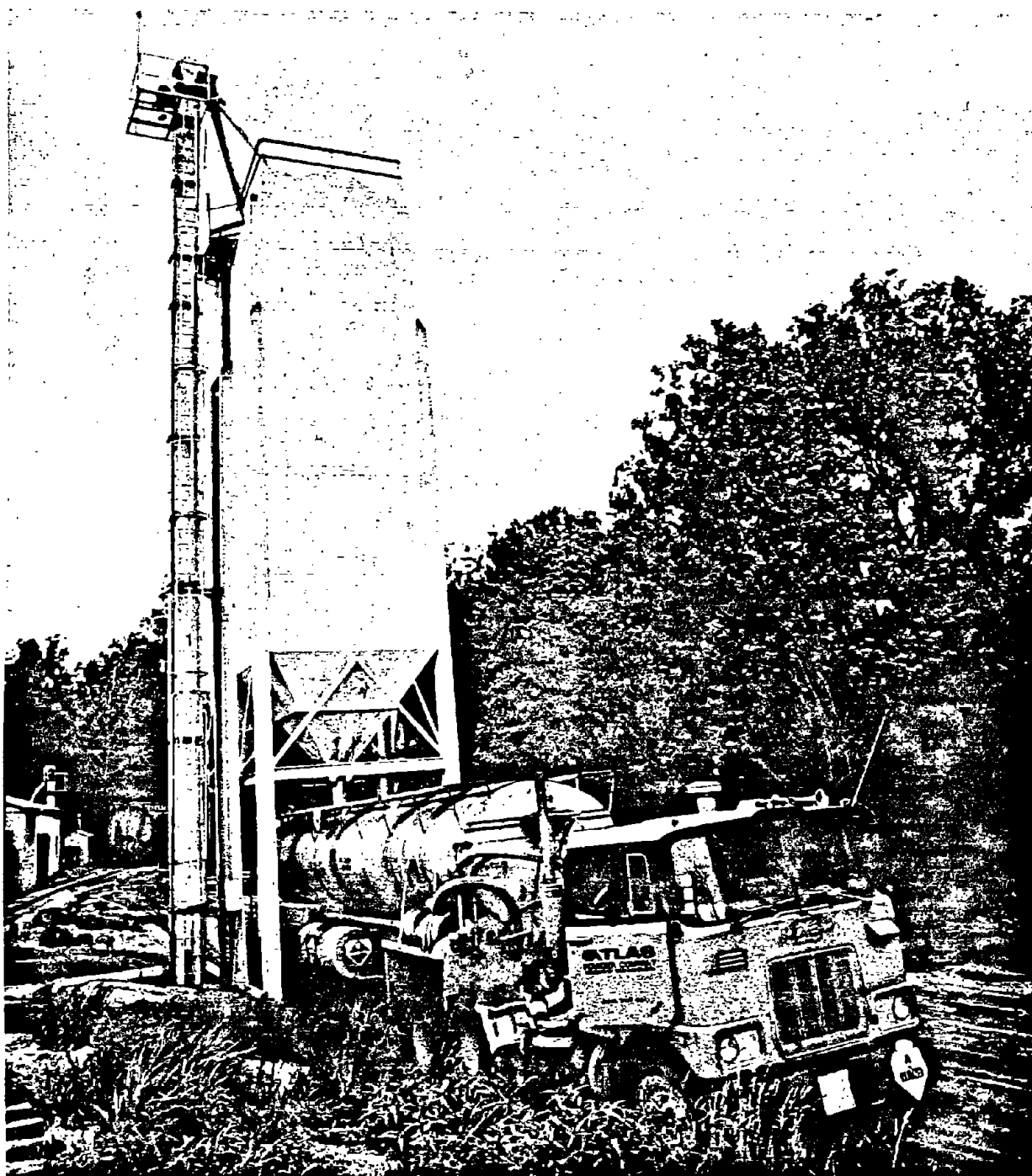
Figure 100.—AN-FO bulk storage facility. (Courtesy Atlas Powder Co.)
