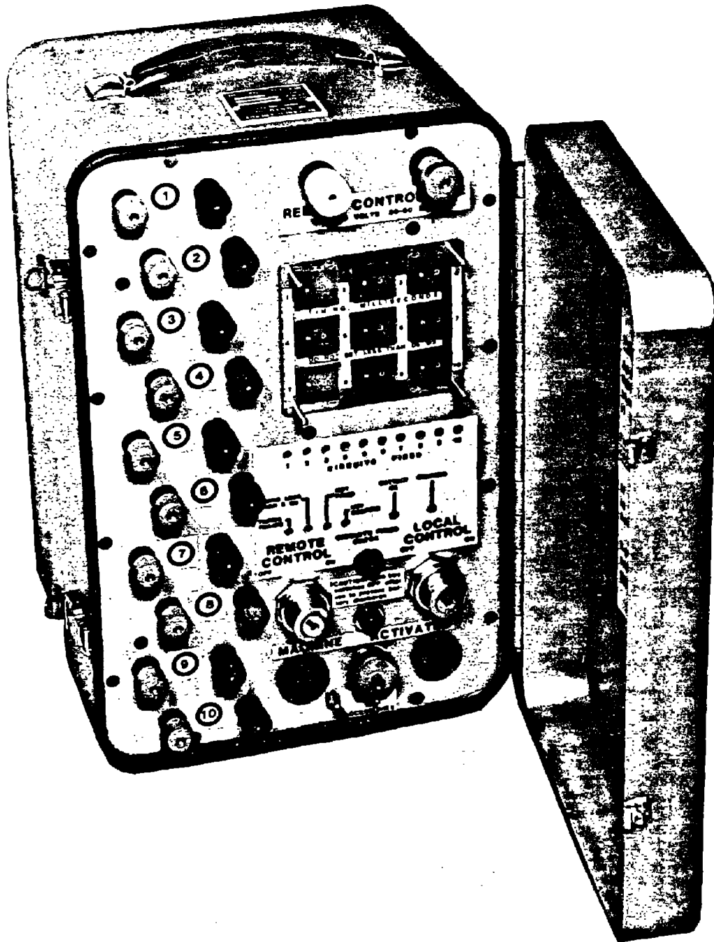
Figure 25.—Sequential blasting machine.
