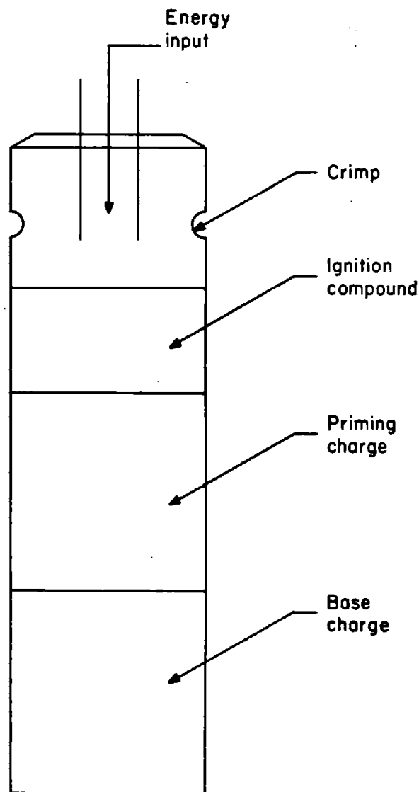
Figure 17.—Instantaneous detonator.
