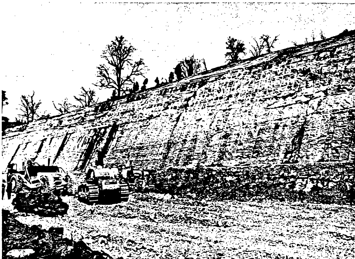
Figure 88.—Stable slope produced by controlled blasting. (Courtesy Austin Powder Co.)
