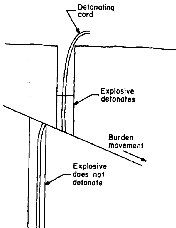
Figure 34.—Misfire caused by cutoff from burden movement.
