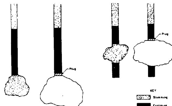
Figure 52.—Corrective measures for voids.
