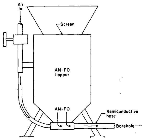
Figure 54.—Ejector-type pneumatic AN-FO loader.
