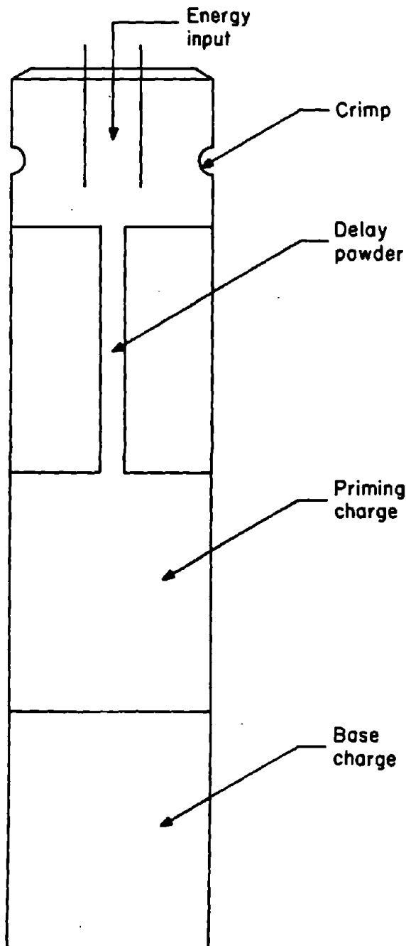
Figure 18.—Delay detonator.
