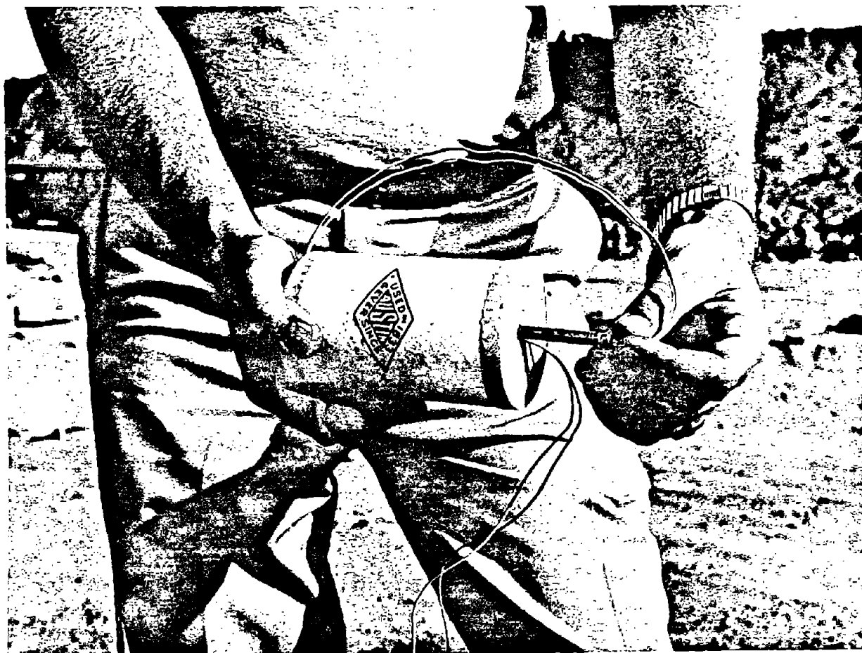
Figure 50.—Priming cast primer with electric blasting cap. (Courtesy Austin Powder Co.)
