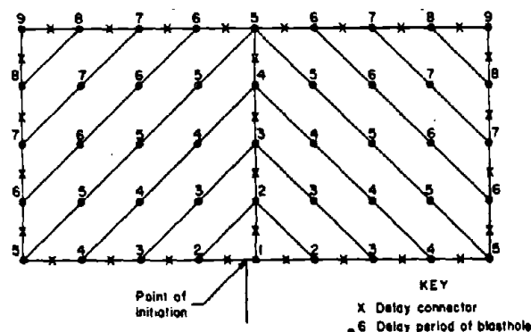
Figure 33.—Typical blast pattern with surface delay connectors.
