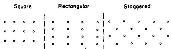
Figure 67.—Three basic types of drill pattern.
