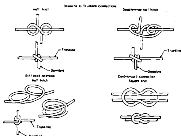
Figure 31.—Recommended knots for detonating cord.
