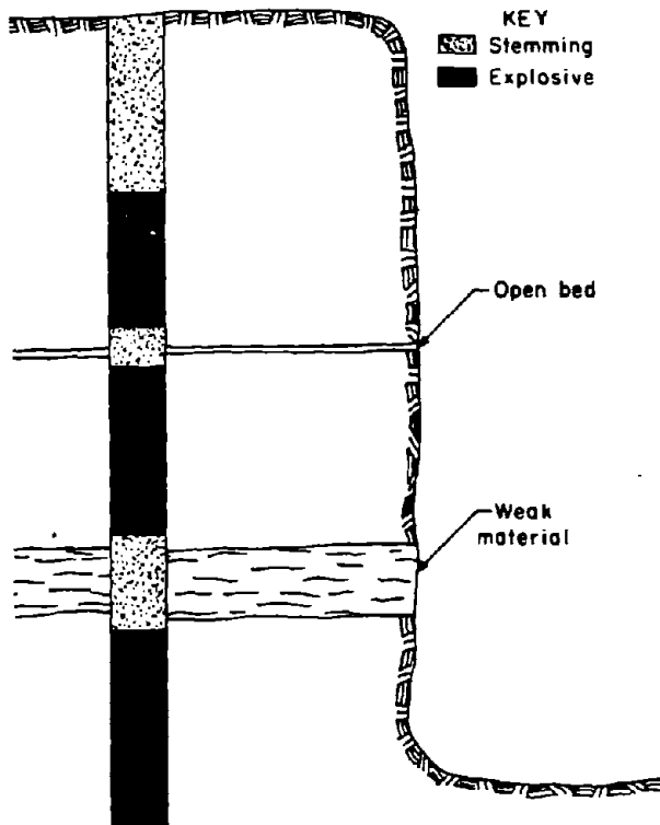
Figure 62.—Stemming through weak material and open beds.
