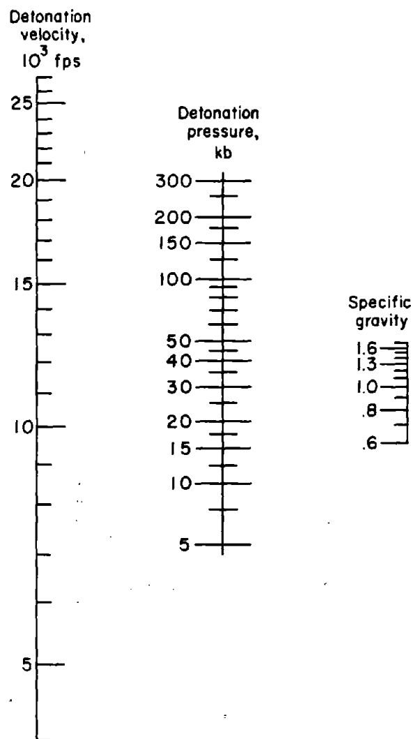
Figure 15.—Nomograph for finding detonation pressure.
