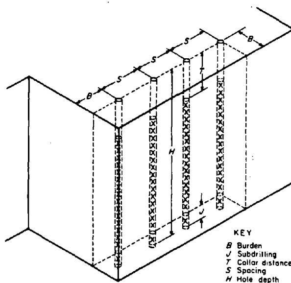
Figure 70.—Isometric view of a bench blast.
