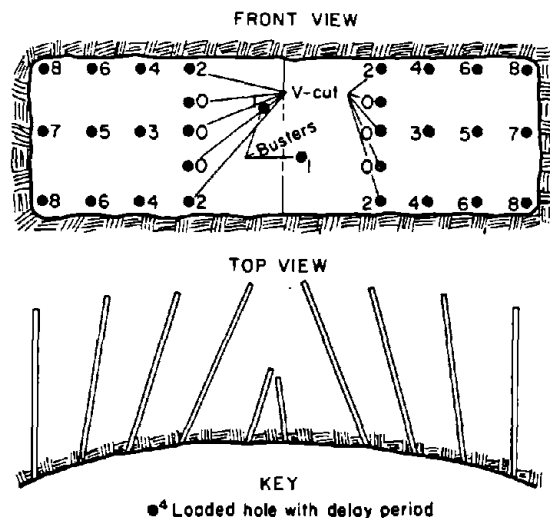
Figure 86.—Typical V-cut blast round delay pattern.
