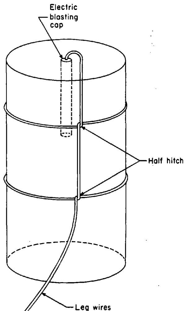
Figure 49.—Cartridge primed with electric blasting cap.
