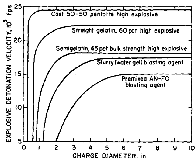
Figure 13.—Effect of charge diameter on detonation velocity.
