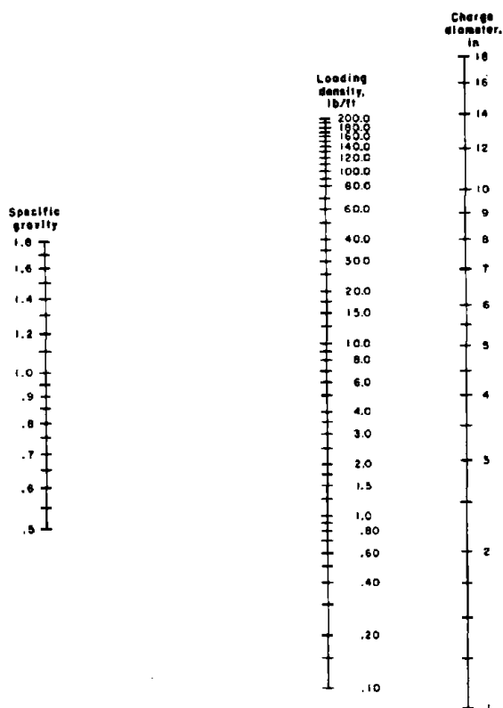
Figure 14.—Nomograph for finding loading density.
