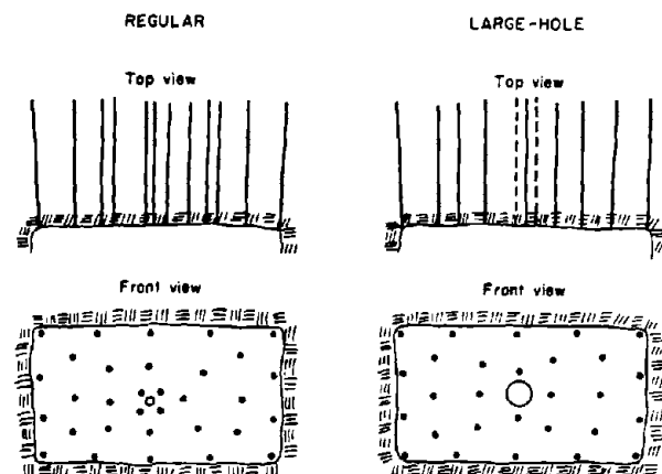
Figure 82.—Parallel hole cut blast rounds.
