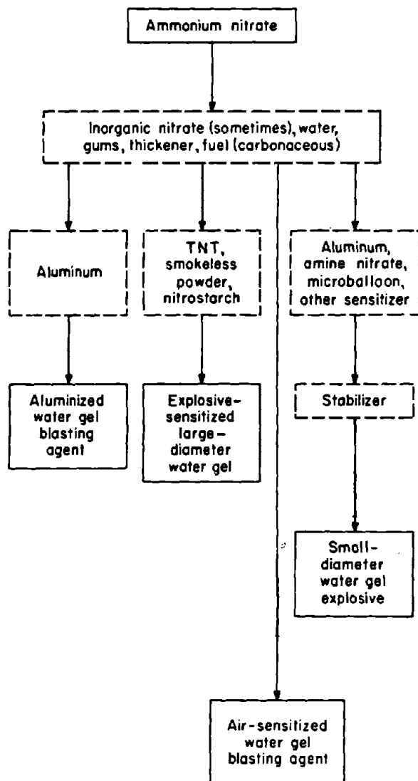
Figure 8.—Formulations of water-based products.
