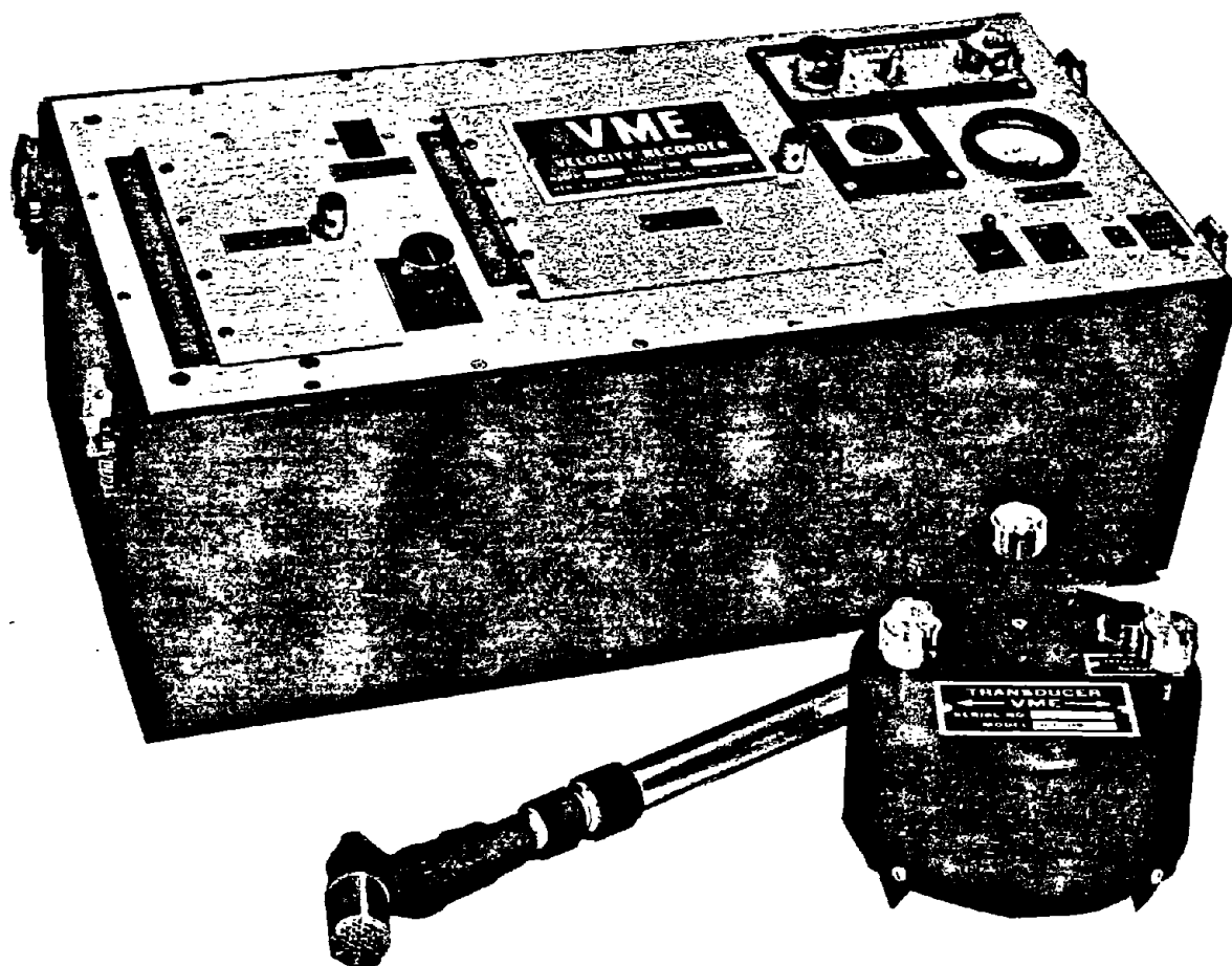
Figure 97.—Blasting seismograph with microphone for measuring airblast.
