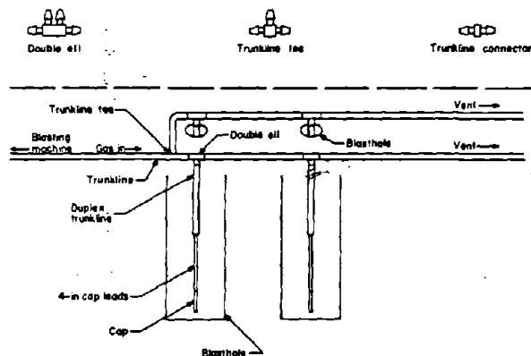
Figure 39.—Hercudet connections for surface blasting.
