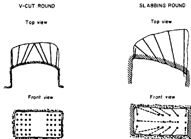
Figure 81.—Angled cut blast rounds.
