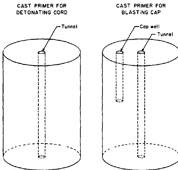
Figure 11.—Cast primers for blasting caps and detonating cord.
