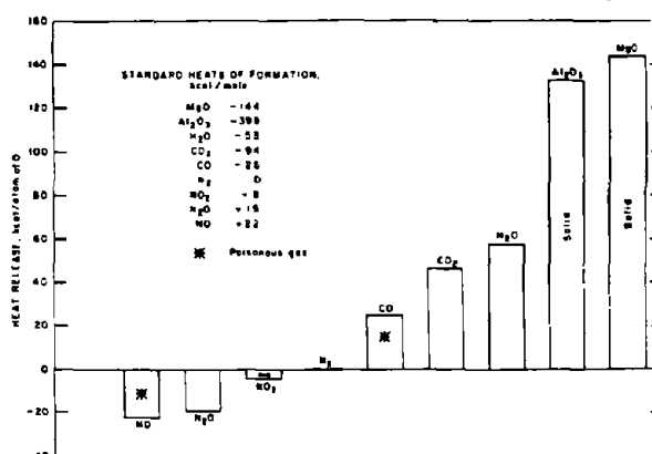
Figure 1.—Energy released by common products of detonation.
