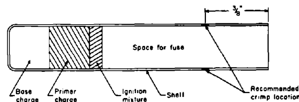
Figure 35.—Blasting cap for use with safety fuse.
