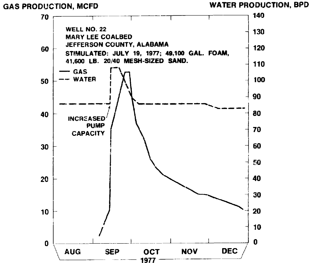
FIGURE 4. - PRODUCTION CURVES FROM A DRAINAGE WELL PLACED MORE THAN 3000 FEET FROM ANOTHER DRAINAGE POINT IN THE MARY LEE COALBED.
