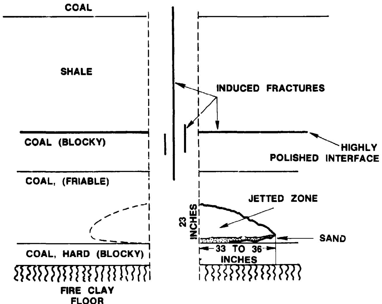
FIGURE 63. - SKETCH OF TW5 WELLBORE SHOWING POSITION AND ORIENTATION OF INDUCED FRACTURES AS INDICATED BY THE PRESENCE OF FLUORESCENT MATERIAL CONTAINED IN THE STIMULATION TREATMENT FLUID.
