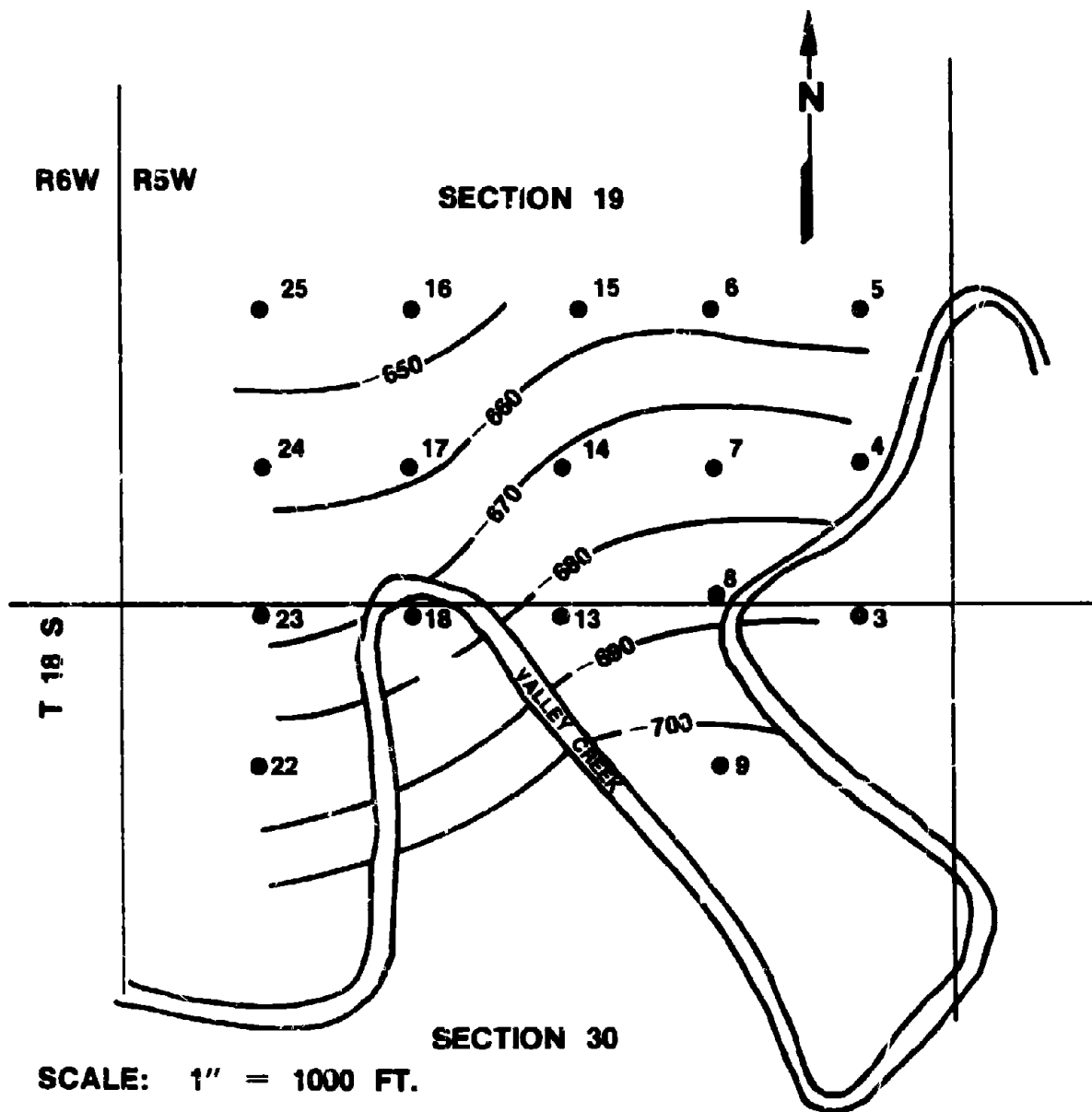
FIGURE 47. - OAK GROVE DEGASIFICATION GRID PATTERN, MARY LEE COALBED, JEFFERSON CO., ALABAMA
