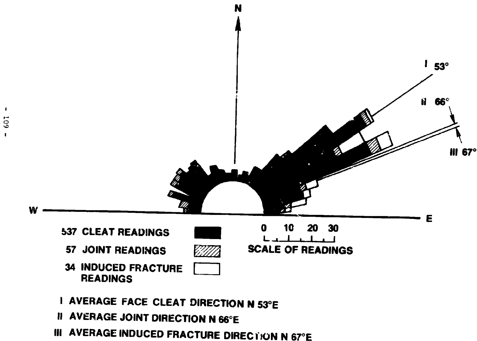
FIGURE 45. - COMPOSITE ROSE DIAGRAM OF TW3 AND TW4 SURVEY AREA SHOWING CLEAT, ROOF JOINT, AND INDUCED FRACTURE DIRECTIONS.
