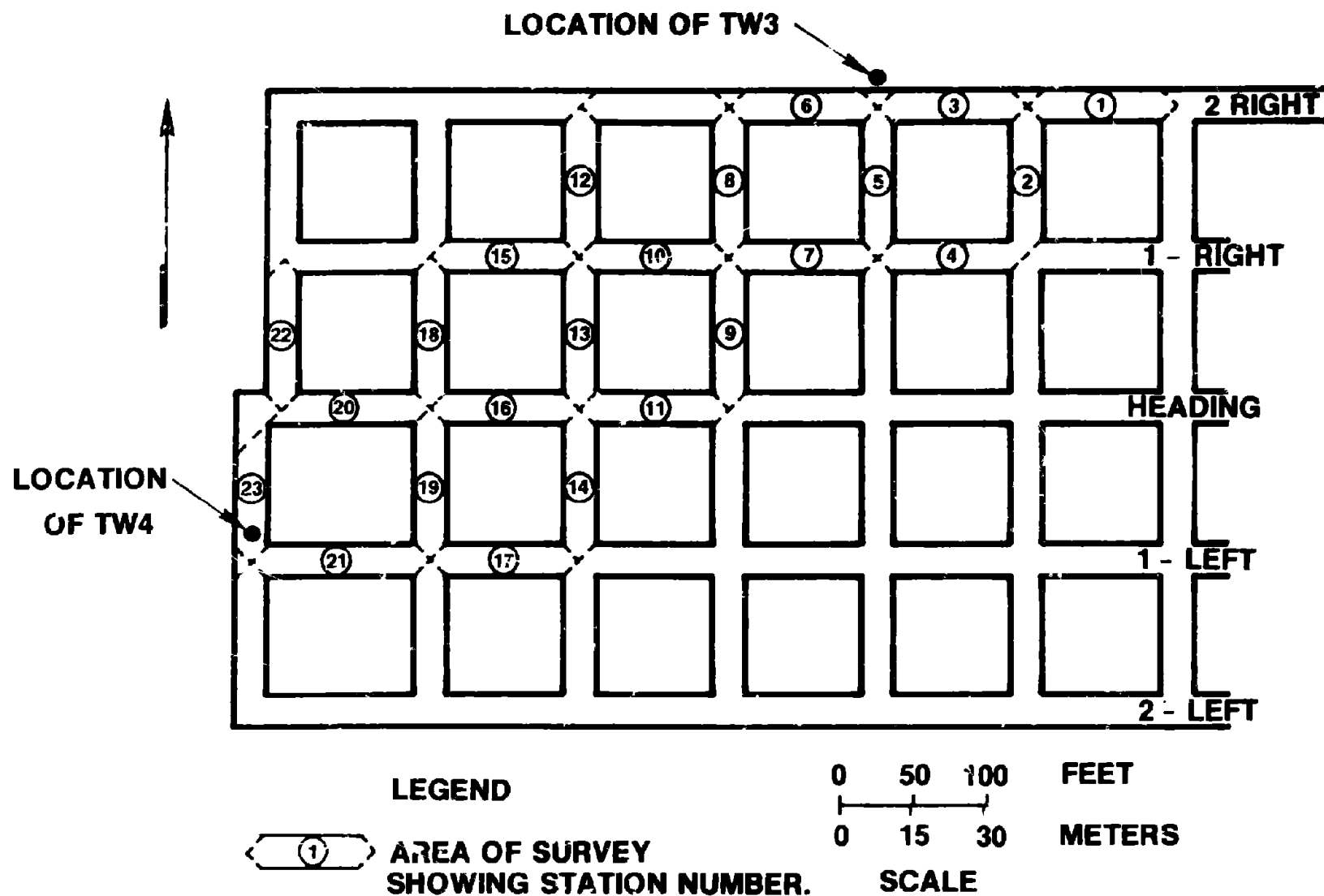
FIGURE 44. - SURVEY STATIONS DIVIDING AREA OF MINE NEAR TW3 AND TW4 (26).
