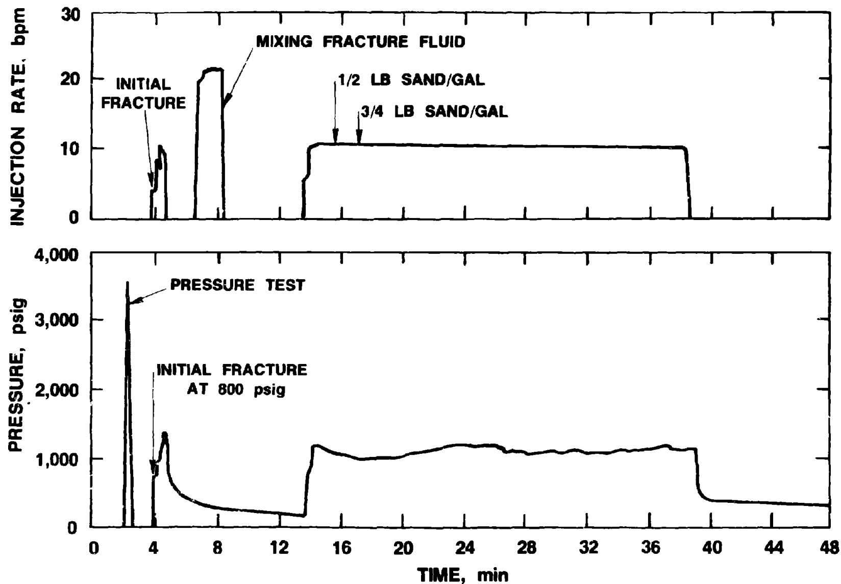
FIGURE 20. - WELLHEAD PRESSURE AND INJECTION RATE CHARTS OF HYDRAULIC STIMULATION OF THE MARY LEE COALBED (7).
