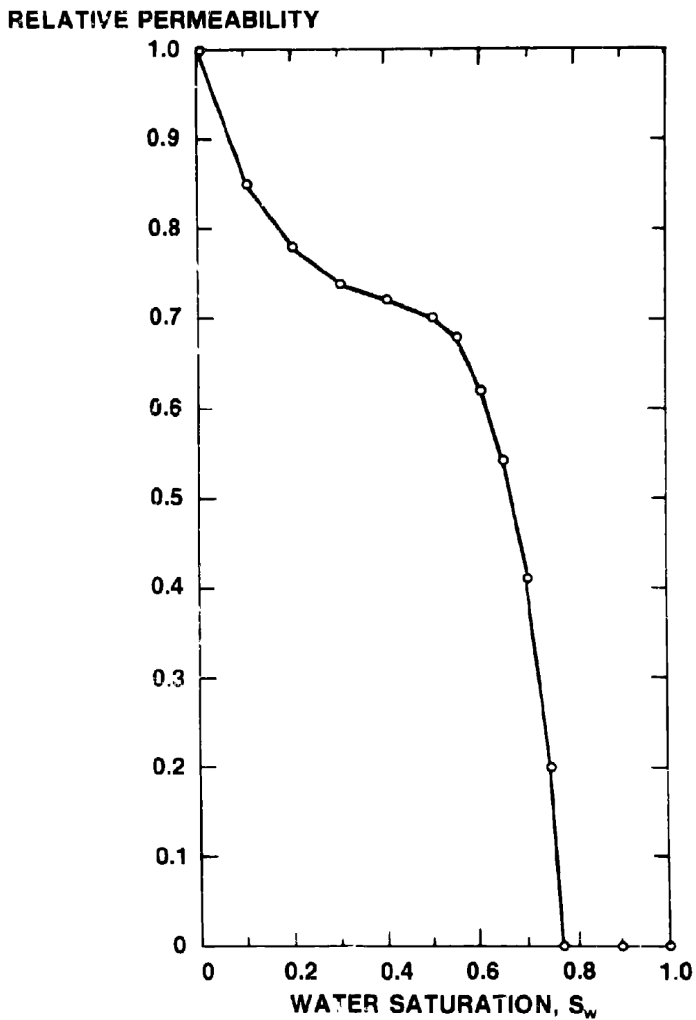
FIGURE 3. - GAS PERMEABILITY RELATIVE TO WATER SATURATION (22).
