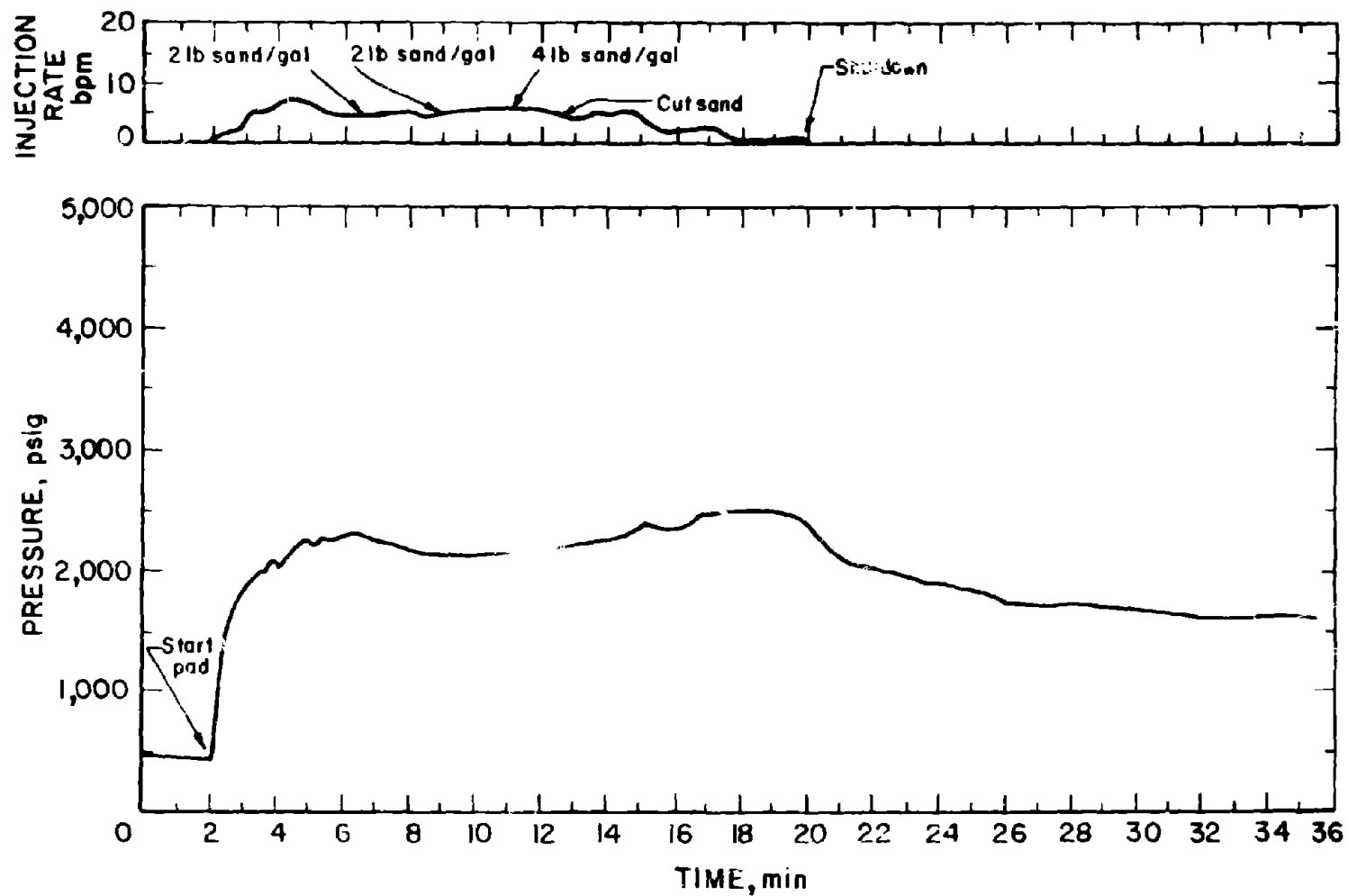
FIGURE 24. - HYDRAULIC STIMULATION PRESSURE AND FLUID INJECTION CHART TW2, MARY LEE COALBED (23).
