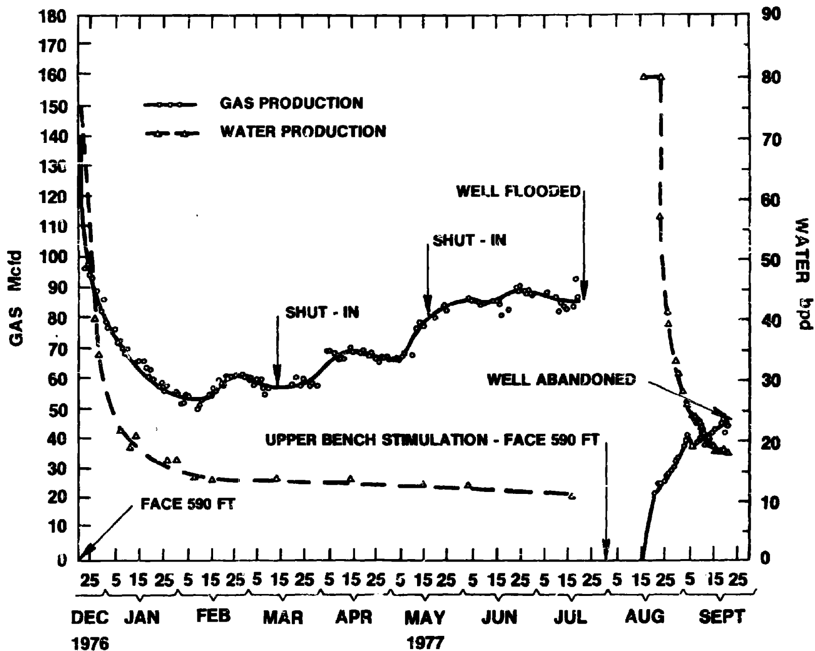
FIGURE 42. - PRODUCTION CURVES FOR TW3 (26).
