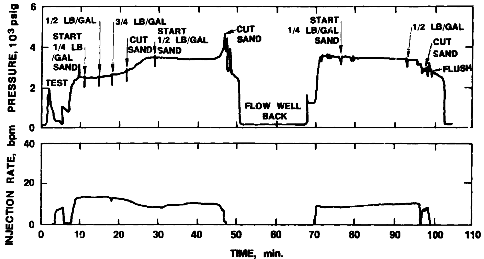
FIGURE 18. - WELL HEAD PRESSURE AND INJECTION RATE CHARTS OF HYDRAULIC STIMULATION TREATMENT OF POCAHONTAS NO. 3 COALBED (16).
