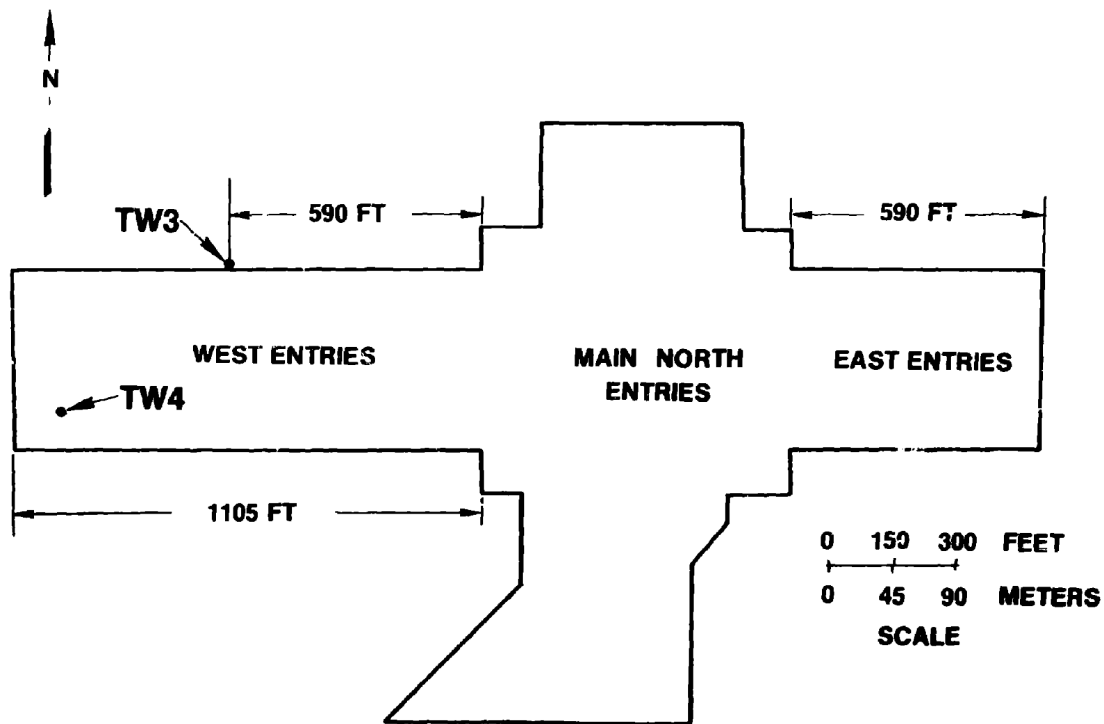
FIGURE 65. - VIEW OF MINE SHOWING TEST WELL LOCATIONS AND MINE ENTRIES STUDIED FOR GAS EMISSIONS.
