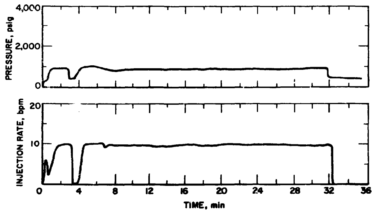
FIGURE 31. - PRESSURE AND INJECTION RATE CHARTS DURING HYDRAULIC STIMULATION, USBM NO.1 NE, JEFFERSON COUNTY, ILL. (16).
