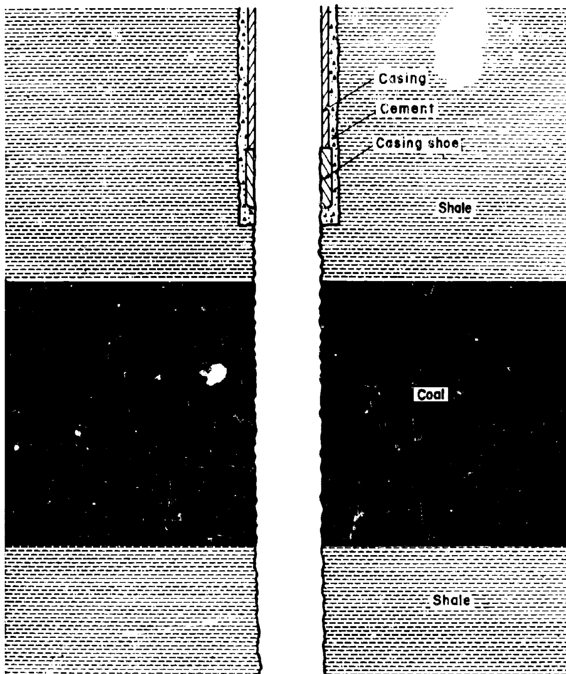
FIGURE 13. - SINGLE-HORIZON (OPENHOLE) COMPLETION
