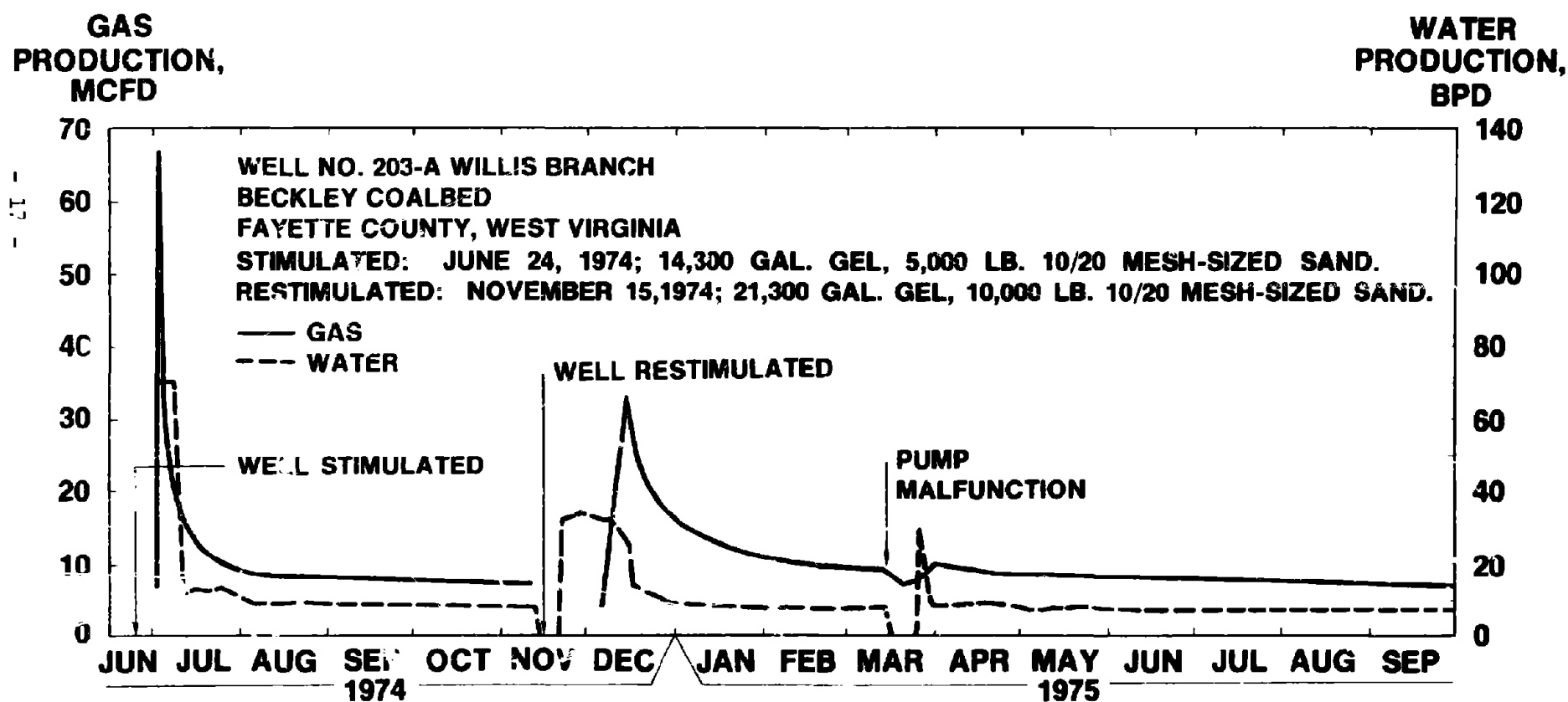
FIGURE 6. - PRODUCTION CURVES FROM A COALBED GAS DRAINAGE WELL PLACED MORE THAN 3000 FEET FROM ANOTHER DRAINAGE POINT IN THE BECKLEY COALBED.
