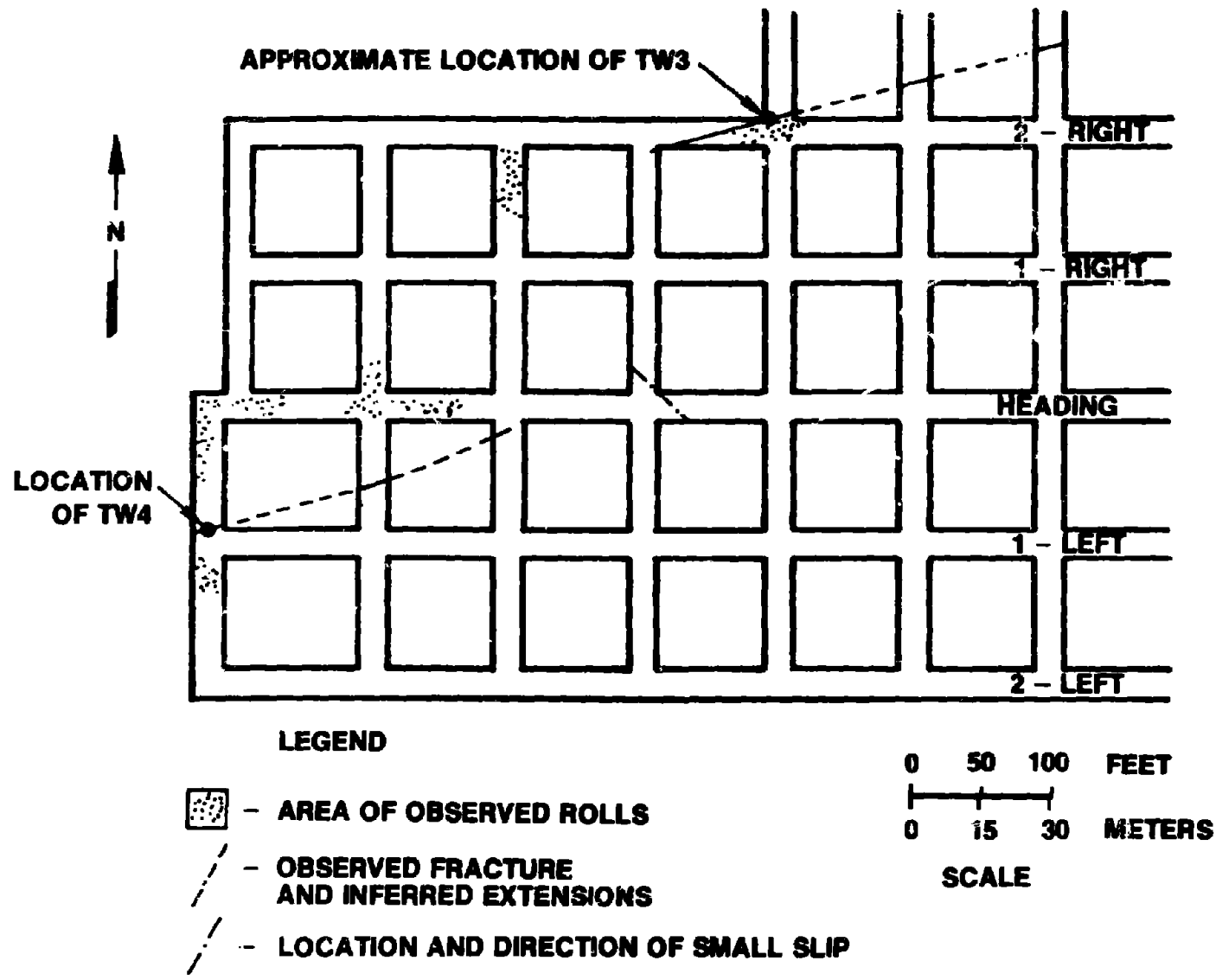
FIGURE 46. - PLAN VIEW OF MINE SHOWING TW3 AND TW4 LOCATIONS, TRACEABLE INDUCED FRACTURES AND OTHER FEATURES AS OBSERVED UNDERGROUND (26).
