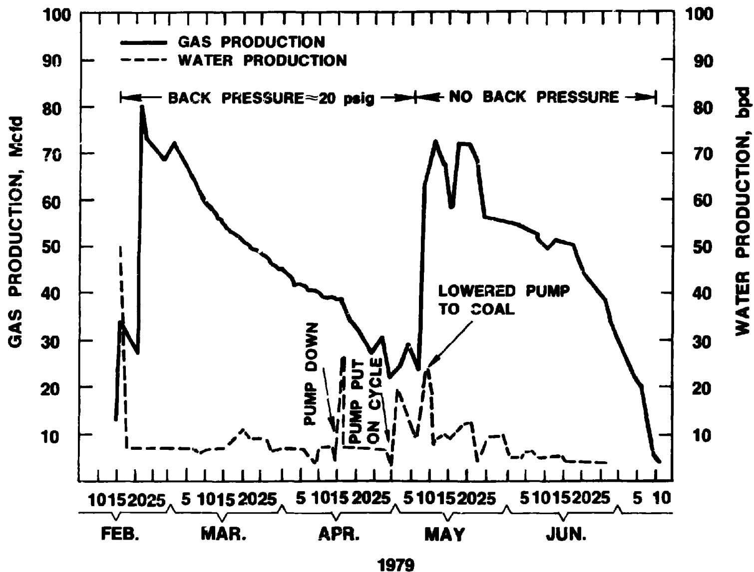
FIGURE 61. - DAILY PRODUCTION FROM TW5, MARY LEE COALBED, JEFFERSON COUNTY, ALABAMA.
