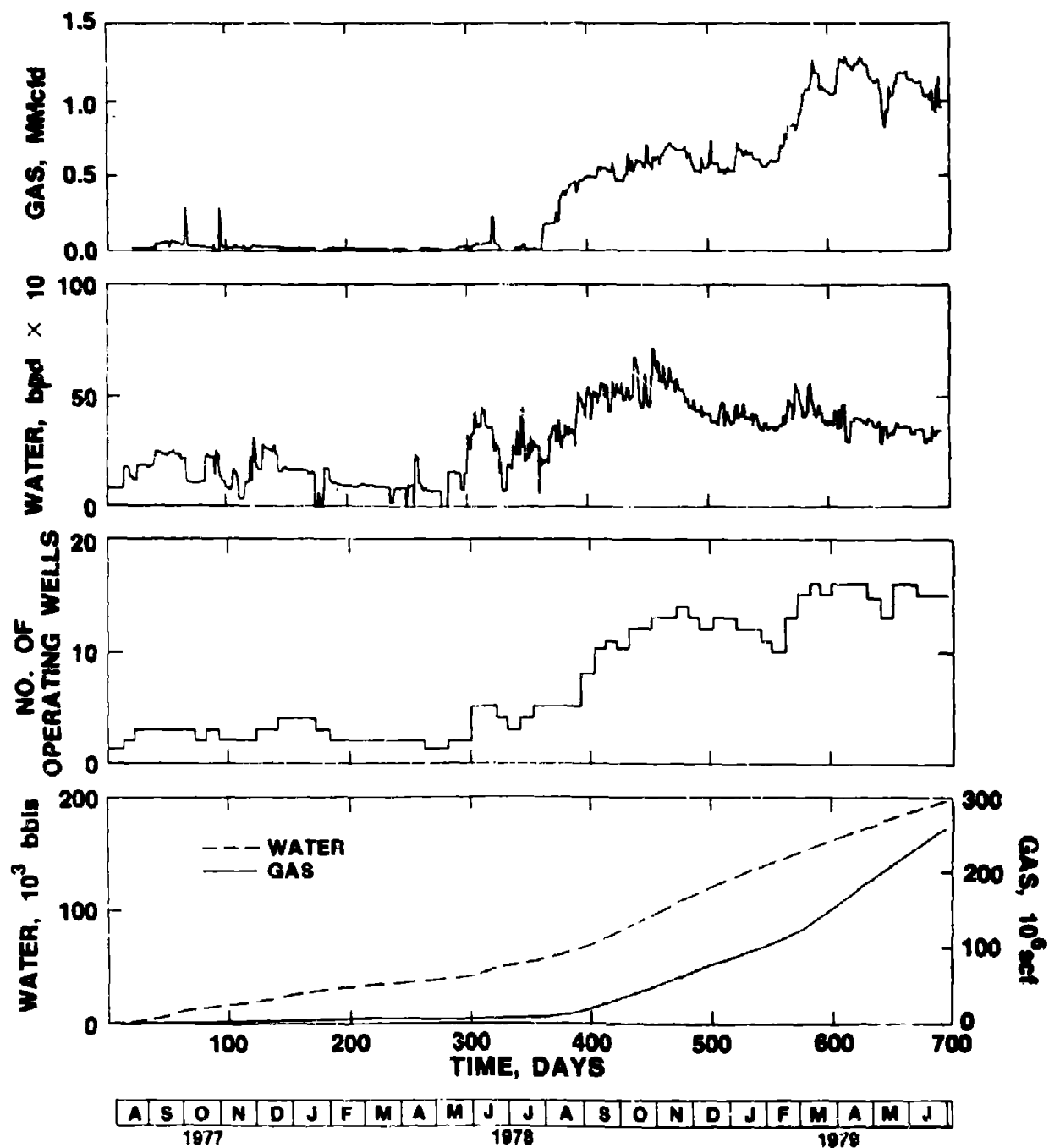
FIGURE 56 - DAILY PRODUCTION; NUMBER OF OPERATING WELLS AND CUMULATIVE TOTAL AMOUNT OF GAS AND WATER PRODUCED FROM THE MARY LEE COALBED DEGASIFICATION PATTERN NEAR OAK GROVE, JEFFERSON COUNTY, ALABAMA
