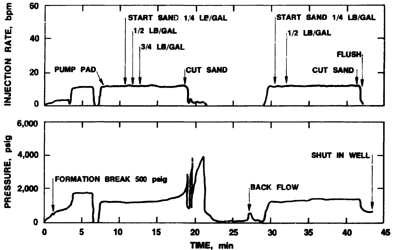
FIGURE 22. - WELL HEAD PRESSURE AND INJECTION RATE CHARTS OF HYDRAULIC STIMULATION TREATMENT OF PITTSBURGH COAL BED (14).
