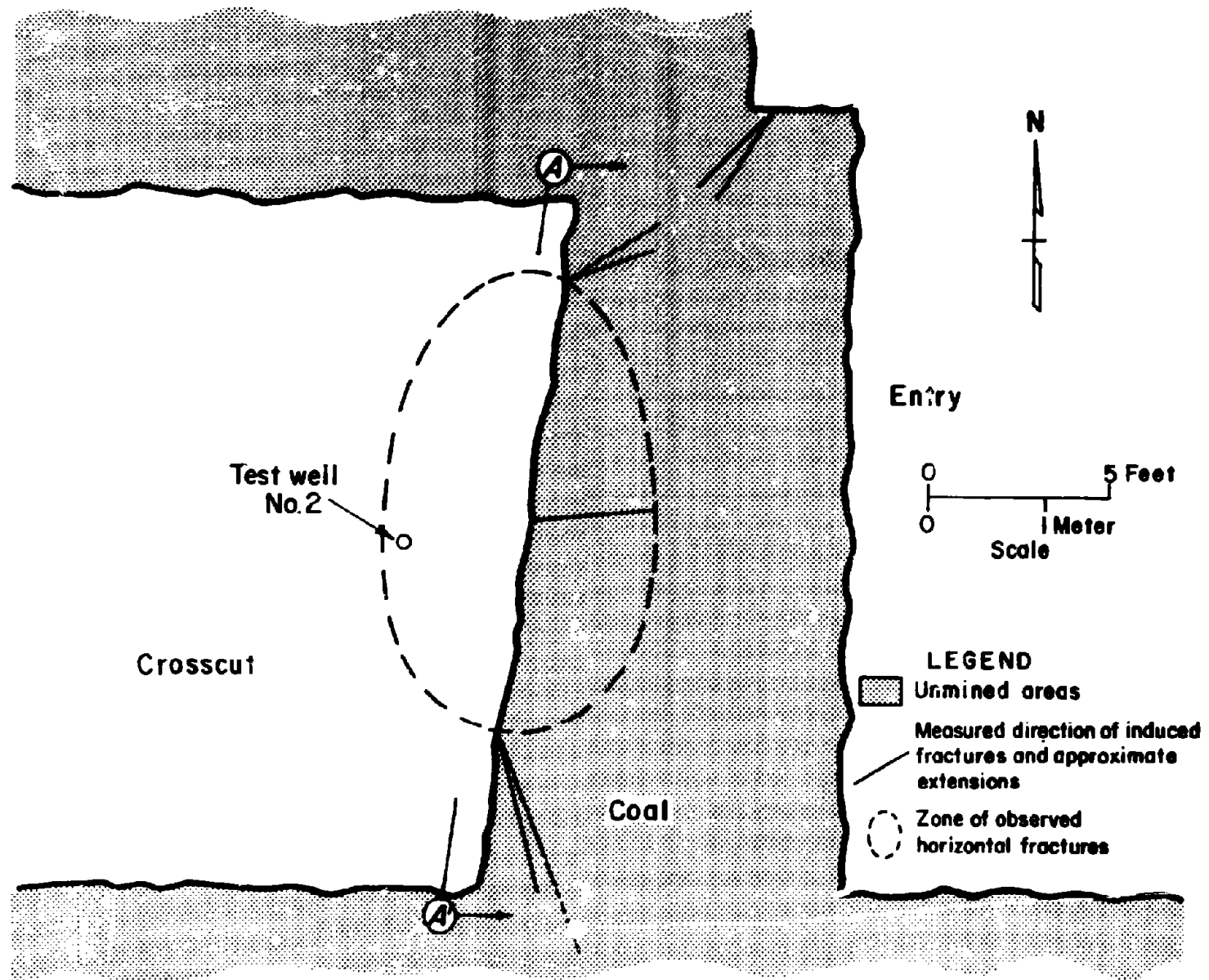
FIGURE 26. - POSITION OF MINE FACE DURING UNDERGROUND INVESTIGATION OF TW2 (23).
