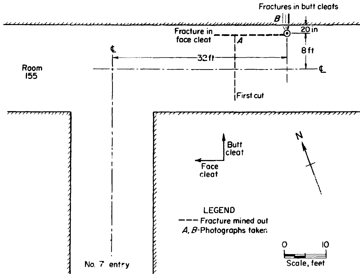
FIGURE 28. - INDUCED FRACTURE ORIENTATION RELATIVE TO MINE ENTRY DEVELOPMENT (16).
