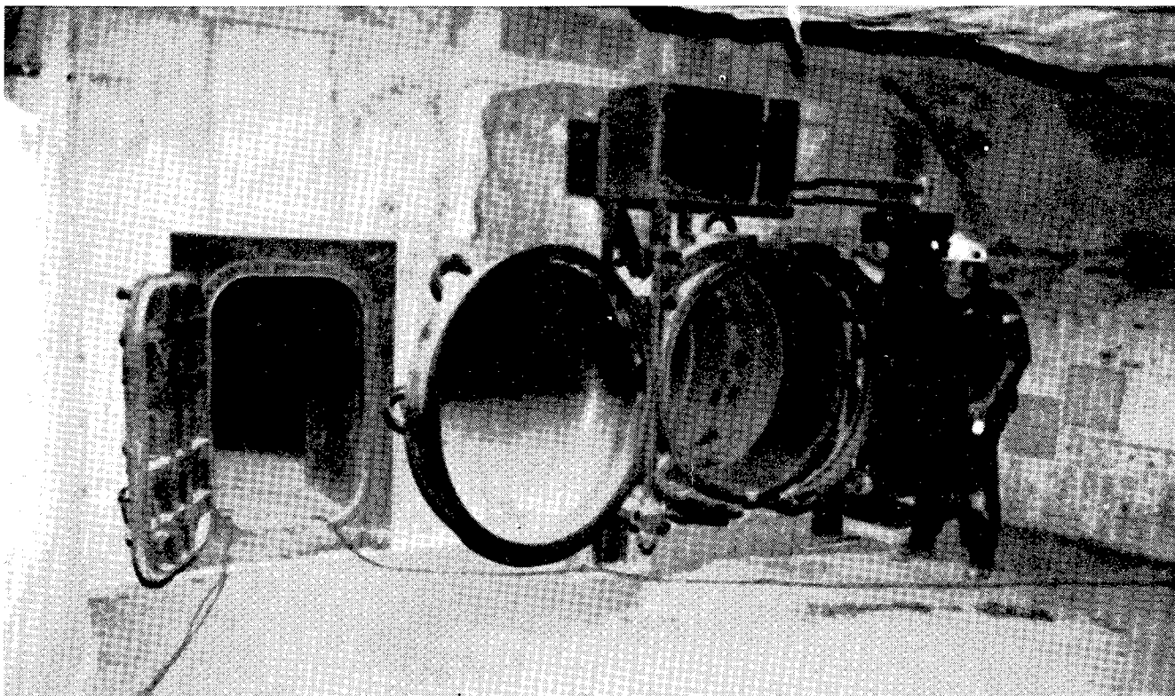
FIGURE 23. - Remote-controlled circular ventilation door is on the right. A marine explosion-proof door is on the left.
