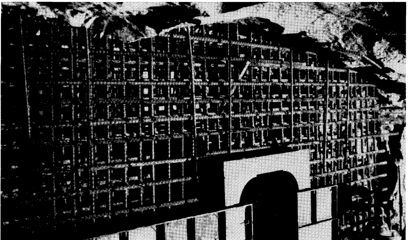
FIGURE A-19. - Reinforcement rods prior to pouring of concrete to construct bulkhead for an underground instrument room.
