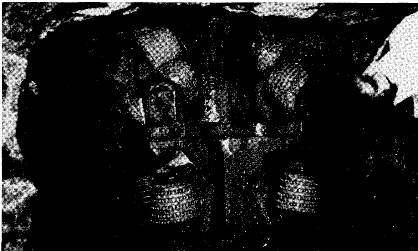
FIGURE A-14. - Five-foot-diameter rock drill used to bore the vertical borehole for the ventilation duct. Raise drilling method was used.
