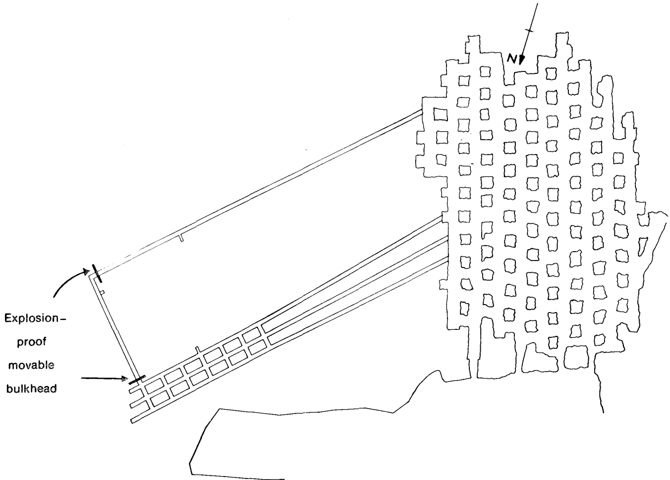
FIGURE 10. - Explosionproof bulkhead location.
