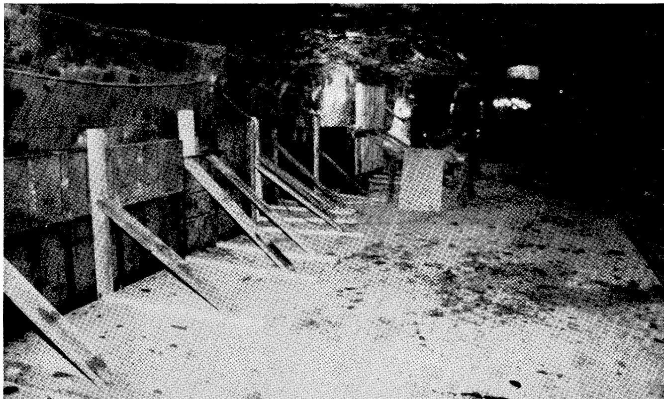
FIGURE A-20. - Forms to hold wet concrete for fender to protect instrumentation and utility, power, air, and water lines.
