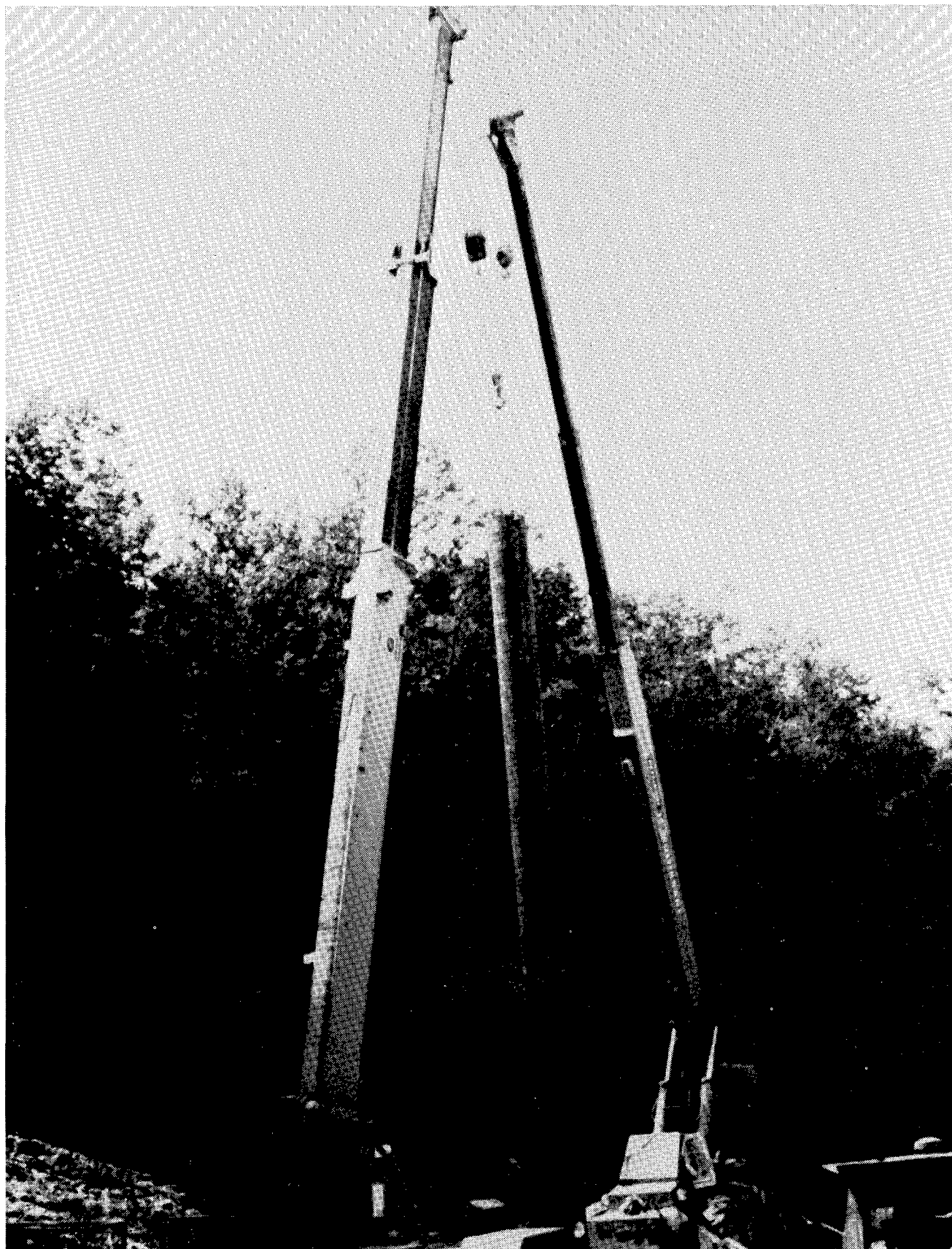
FIGURE A-13. - Two cranes lowering a 2-ft casing into a vertical borehole.
