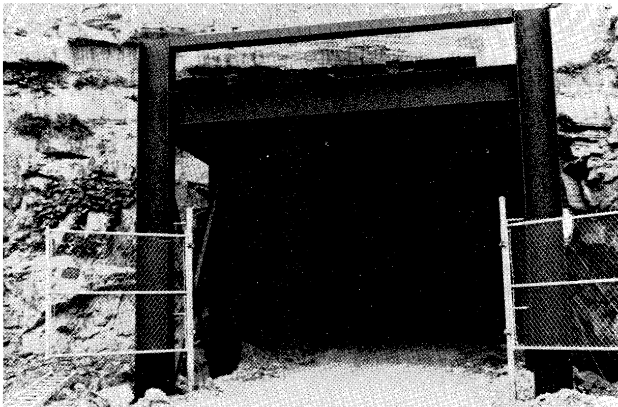
FIGURE 6. - Portal canopy illustration as built.
