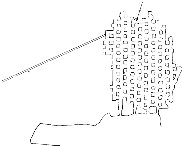
FIGURE 18. - Single-entry configuration.
