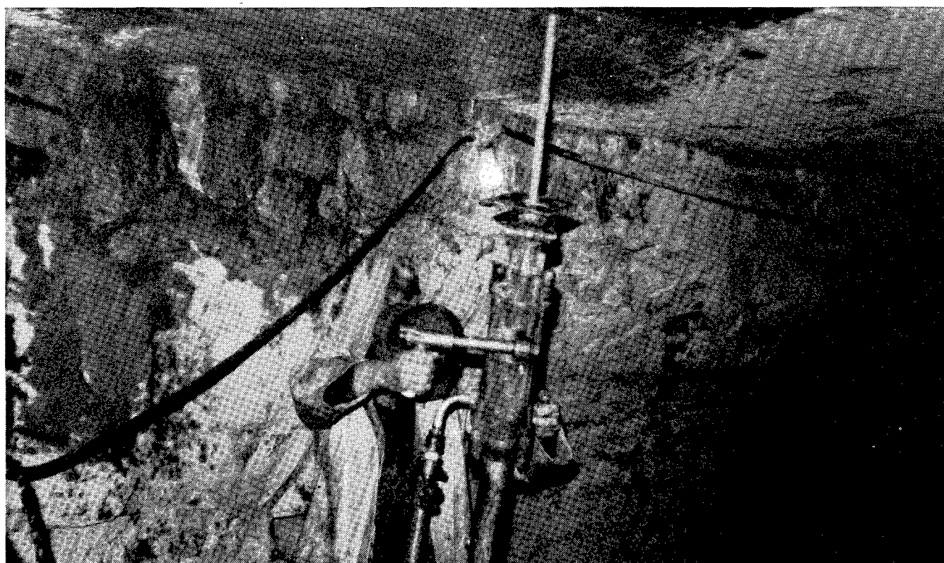
FIGURE A-17. - Installation of 4-ft roof bolt in a drift.
