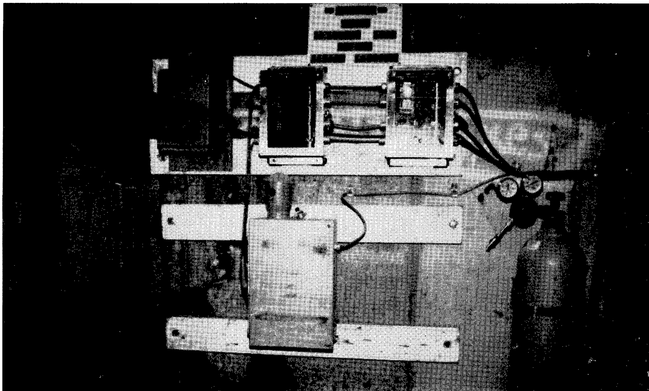
FIGURE 29. - Shotfiring panel.
