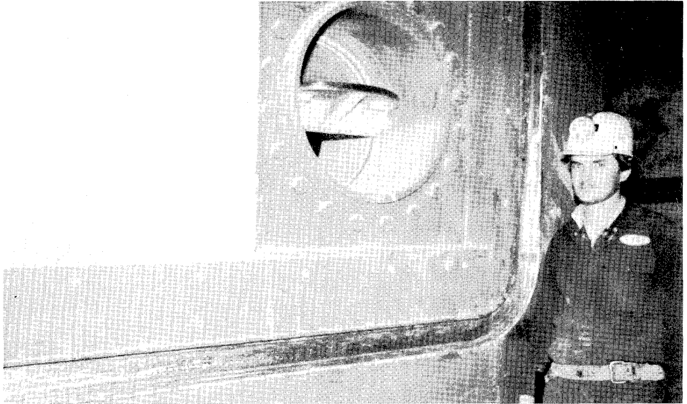
FIGURE 16. - Remote-controlled 24-in butterfly valve installed in movable bulkhead.
