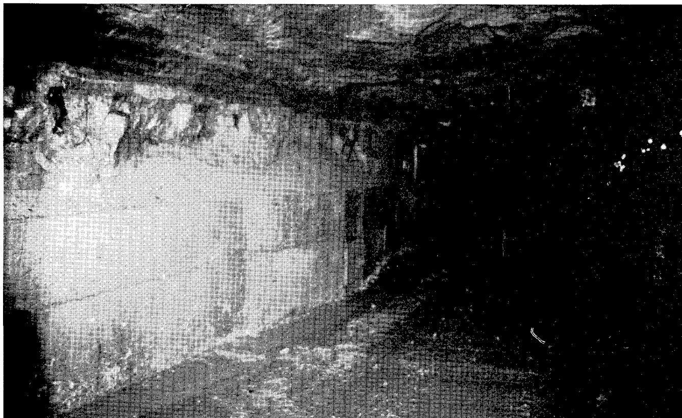
FIGURE 35. - View of a completed drift showing concrete floor and rib with concrete fender.
