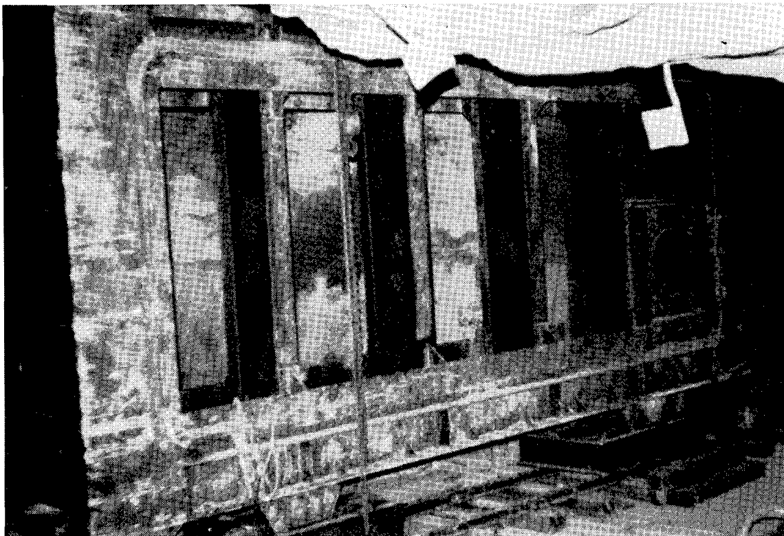
FIGURE 12. - Movable bulkhead before installation of reinforcing rods and pouring of concrete.
