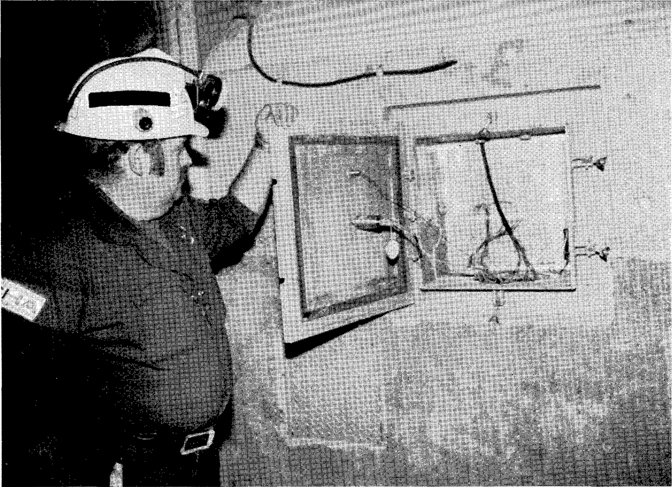
FIGURE 26. - DG panel with completed concrete.
