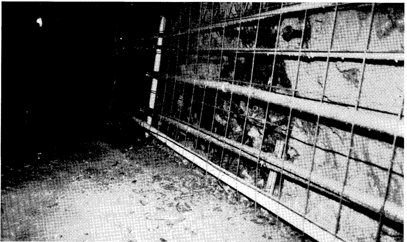
FIGURE 34. - Forming and reinforcement for the concrete fenders underground; these fenders encase the air and water lines and the power, communication, and instrument cables.
