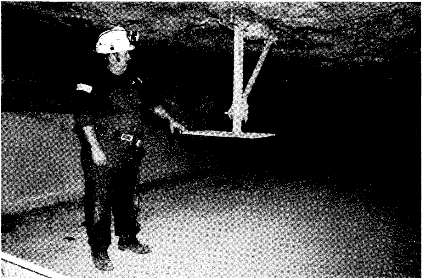
FIGURE 28. - Instrument platform that retracts into the roof of the entries—there are 38 such platforms installed in the facility.
