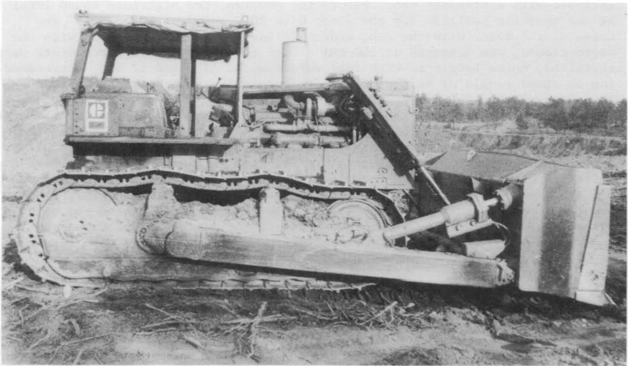
FIGURE 1. - Caterpillar D9G bulldozer with rollover protective structure.
