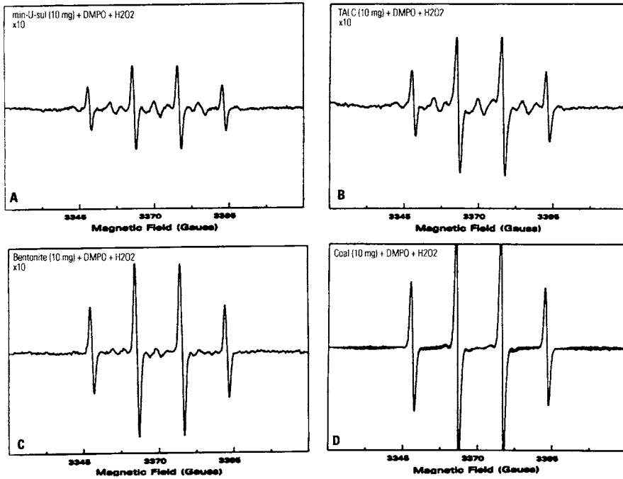
Figure 1. Typical ESR spectra obtained from (A) 10 mg crystalline silica; (B), 10 mg talc; (C), 10 mg bentonite; (D), and 10 mg coal; with 10 mM H 2 O 2 in the presence of 0.1 M DMPO. Note the gain used for the 10-mg coal sample, which produced a signal 18-fold stronger than the bentonite generating the maximal •OH radical generation on an equal mass basis.
