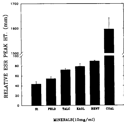
Figure 2. Bar graph illustrating the relative intensities of DMPO-OH adduct signals generated by reacting 10 mg/ml minerals with 10 mM H 2 O 2 in the presence of 100 mM DMPO as a spin trap. Note that the coal generated signals 18-fold greater than the bentonite.
