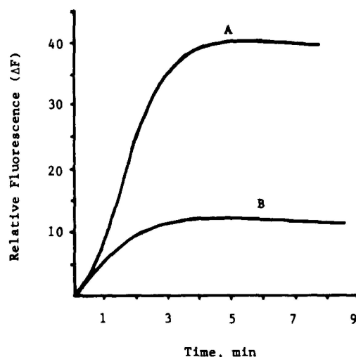
Fig. 9. Fluorescence change ( \Delta F ) as a function of time upon addition of 0.25 \mu g/ml phospholipase A 2 to solutions containing 1 \times 10^{-5} M DPPC, 5 \times 10^{-5} M ANS, 6 \times 10^{-3} M Ca 2+ , and in the absence (A) and presence of 6 \times 10^{-3} M chlorphentermine (B). Drug inhibition of enzyme activities is indicated by the reduction of fluorescence enhancement.
