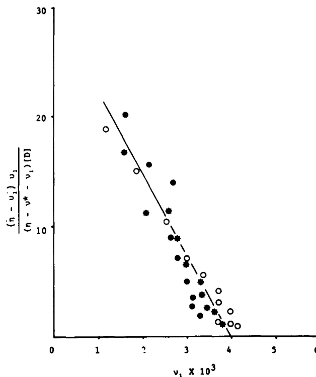
Fig. 5. Binding of chlorphentermine to DPPC measured by using DPH as a probe (equation 2). Data were obtained from solutions containing 2 \times 10^{-5} \text{ M} DPPC, varying concentrations of chlorphentermine and (●) 5 \times 10^{-7} \text{ M} DPH; (*) 8 \times 10^{-7} \text{ M} DPH; and (○) 2 \times 10^{-6} \text{ M} DPH.
