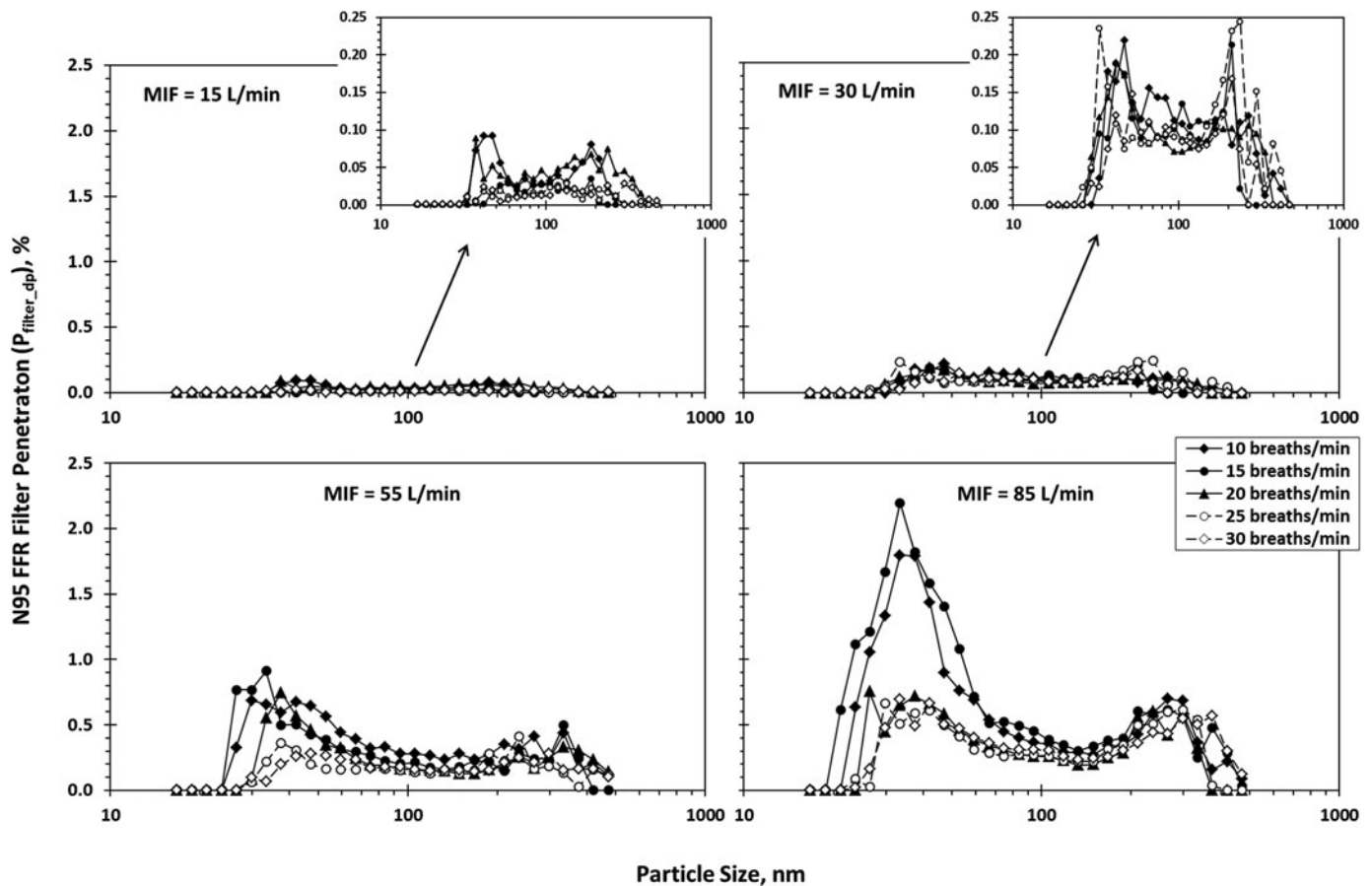
FIG. 1. Size-specific filter penetration for an N95 FFR sealed to a plastic manikin's face while challenged with charge-equilibrated NaCl particles. Each point represents the mean value of three replicates. Calculated coefficient of variation (CV) has a mean of 0.42 and a standard deviation of 0.31.
