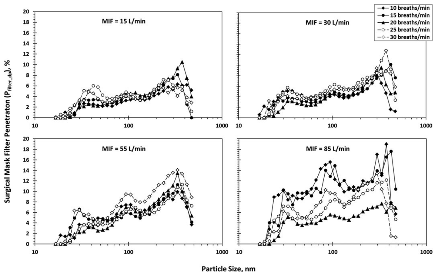
FIG. 3. Size-specific filter penetration for a surgical mask sealed to a plastic manikin's face while challenged with charge-equilibrated NaCl particles. Each point represents the mean value of three replicates. Calculated coefficient of variation (CV) has a mean of 0.45 and a standard deviation of 0.29.
