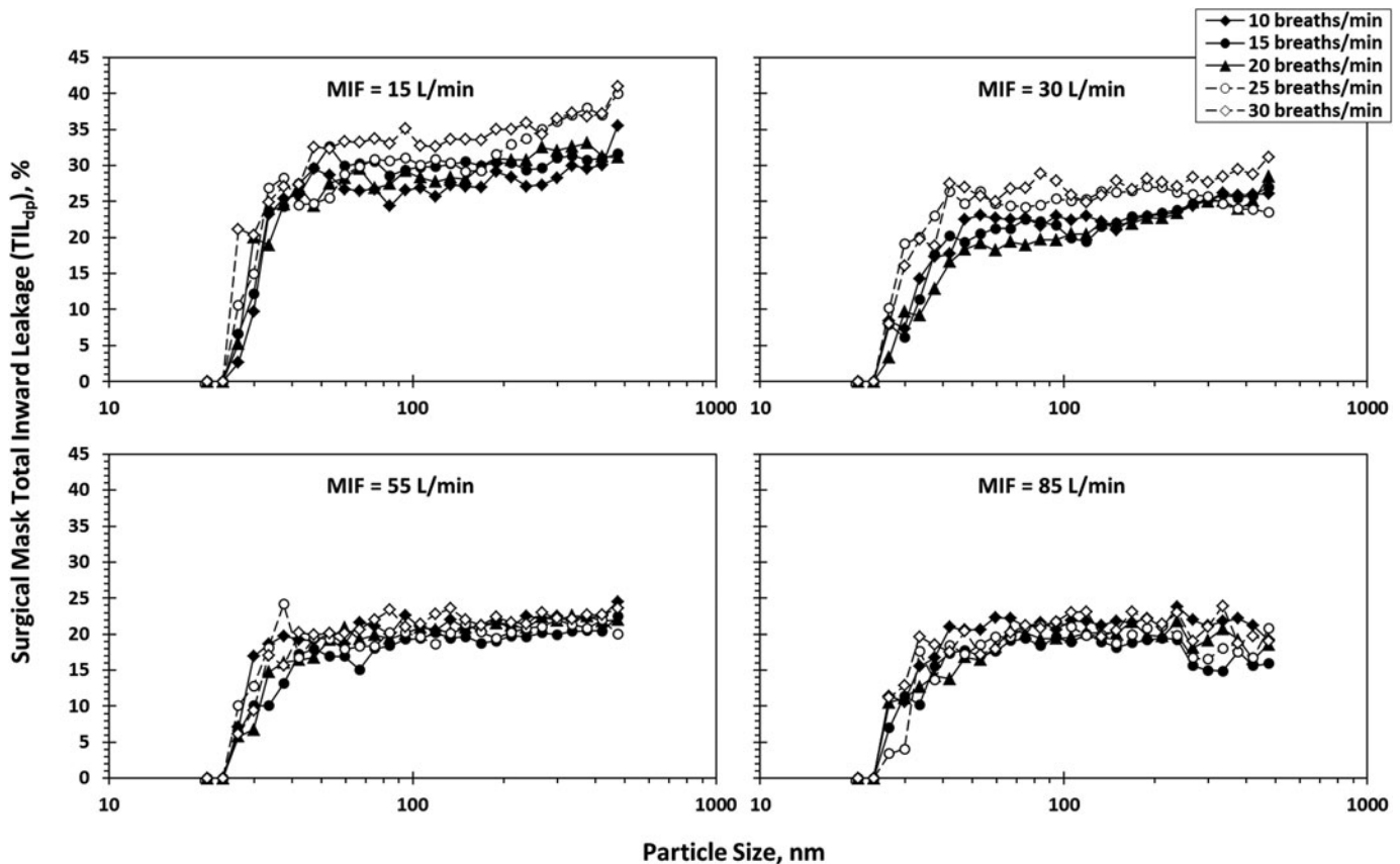
FIG. 4. Size-specific total inward leakage for a surgical mask donned on an advanced manikin headform while challenged with charge-equilibrated NaCl particles. Each point represents the mean value of three replicates. Calculated coefficient of variation (CV) has a mean of 0.18 and a standard deviation of 0.17.
