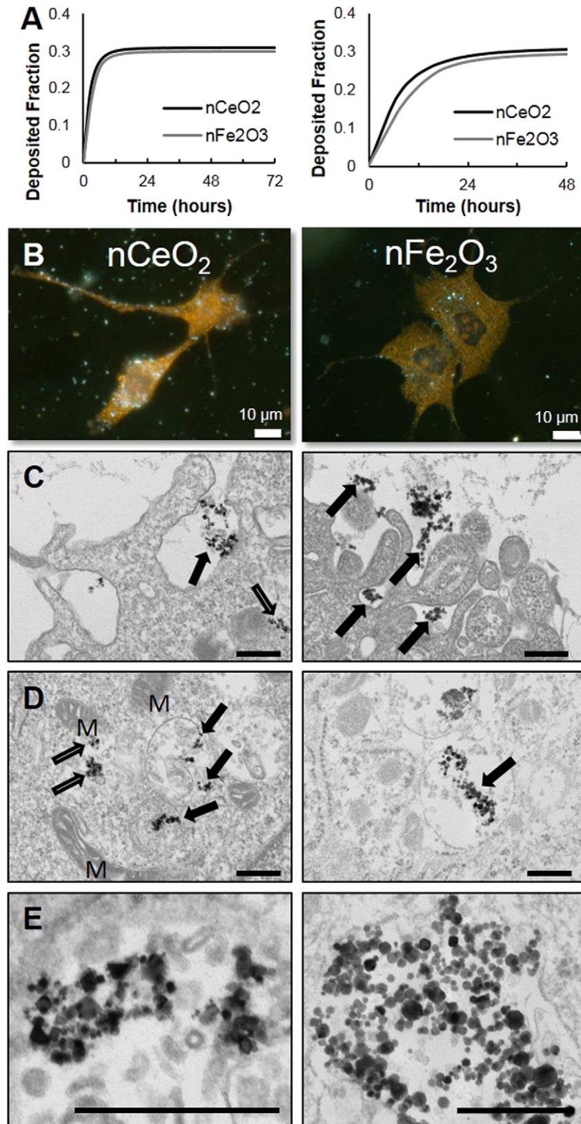
Fig. 1. Dosimetry modeling, cellular fate, and co-localization of nCeO 2 and nFe 2 O 3 particles via enhanced darkfield and transmission electron microscopy following exposure in primary human small airway epithelial cells. A) Harvard distorted grid modeling of sub-chronic exposure in 6-well plates (left) and acute exposure in 96-well plates (right). B) Cells plated on medium-conditioned glass slides were exposed for 48 h in 24-well plates to nCeO 2 (left) and nFe 2 O 3 (right; 0.017 μg/cm 2 deposited). Both nanometal oxides were found co-localized in cytoplasm. Bars = 10 μm. C) Following 24 h exposure to 0.18 μg/cm 2 , both nCeO 2 and nFe 2 O 3 were observed to undergo internalization via phagocytosis (black arrows) and the cell membrane periphery. D) nCeO 2 was observed both in the cytoplasm (white arrows) and enclosed in membrane-bound vesicles (black arrows). nFe 2 O 3 particles were exclusively found in membrane-bound vesicles. 'M' signifies mitochondria. E) Both NMO were found as loose agglomerates within exposed cells. Bars = 400 nm.
