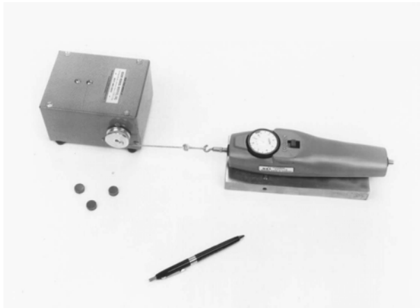
FIGURE 12.9 Horizontal pull slipmeter (HPS). (From Chang, W.R. et al., Ergonomics , 44, 1233–1261, 2001.)
